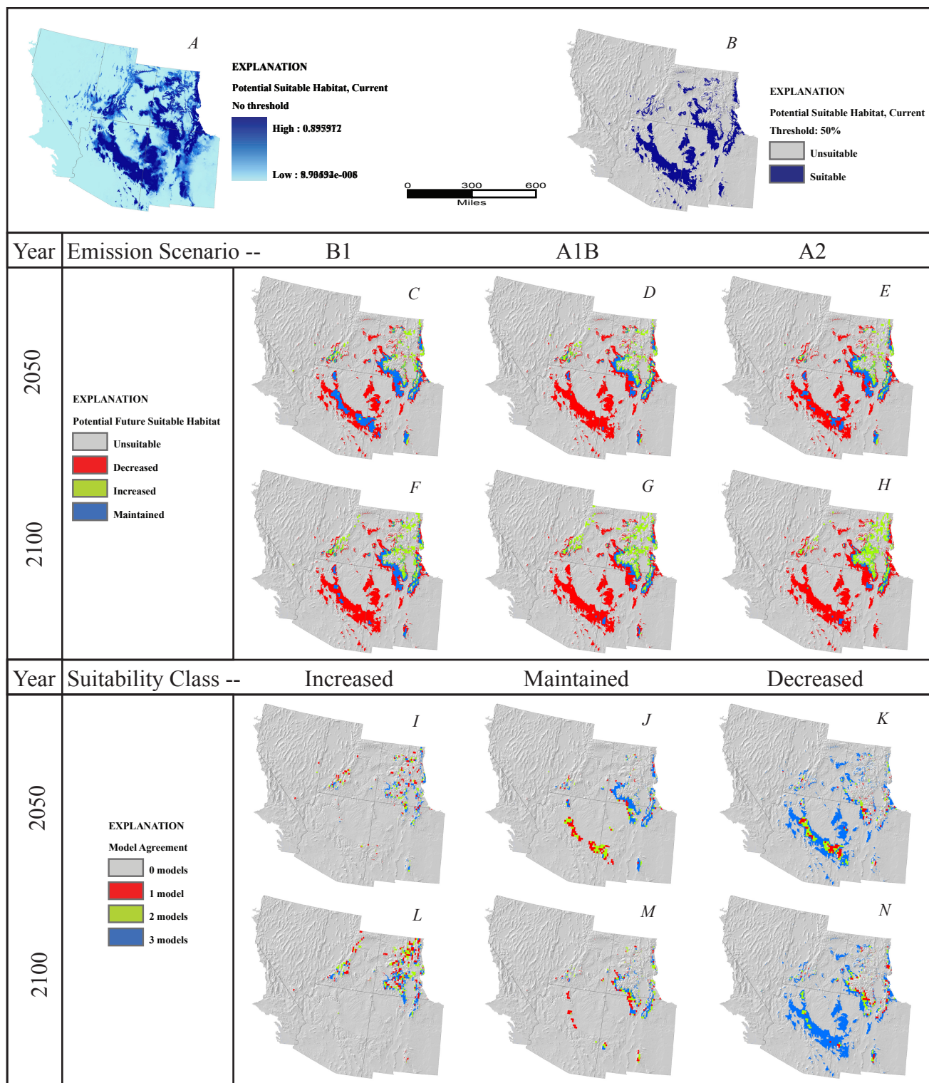
Figure 24. Pinus ponderosa . A, Potential suitable habitat for species based on average annual and monthly precipitation and temperature from 1971 to 2000, continuous model output with no threshold. B, Potential suitable habitat, binary output using .5 threshold. C-E, Potential suitable habitat predicted by year 2050 under emission scenario (C), B1, (D), A1B, (E), A2. F-H, Potential suitable habitat predicted by year 2100 under emission scenario (F), B1, (G), A1B, (H), A2. I-K, Number of 2050 emission scenario models predicting each suitability class, (I), increased suitability, (J), maintained suitability, (K), decreased suitability. L-N, Number of 2100 emission scenario models predicting each suitability class, (L), increased suitability, (M), maintained suitability, and (N), decreased suitability.
