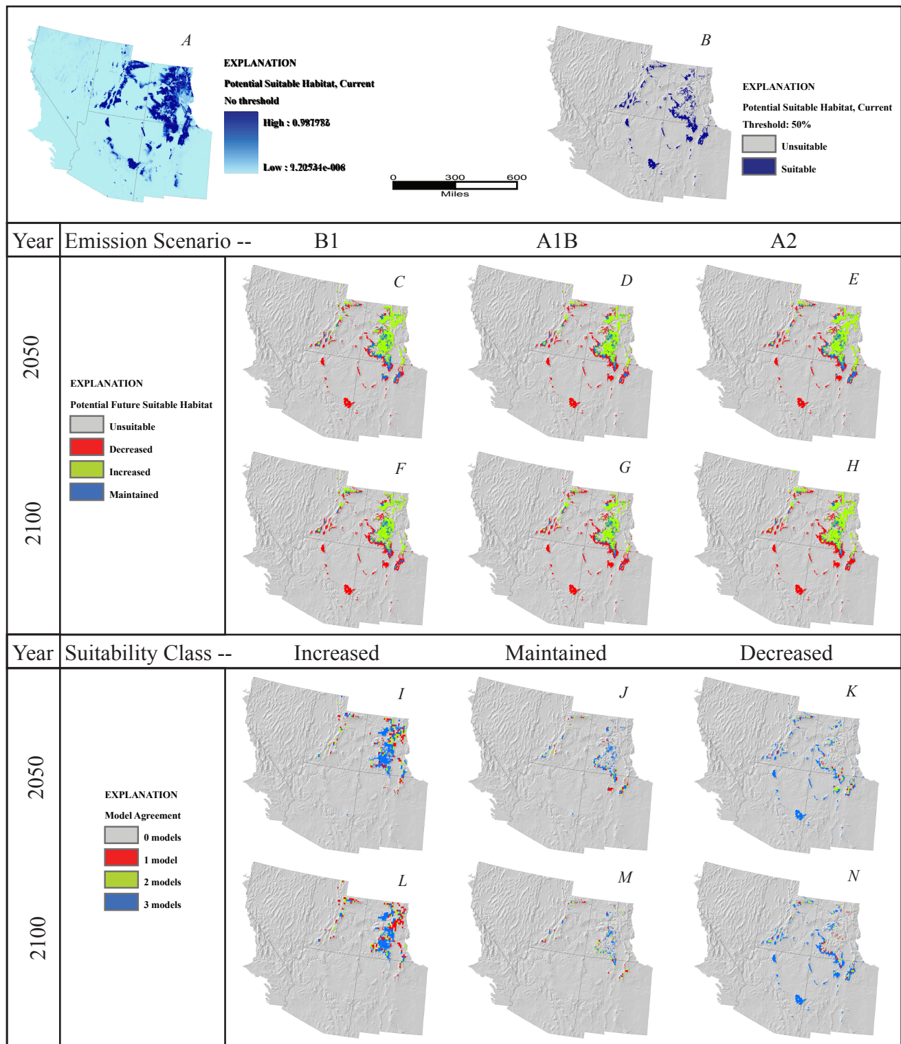
Figure 18. Picea pungens . A, Potential suitable habitat for species based on average annual and monthly precipitation and temperature from 1971 to 2000, continuous model output with no threshold. B, Potential suitable habitat, binary output using .5 threshold. C-E, Potential suitable habitat predicted by year 2050 under emission scenario (C), B1, (D), A1B, (E), A2. F-H, Potential suitable habitat predicted by year 2100 under emission scenario (F), B1, (G), A1B, (H), A2. I-K, Number of 2050 emission scenario models predicting each suitability class, (I), increased suitability, (J), maintained suitability, (K), decreased suitability. L-N, Number of 2100 emission scenario models predicting each suitability class, (L), increased suitability, (M), maintained suitability, and (N), decreased suitability.
