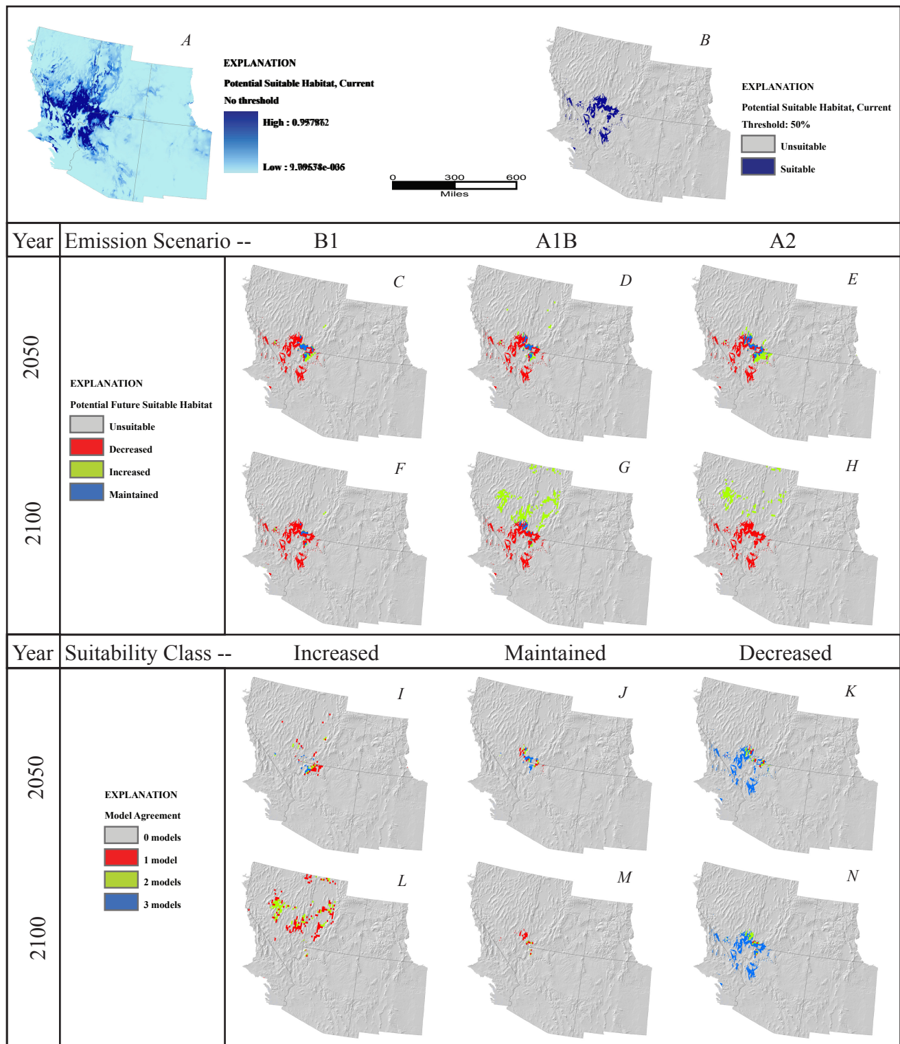
Figure 102. Prunus fasciculata . A, Potential suitable habitat for species based on average annual and monthly precipitation and temperature from 1971 to 2000, continuous model output with no threshold. B, Potential suitable habitat, binary output using .5 threshold. C-E, Potential suitable habitat predicted by year 2050 under emission scenario (C), B1, (D), A1B, (E), A2. F-H, Potential suitable habitat predicted by year 2100 under emission scenario (F), B1, (G), A1B, (H), A2. I-K, Number of 2050 emission scenario models predicting each suitability class, (I), increased suitability, (J), maintained suitability, (K), decreased suitability. L-N, Number of 2100 emission scenario models predicting each suitability class, (L), increased suitability, (M), maintained suitability, and (N), decreased suitability.
