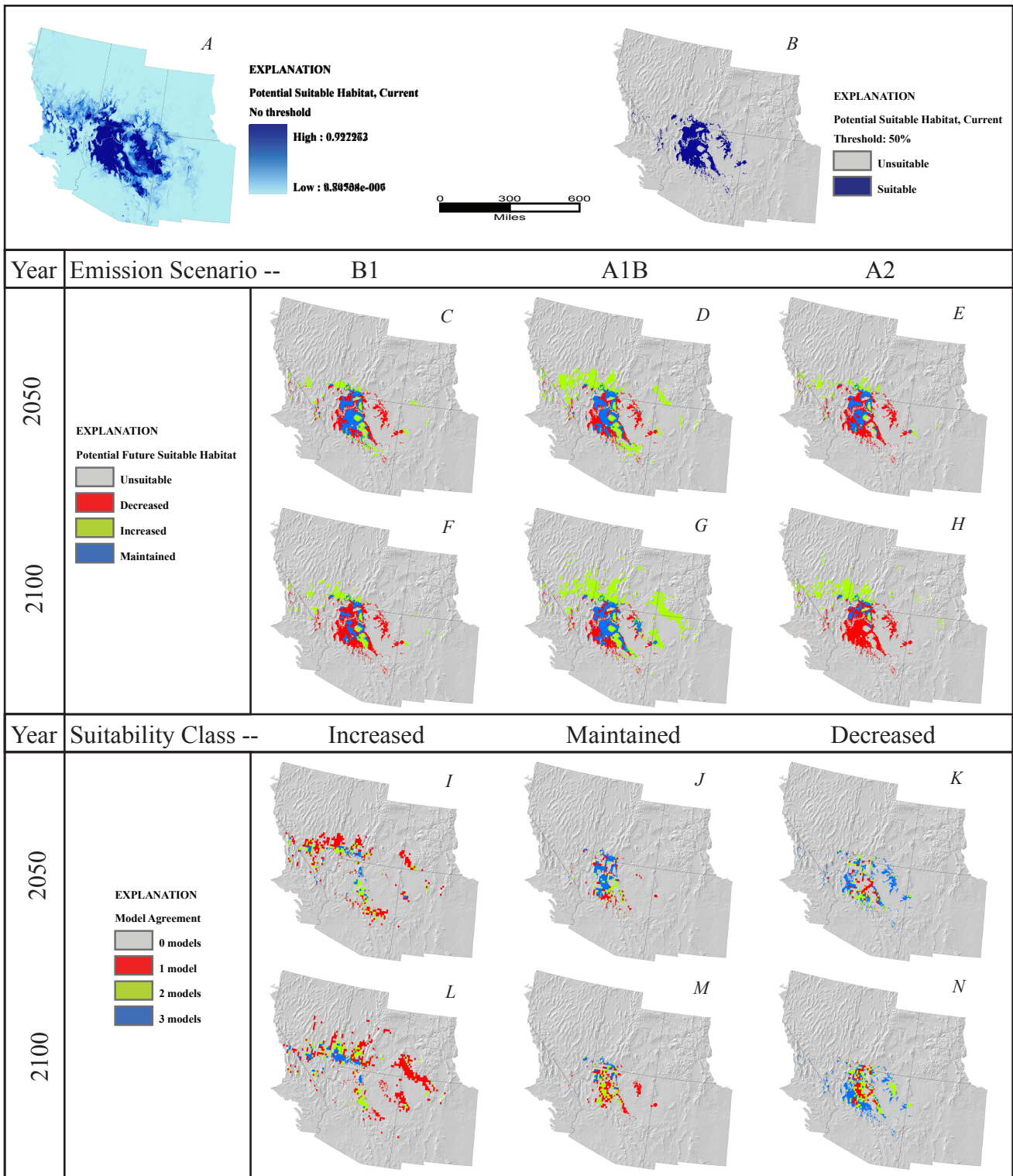
Figure 104. Purshia mexicana . A, Potential suitable habitat for species based on average annual and monthly precipitation and temperature from 1971 to 2000, continuous model output with no threshold. B, Potential suitable habitat, binary output using .5 threshold. C-E, Potential suitable habitat predicted by year 2050 under emission scenario (C), B1, (D), A1B, (E), A2. F-H, Potential suitable habitat predicted by year 2100 under emission scenario (F), B1, (G), A1B, (H), A2. I-K, Number of 2050 emission scenario models predicting each suitability class, (I), increased suitability, (J), maintained suitability, (K), decreased suitability. L-N, Number of 2100 emission scenario models predicting each suitability class, (L), increased suitability, (M), maintained suitability, and (N), decreased suitability.
