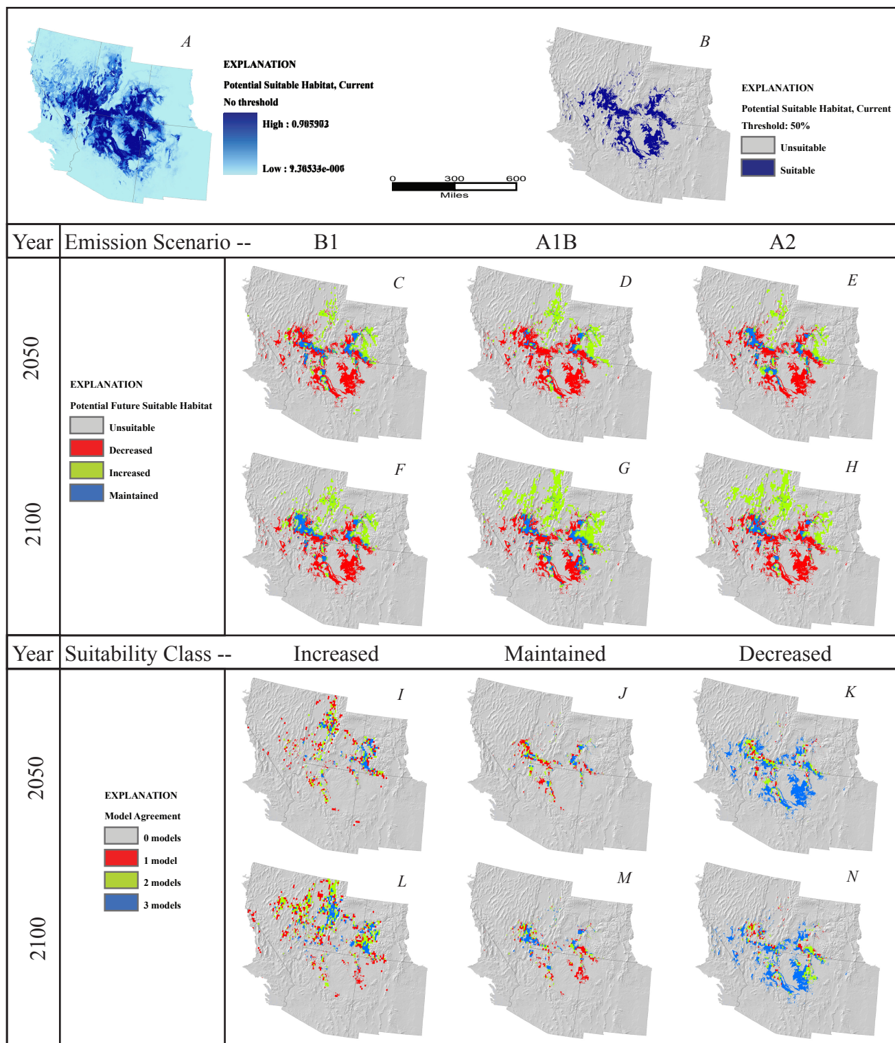
Figure 105. Purshia stansburiana . A, Potential suitable habitat for species based on average annual and monthly precipitation and temperature from 1971 to 2000, continuous model output with no threshold. B, Potential suitable habitat, binary output using .5 threshold. C-E, Potential suitable habitat predicted by year 2050 under emission scenario (C), B1, (D), A1B, (E), A2. F-H, Potential suitable habitat predicted by year 2100 under emission scenario (F), B1, (G), A1B, (H), A2. I-K, Number of 2050 emission scenario models predicting each suitability class, (I), increased suitability, (J), maintained suitability, (K), decreased suitability. L-N, Number of 2100 emission scenario models predicting each suitability class, (L), increased suitability, (M), maintained suitability, and (N), decreased suitability.
