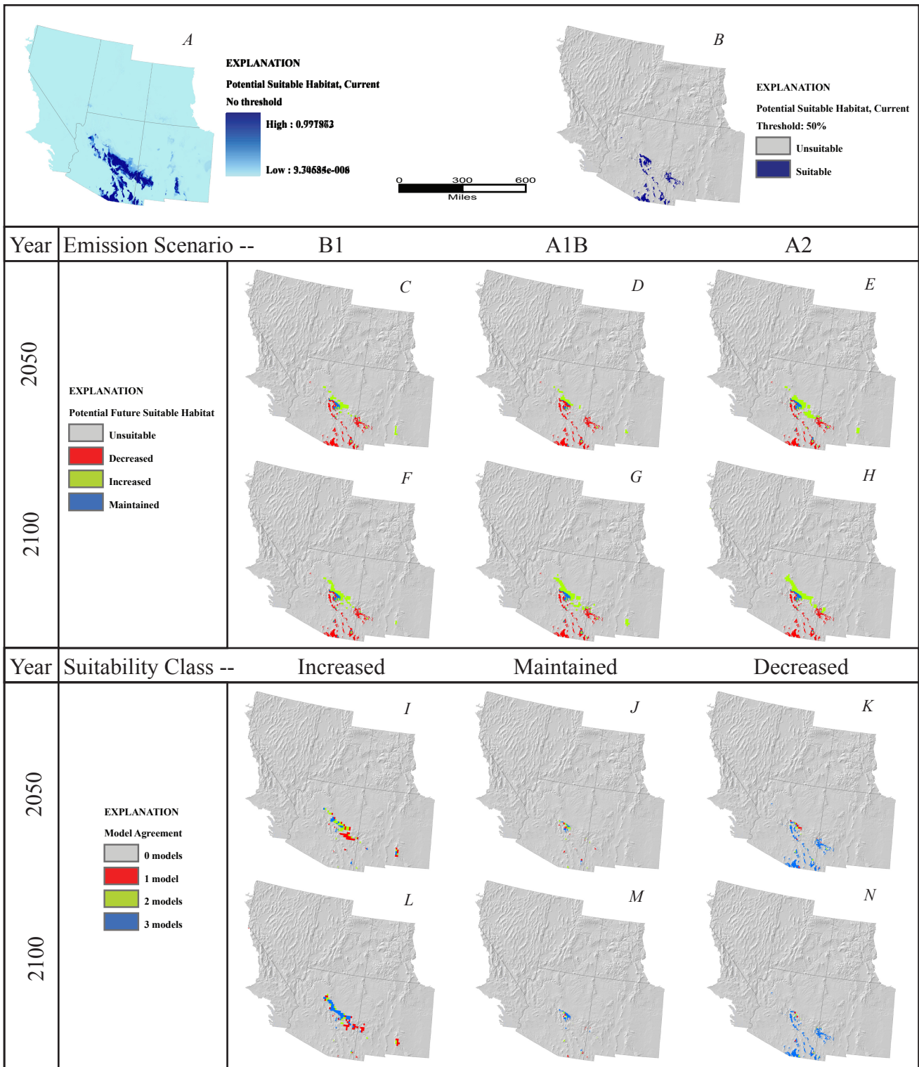
Figure 31. Quercus arizonica . A, Potential suitable habitat for species based on average annual and monthly precipitation and temperature from 1971 to 2000, continuous model output with no threshold. B, Potential suitable habitat, binary output using .5 threshold. C-E, Potential suitable habitat predicted by year 2050 under emission scenario (C), B1, (D), A1B, (E), A2. F-H, Potential suitable habitat predicted by year 2100 under emission scenario (F), B1, (G), A1B, (H), A2. I-K, Number of 2050 emission scenario models predicting each suitability class, (I), increased suitability, (J), maintained suitability, (K), decreased suitability. L-N, Number of 2100 emission scenario models predicting each suitability class, (L), increased suitability, (M), maintained suitability, and (N), decreased suitability.
