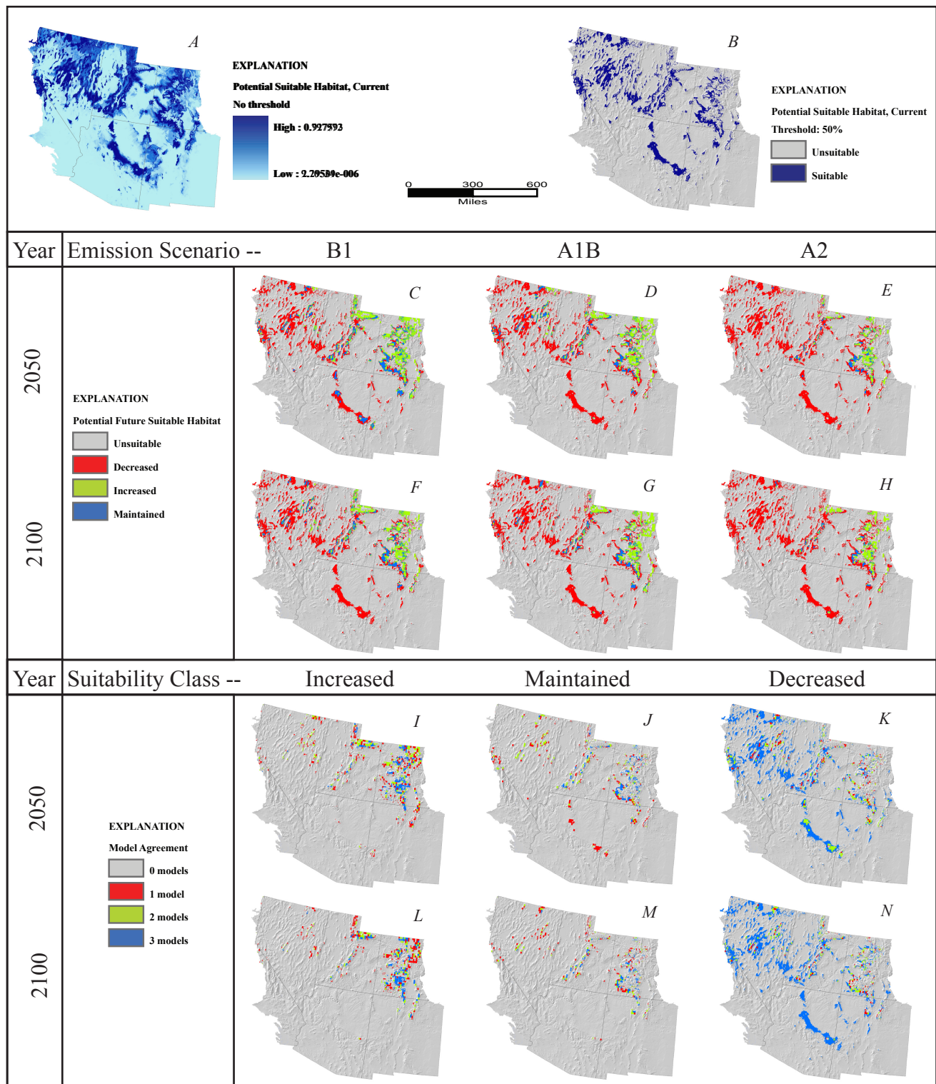
Figure 114. Rosa woodsii . A, Potential suitable habitat for species based on average annual and monthly precipitation and temperature from 1971 to 2000, continuous model output with no threshold. B, Potential suitable habitat, binary output using .5 threshold. C-E, Potential suitable habitat predicted by year 2050 under emission scenario (C), B1, (D), A1B, (E), A2. F-H, Potential suitable habitat predicted by year 2100 under emission scenario (F), B1, (G), A1B, (H), A2. I-K, Number of 2050 emission scenario models predicting each suitability class, (I), increased suitability, (J), maintained suitability, (K), decreased suitability. L-N, Number of 2100 emission scenario models predicting each suitability class, (L), increased suitability, (M), maintained suitability, and (N), decreased suitability.
