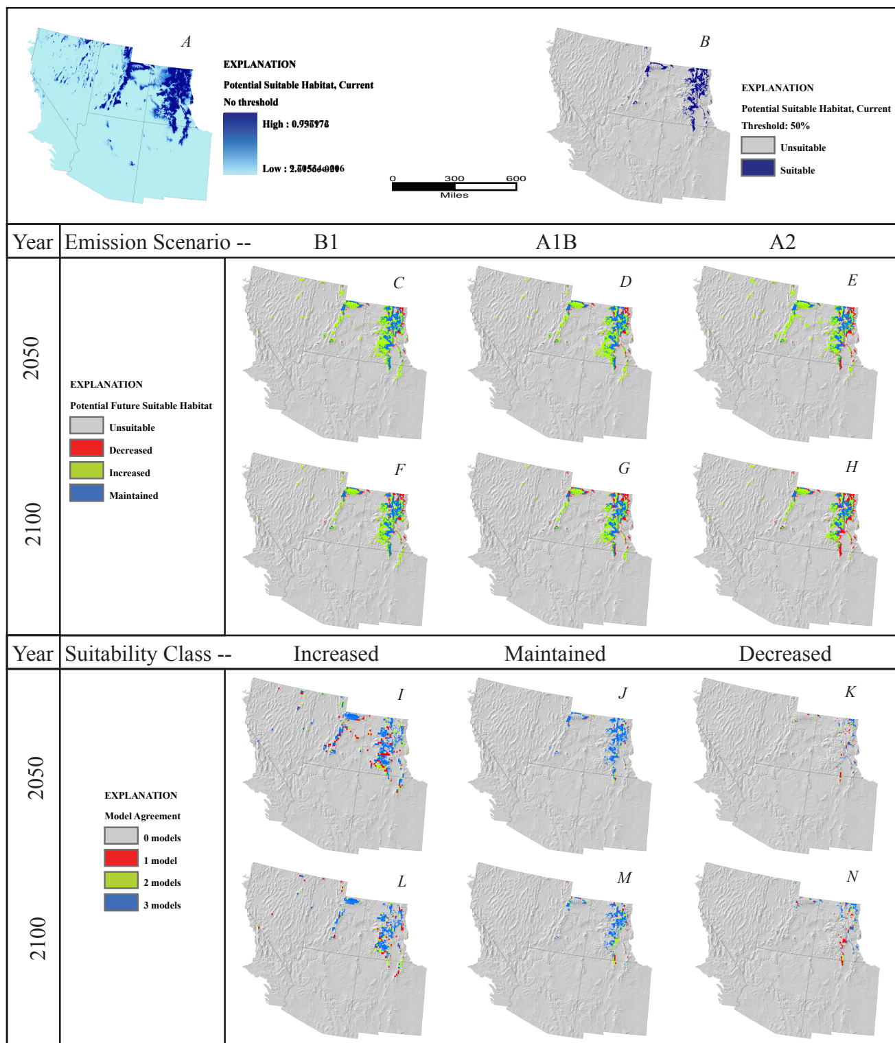
Figure 118. Shepherdia canadensis . A, Potential suitable habitat for species based on average annual and monthly precipitation and temperature from 1971 to 2000, continuous model output with no threshold. B, Potential suitable habitat, binary output using .5 threshold. C-E, Potential suitable habitat predicted by year 2050 under emission scenario (C), B1, (D), A1B, (E), A2. F-H, Potential suitable habitat predicted by year 2100 under emission scenario (F), B1, (G), A1B, (H), A2. I-K, Number of 2050 emission scenario models predicting each suitability class, (I), increased suitability, (J), maintained suitability, (K), decreased suitability. L-N, Number of 2100 emission scenario models predicting each suitability class, (L), increased suitability, (M), maintained suitability, and (N), decreased suitability.
