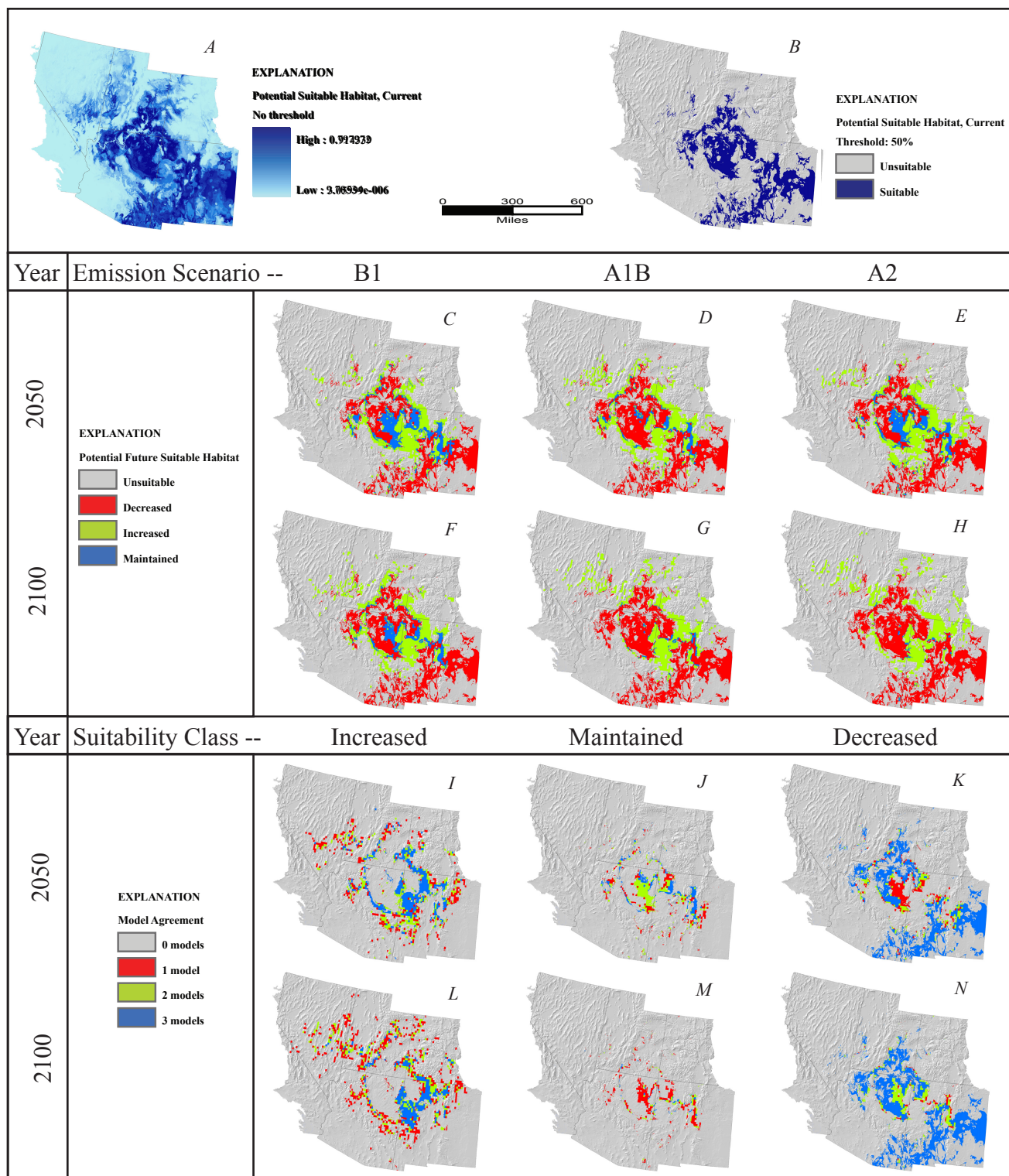
Figure 165. Sporobolus cryptandrus . A, Potential suitable habitat for species based on average annual and monthly precipitation and temperature from 1971 to 2000, continuous model output with no threshold. B, Potential suitable habitat, binary output using .5 threshold. C-E, Potential suitable habitat predicted by year 2050 under emission scenario (C), B1, (D), A1B, (E), A2. F-H, Potential suitable habitat predicted by year 2100 under emission scenario (F), B1, (G), A1B, (H), A2. I-K, Number of 2050 emission scenario models predicting each suitability class, (I), increased suitability, (J), maintained suitability, (K), decreased suitability. L-N, Number of 2100 emission scenario models predicting each suitability class, (L), increased suitability, (M), maintained suitability, and (N), decreased suitability.
