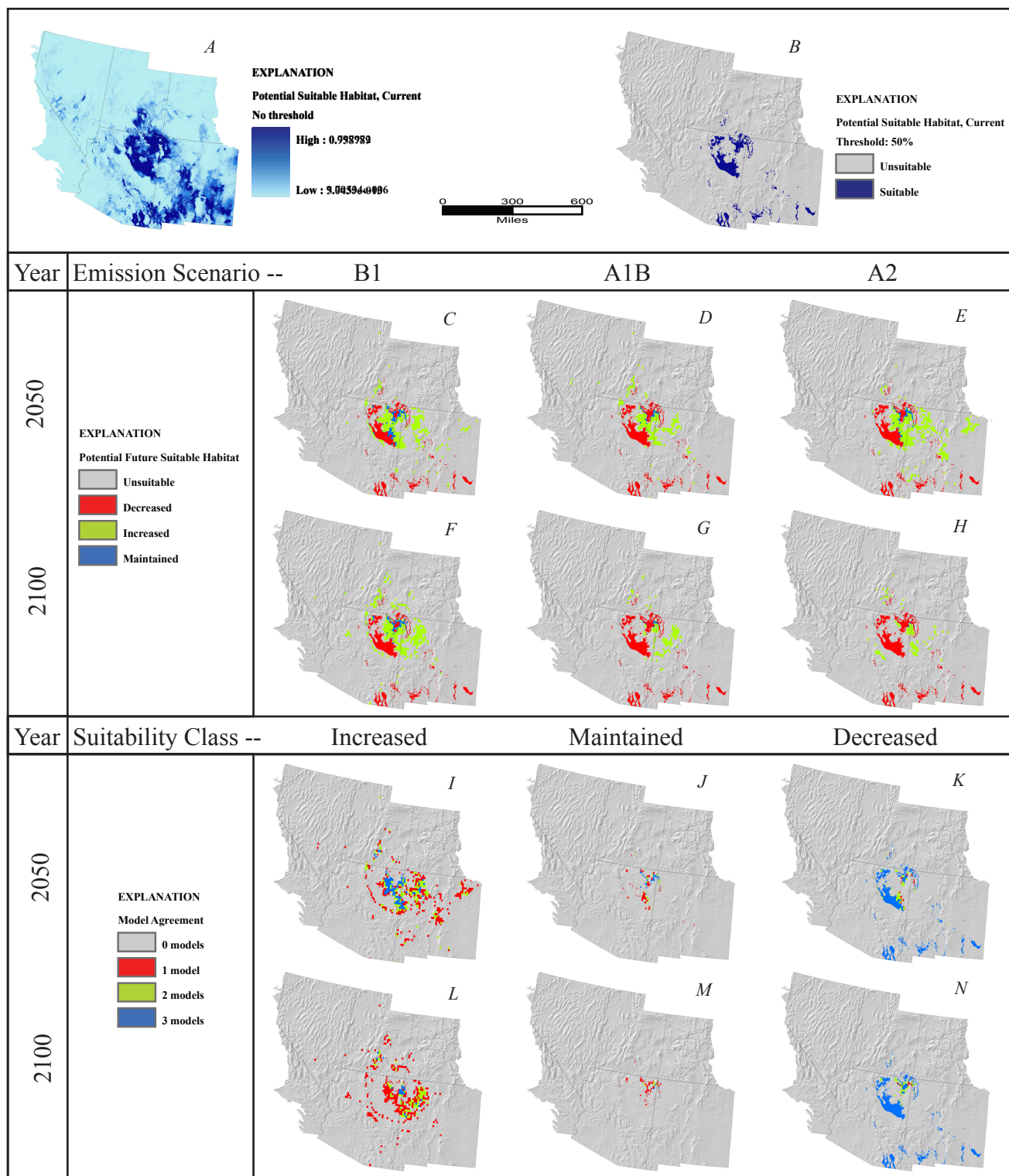
Figure 166. Sporobolus flexuosus . A, Potential suitable habitat for species based on average annual and monthly precipitation and temperature from 1971 to 2000, continuous model output with no threshold. B, Potential suitable habitat, binary output using .5 threshold. C-E, Potential suitable habitat predicted by year 2050 under emission scenario (C), B1, (D), A1B, (E), A2. F-H, Potential suitable habitat predicted by year 2100 under emission scenario (F), B1, (G), A1B, (H), A2. I-K, Number of 2050 emission scenario models predicting each suitability class, (I), increased suitability, (J), maintained suitability, (K), decreased suitability. L-N, Number of 2100 emission scenario models predicting each suitability class, (L), increased suitability, (M), maintained suitability, and (N), decreased suitability.
