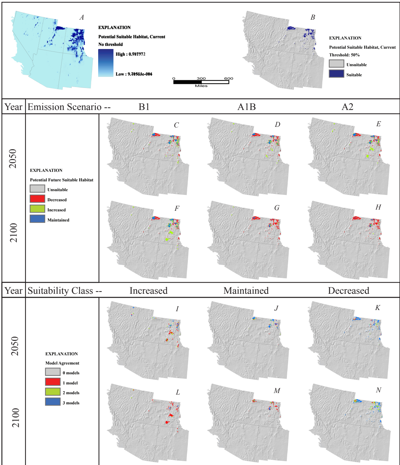
Figure 127. Vaccinium scoparium . A, Potential suitable habitat for species based on average annual and monthly precipitation and temperature from 1971 to 2000, continuous model output with no threshold. B, Potential suitable habitat, binary output using .5 threshold. C-E, Potential suitable habitat predicted by year 2050 under emission scenario (C), B1, (D), A1B, (E), A2. F-H, Potential suitable habitat predicted by year 2100 under emission scenario (F), B1, (G), A1B, (H), A2. I-K, Number of 2050 emission scenario models predicting each suitability class, (I), increased suitability, (J), maintained suitability, (K), decreased suitability. L-N, Number of 2100 emission scenario models predicting each suitability class, (L), increased suitability, (M), maintained suitability, and (N), decreased suitability.
