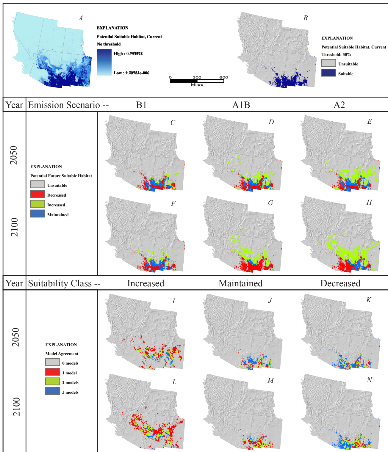
Figure 130. Yucca elata . A, Potential suitable habitat for species based on average annual and monthly precipitation and temperature from 1971 to 2000, continuous model output with no threshold. B, Potential suitable habitat, binary output using .5 threshold. C-E, Potential suitable habitat predicted by year 2050 under emission scenario (C), B1, (D), A1B, (E), A2. F-H, Potential suitable habitat predicted by year 2100 under emission scenario (F), B1, (G), A1B, (H), A2. I-K, Number of 2050 emission scenario models predicting each suitability class, (I), increased suitability, (J), maintained suitability, (K), decreased suitability. L-N, Number of 2100 emission scenario models predicting each suitability class, (L), increased suitability, (M), maintained suitability, and (N), decreased suitability.
