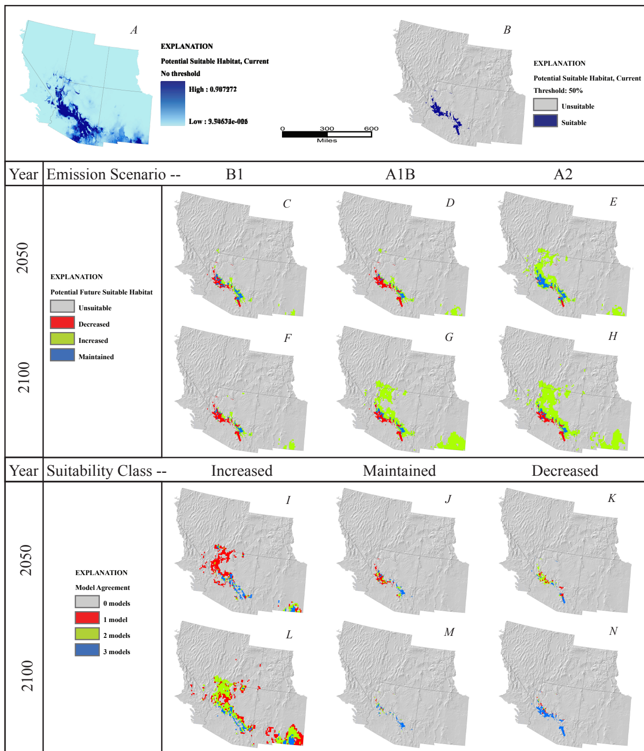
Figure 133. Ziziphus obtusifolia . A, Potential suitable habitat for species based on average annual and monthly precipitation and temperature from 1971 to 2000, continuous model output with no threshold. B, Potential suitable habitat, binary output using .5 threshold. C-E, Potential suitable habitat predicted by year 2050 under emission scenario (C), B1, (D), A1B, (E), A2. F-H, Potential suitable habitat predicted by year 2100 under emission scenario (F), B1, (G), A1B, (H), A2. I-K, Number of 2050 emission scenario models predicting each suitability class, (I), increased suitability, (J), maintained suitability, (K), decreased suitability. L-N, Number of 2100 emission scenario models predicting each suitability class, (L), increased suitability, (M), maintained suitability, and (N), decreased suitability.
