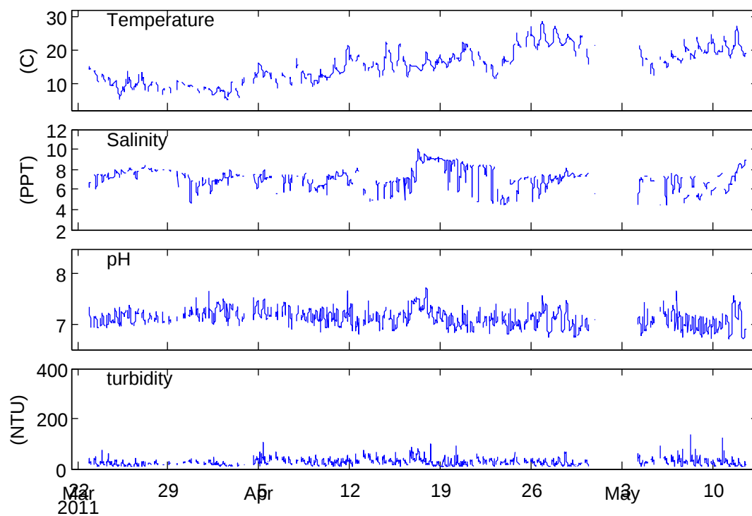
Edge of tidal creek off Transquaking River, Spring 2011 data
