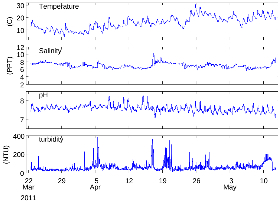
Center of tidal creek off Blackwater River, Spring 2011 data
