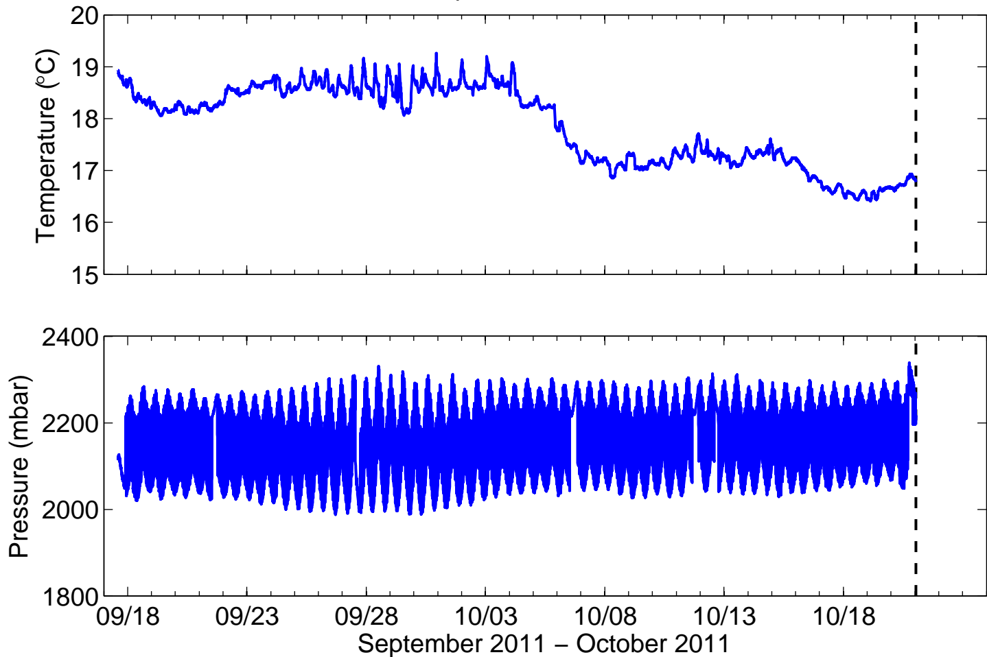
91013 – ADV Temperature and Pressure Time Series
