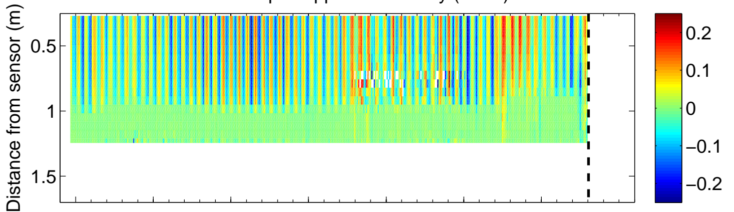
9103 – Aquadopp North Velocity ( \text{m s}^{-1} )
