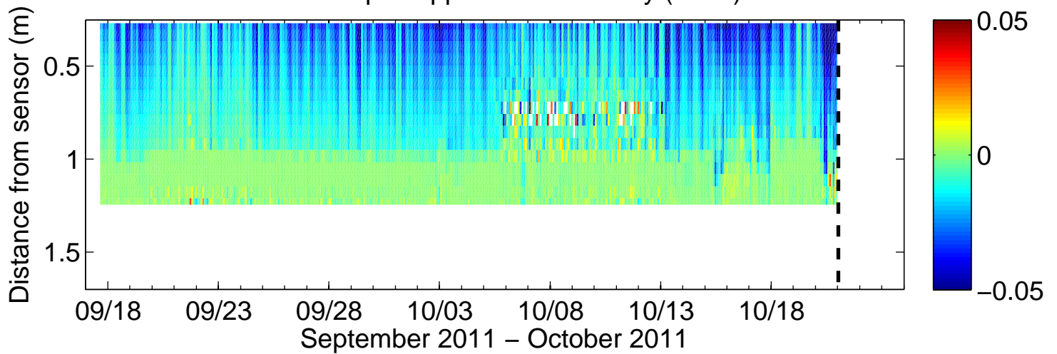
9103 – Aquadopp Vertical Velocity ( \text{m s}^{-1} )
