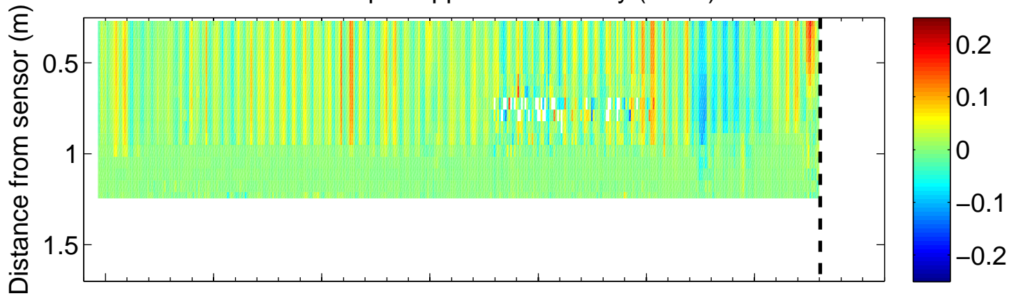
9103 – Aquadopp Vertical Velocity ( \text{m s}^{-1} )
