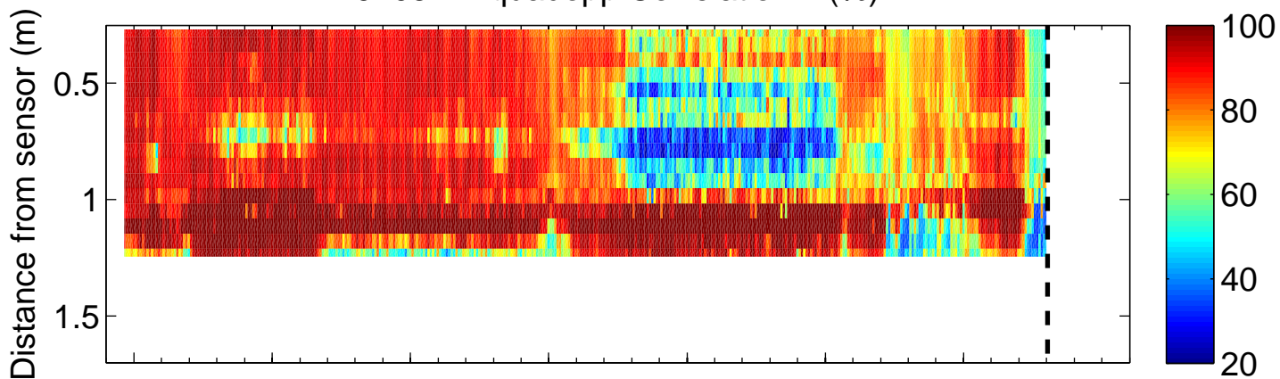
9103 – Aquadopp Correlation 3 (%)
