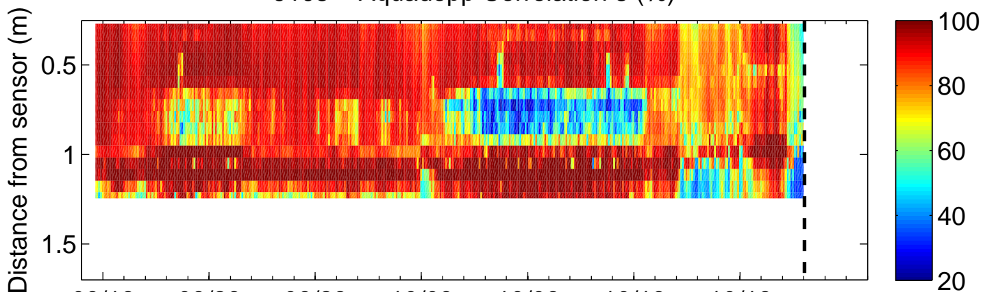
9103 – Aquadopp Correlation 3 (%)
