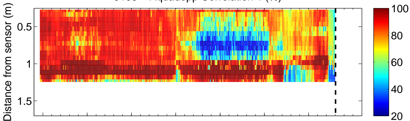
9103 – Aquadopp Correlation 2 (%)
