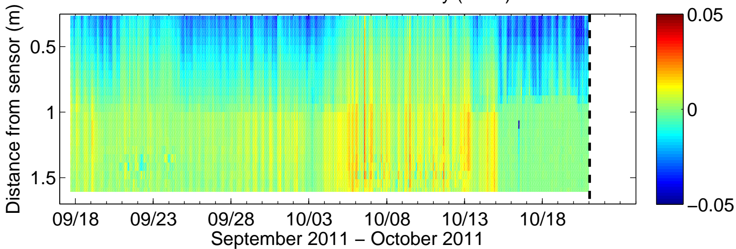
9104 – PCADP Vertical Velocity ( \text{m s}^{-1} )
