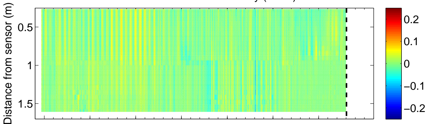
9104 – PCADP Vertical Velocity ( \text{m s}^{-1} )
