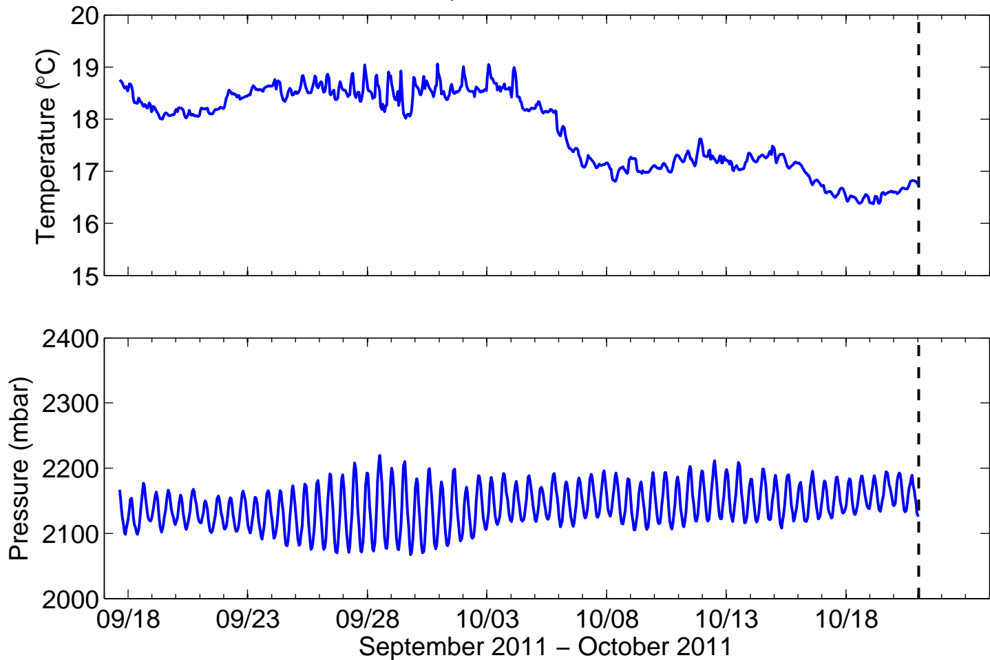
9105 – ADV Temperature and Pressure Time Series
