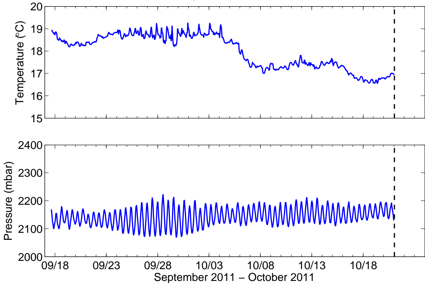
9106 – ADV Temperature and Pressure Time Series
