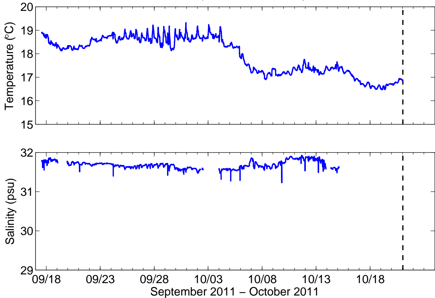
9107 – Seacat Temperature and Salinity Time Series
