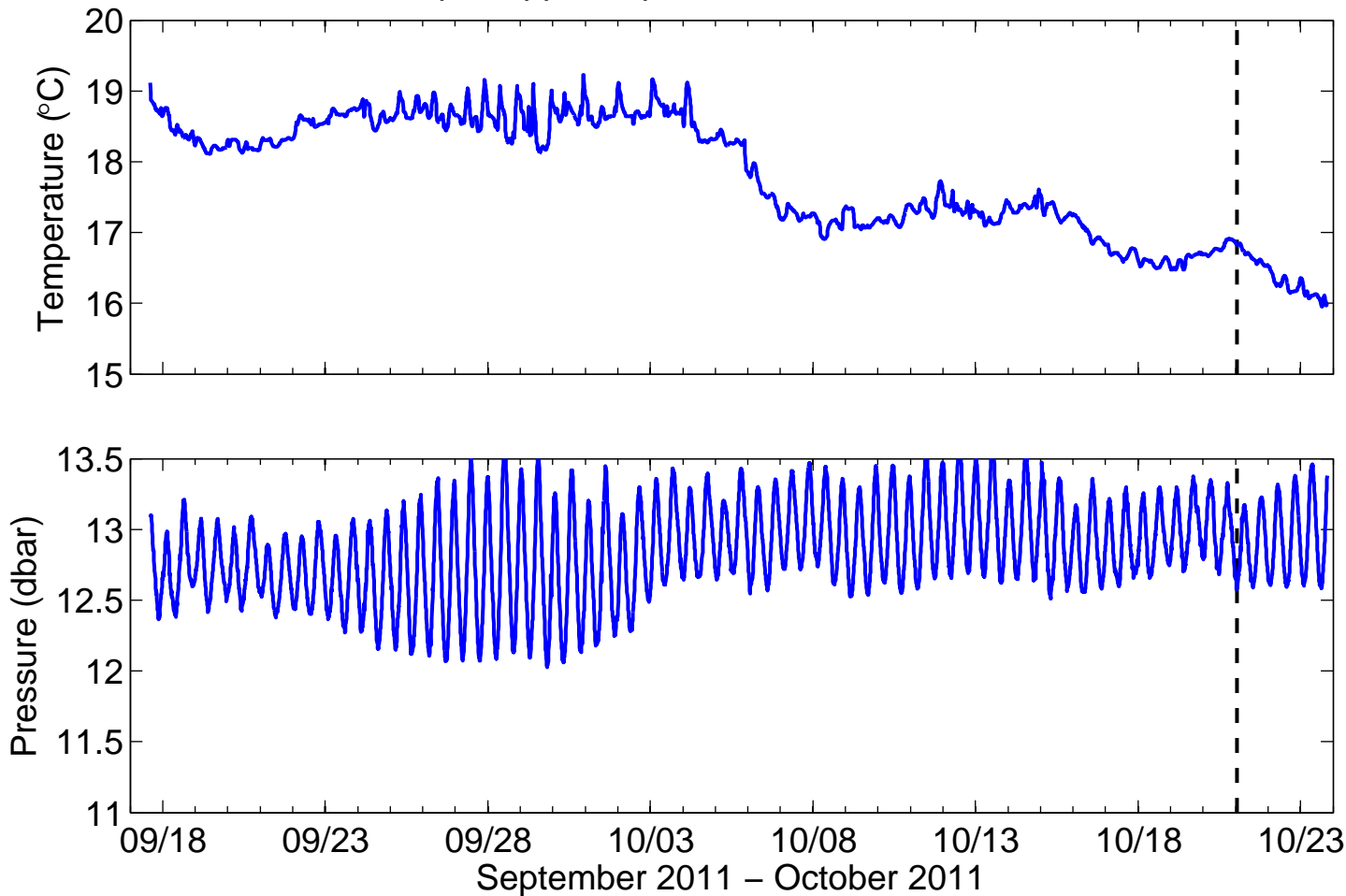
9111 – Aquadopp Temperature and Pressure Time Series
