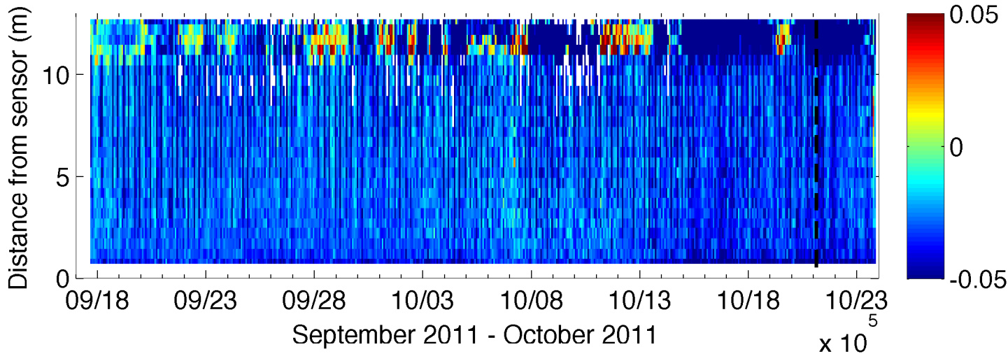
9111 - Aquadopp Vertical Velocity ( \text{m s}^{-1} )
