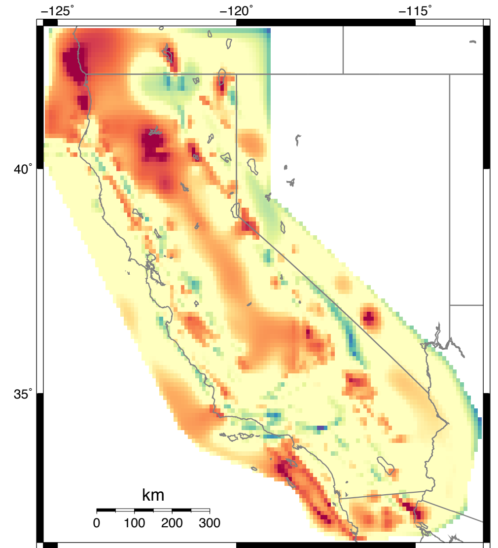
UCERF 3.3 / NSHMP08
