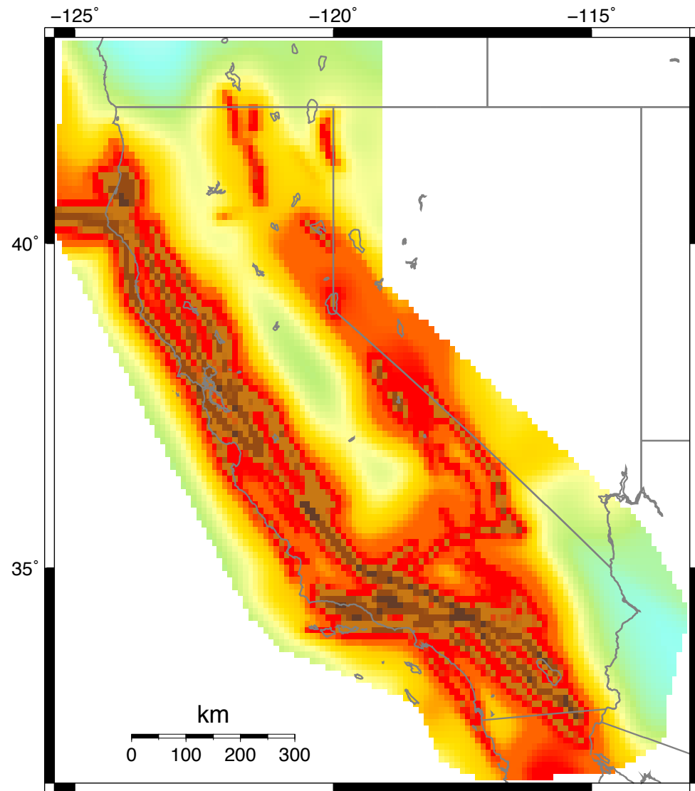
NSHMP08
