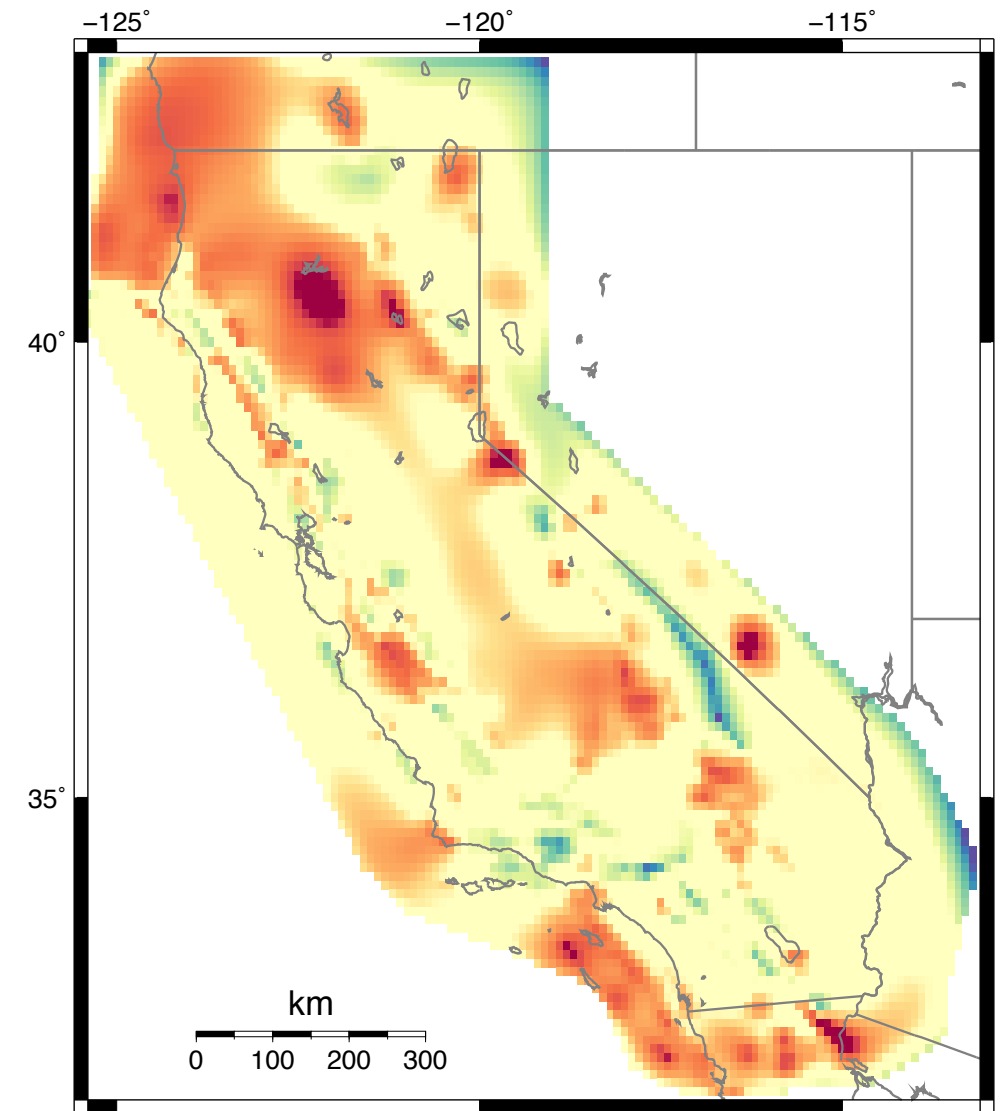
UCERF 3.3 / NSHMP08
