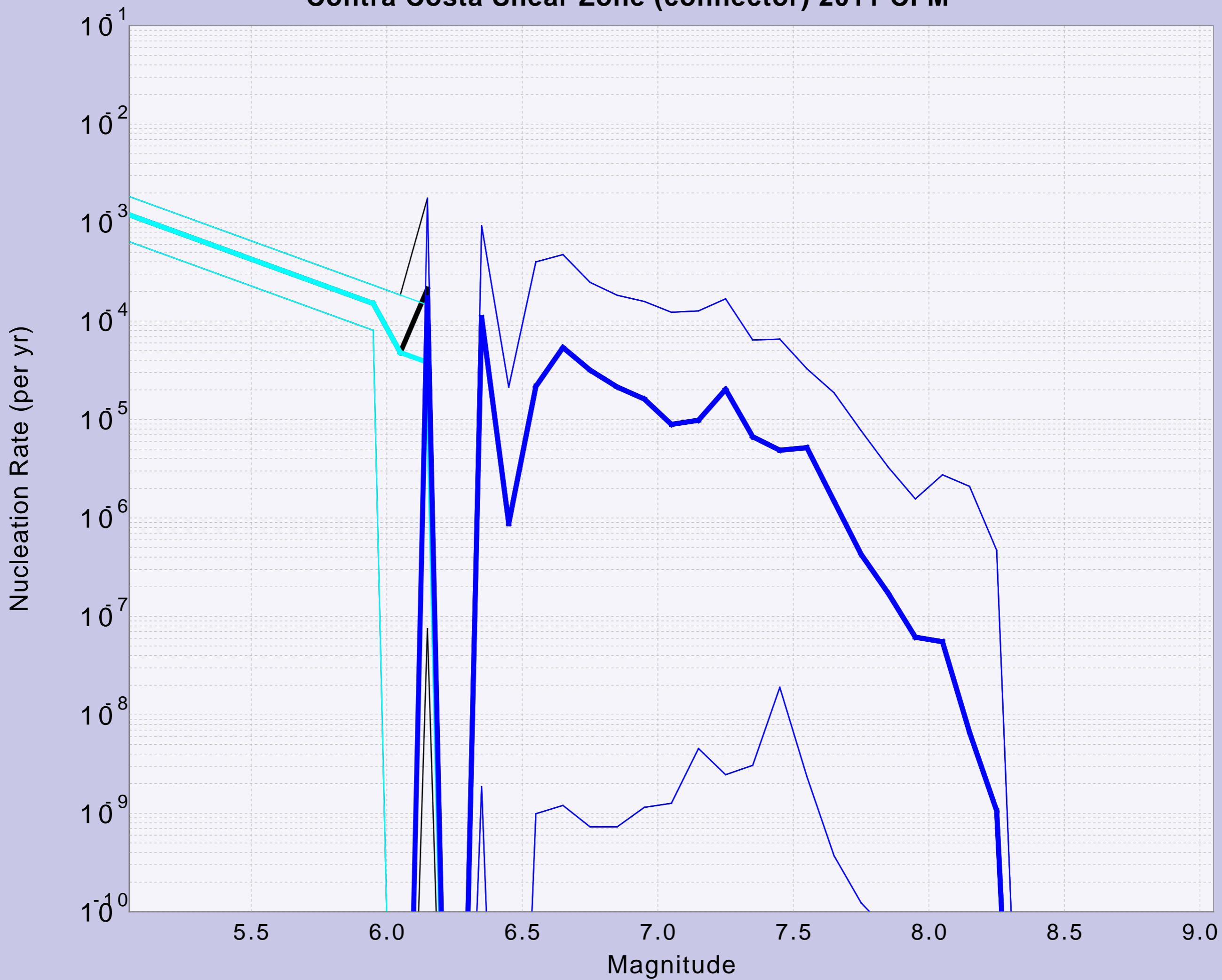
Contra Costa Shear Zone (connector) 2011 CFM
