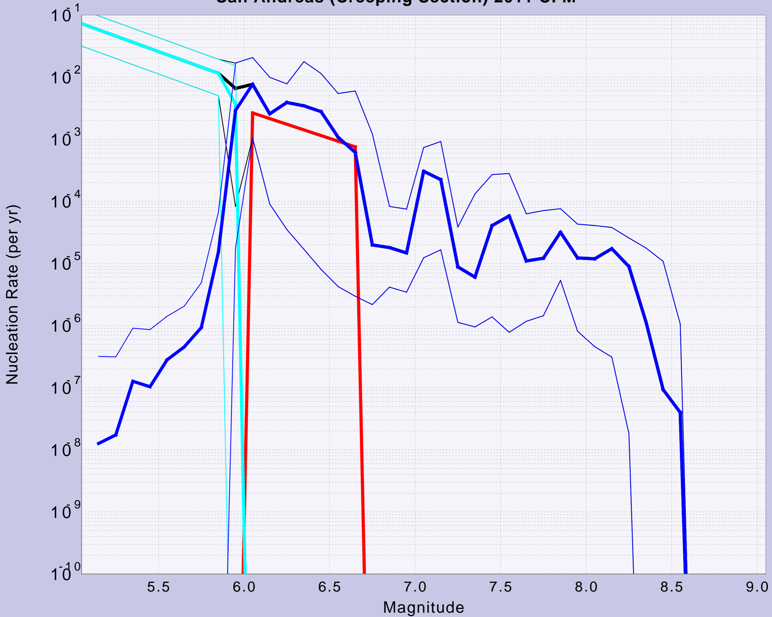
San Andreas (Creeping Section) 2011 CFM
