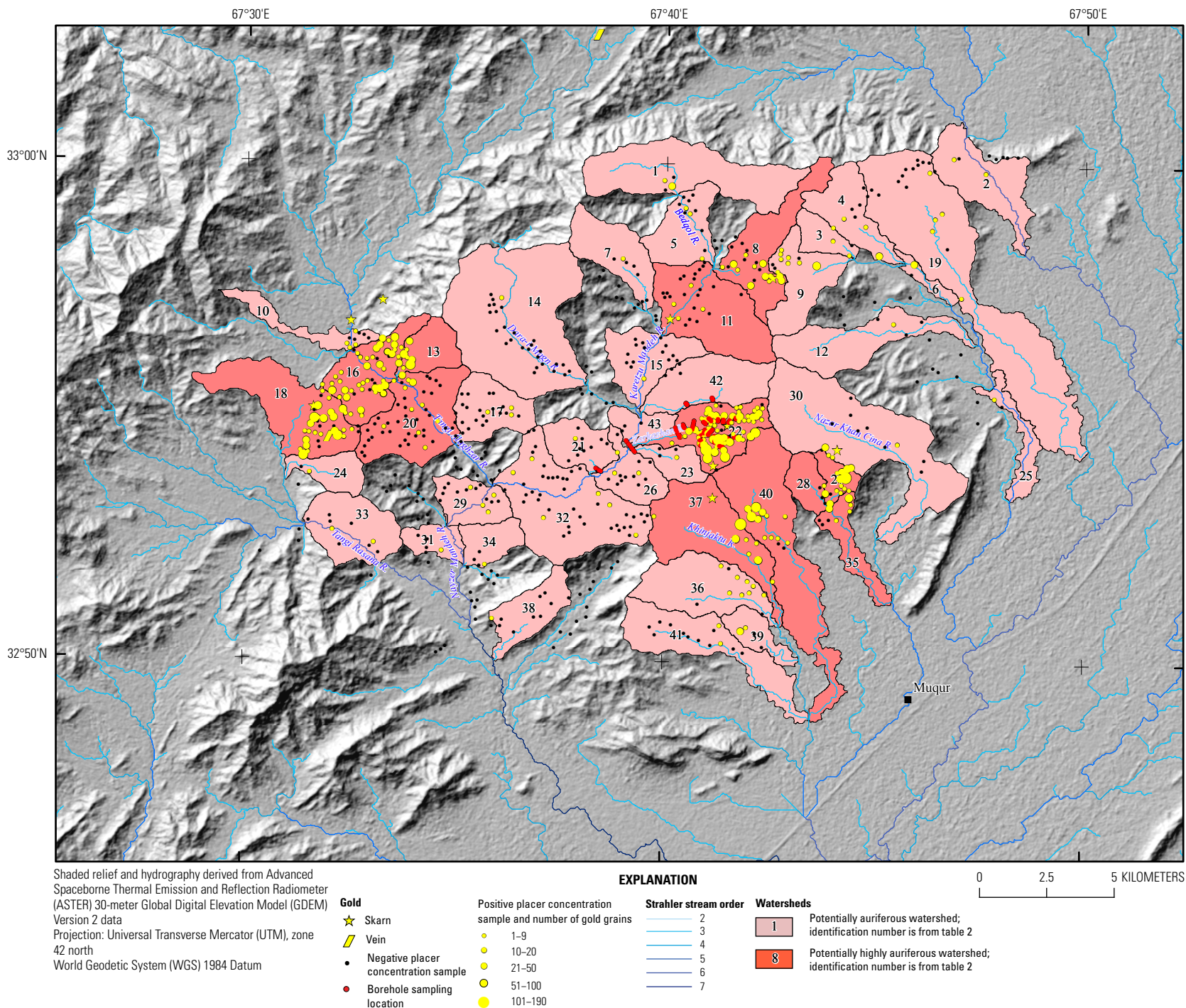
Figure 3. Map showing the potentially auriferous and potentially highly auriferous watersheds in the central part of the Zarkashan AOI.
