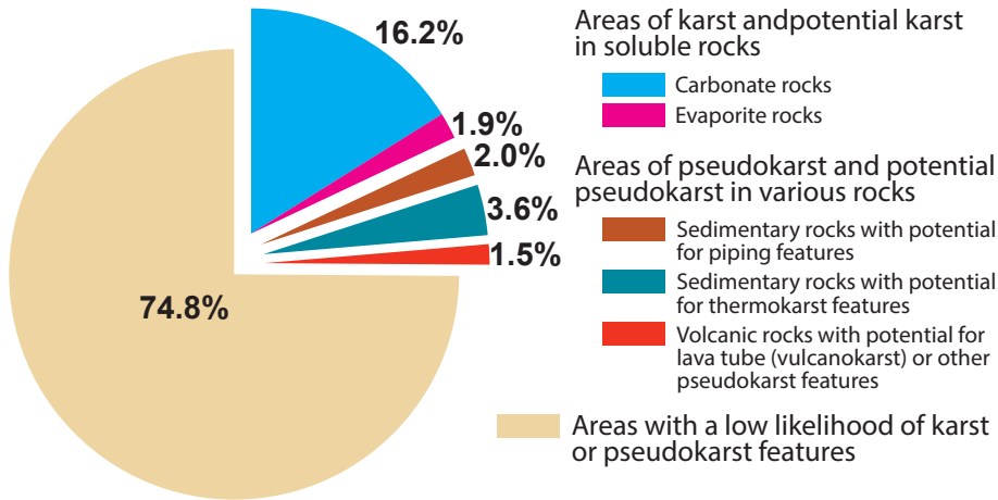
Figure 6. Chart showing proportion of the area of the 50 United States underlain by rocks and sediments having karst or pseudokarst features or a potential for them.
