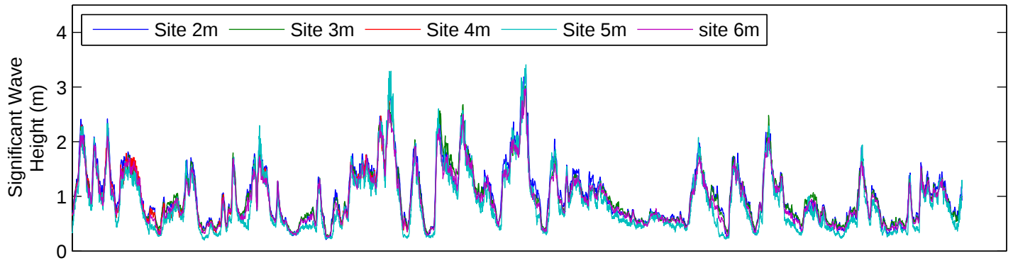
Mean-Removed Pressure Observations Fire Island 2012
