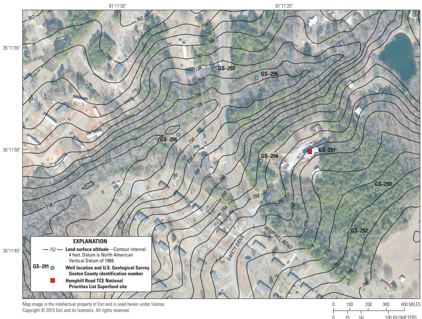
Figure 2. Topography near the Hemphill Road TCE National Priorities List Superfund site and new wells logged as part of the study, Gastonia, Gaston County, North Carolina.
