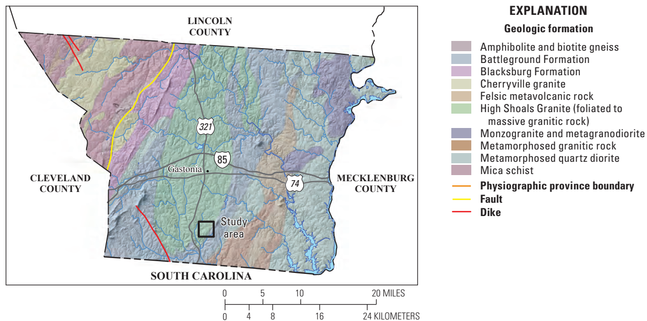
Figure 1. Physiographic provinces in North Carolina, and the Hemphill Road TCE National Priorities List Superfund site and associated local geologic units, Gastonia, North Carolina.
