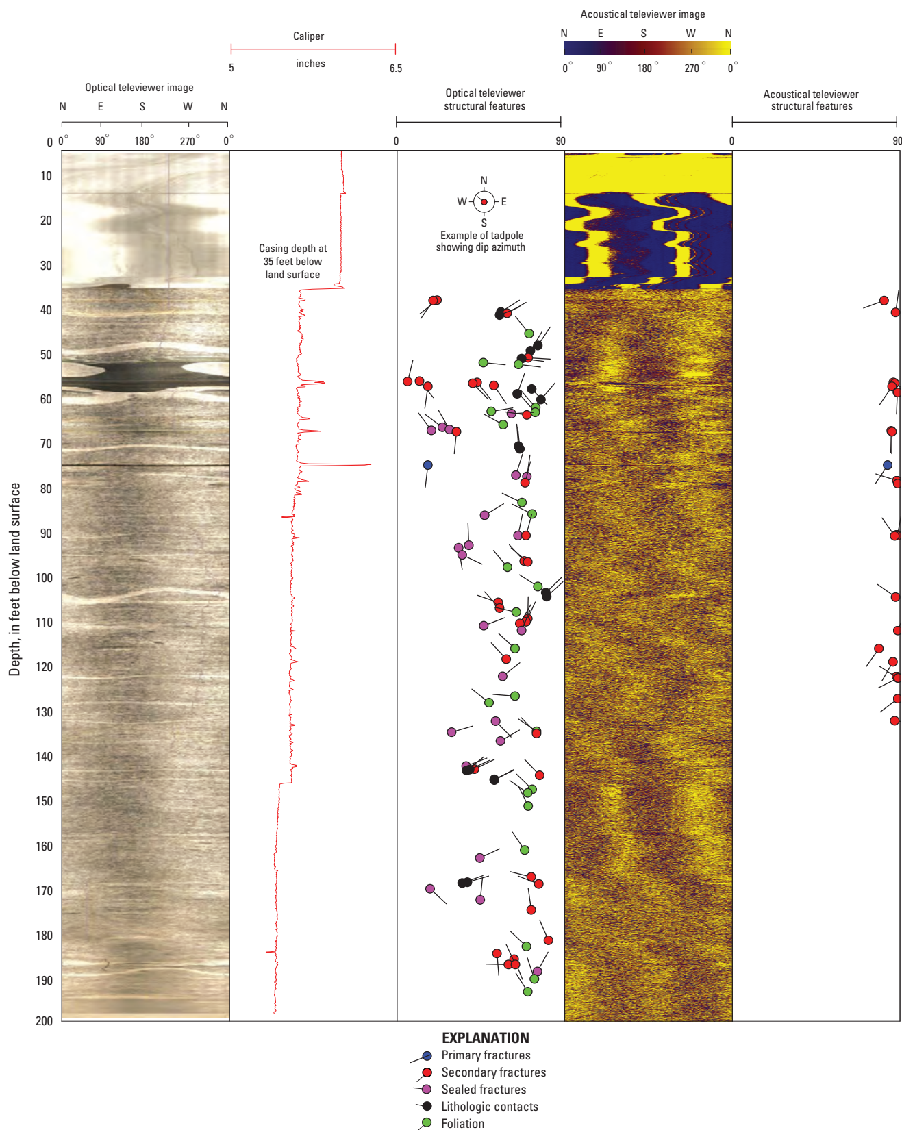
Figure 1-6. Optical televiwer image and structural orientations of subsurface features in well GS-296, near the Hemphill Road TCE National Priorities List Superfund site, Gastonia, Gaston County, North Carolina.
