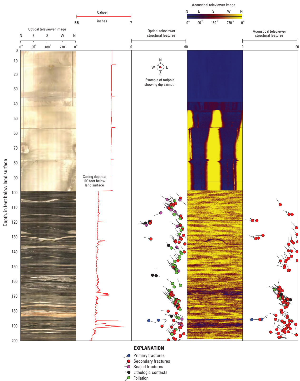
Figure 1-2. Optical televIEWER image and structural orientations of subsurface features in well GS-292, near the Hemphill Road TCE National Priorities List Superfund site, Gastonia, Gaston County, North Carolina.
