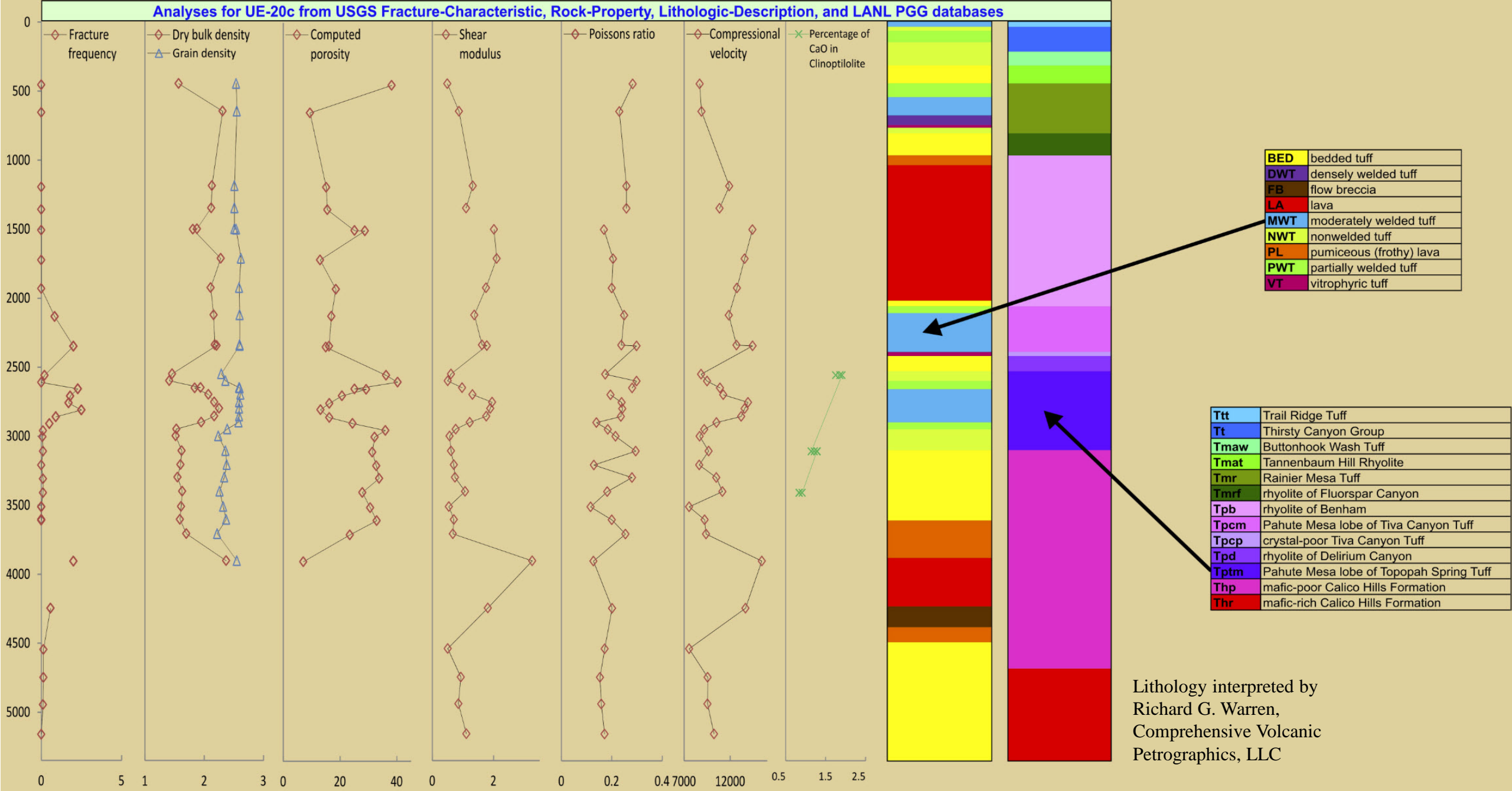
Figure 4. Representation of rock column derived from lithologic records compared with profiles from fracture characteristic, rock property and geochemical database records for the UE-20c borehole, Nevada National Security Site, Nye County, Nevada
