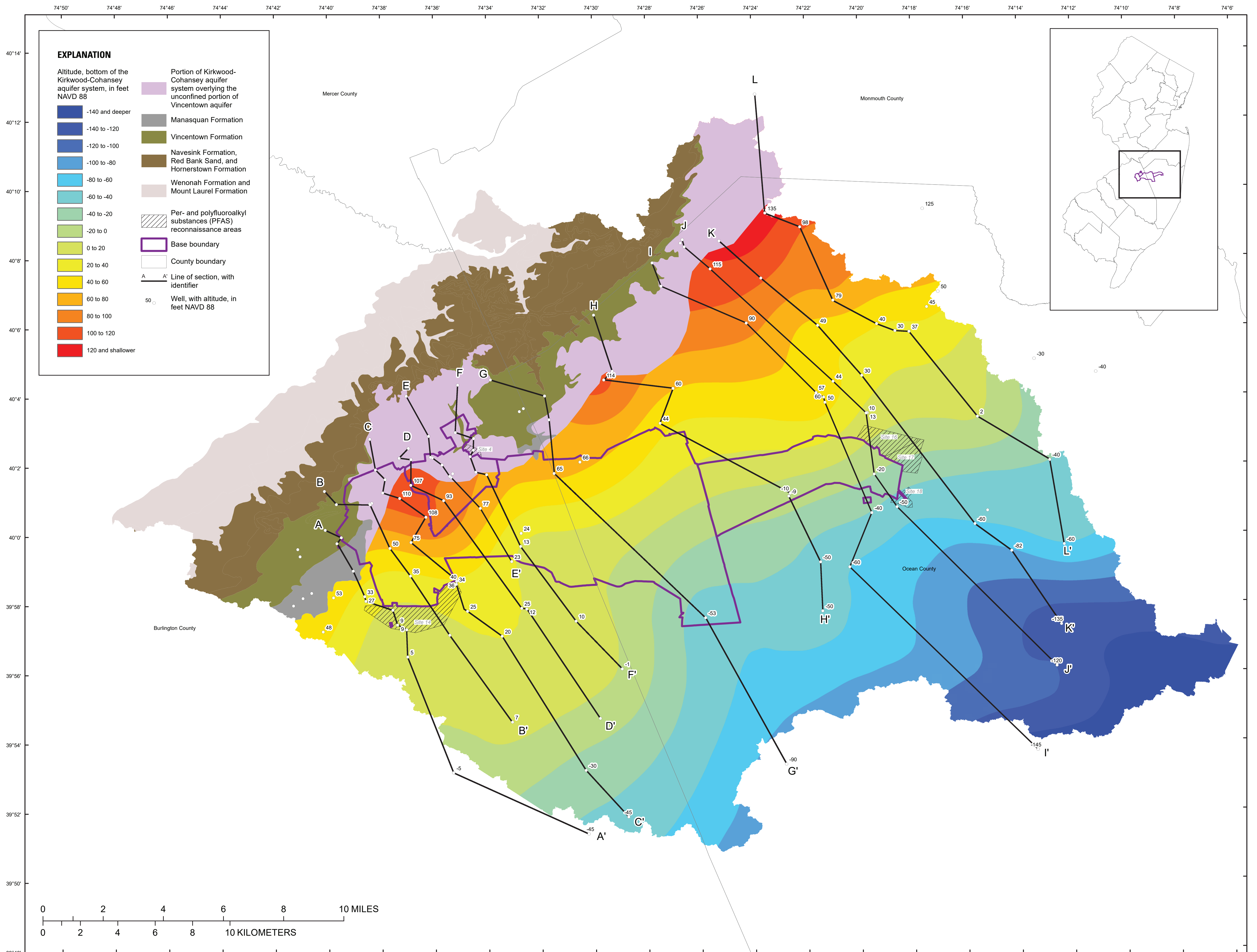
Bottom of the Kirkwood-Cohansey aquifer system, Joint Base McGuire-Dix-Lakehurst and vicinity, New Jersey
