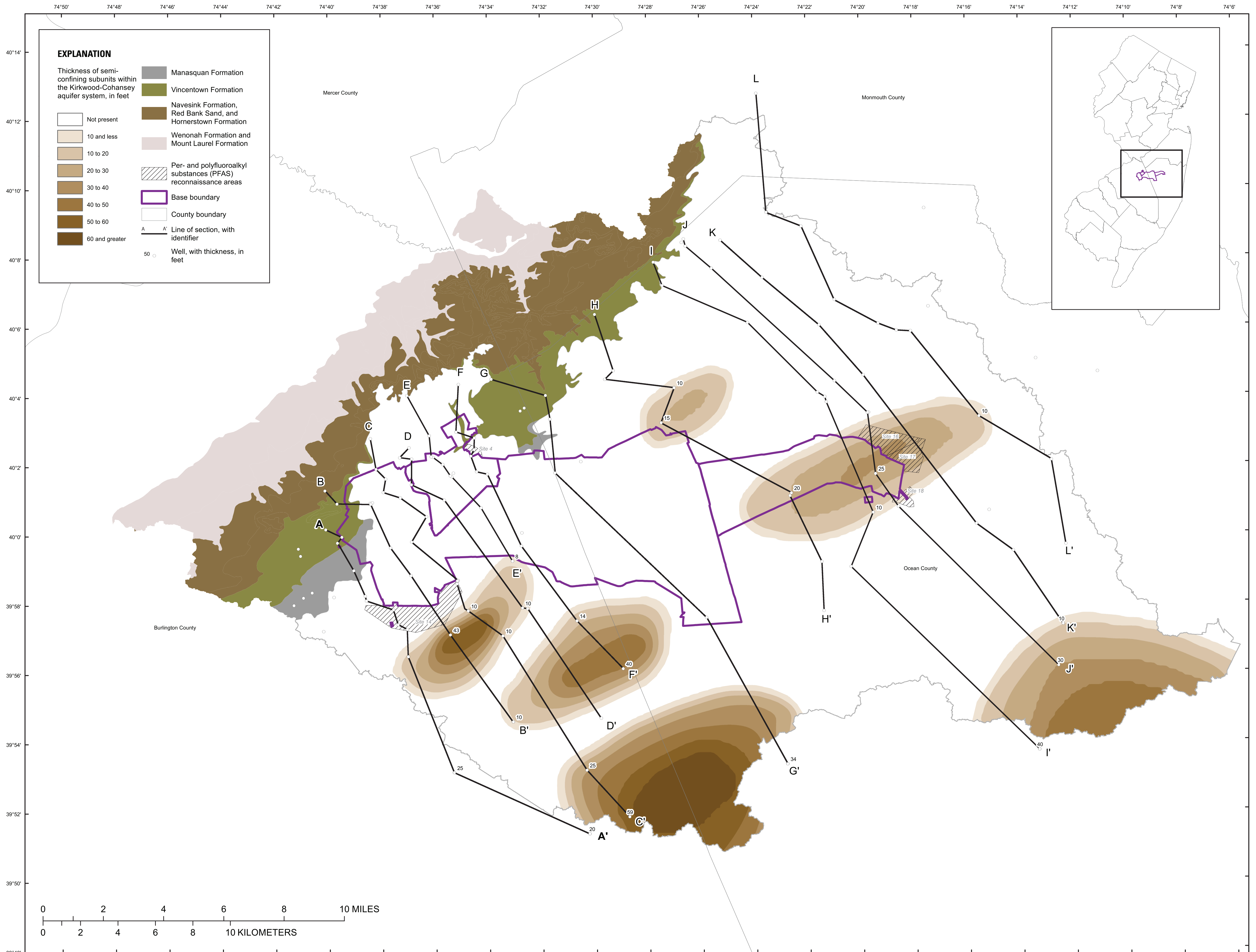
Thickness of semi-confining subunits within the Kirkwood-Cohansey aquifer system, Joint Base McGuire-Dix-Lakehurst and vicinity, New Jersey
