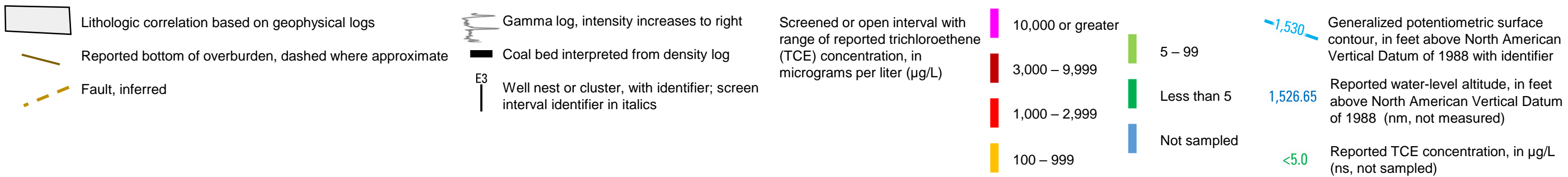
Section C-C' with generalized potentiometric surfaces and trichloroethene concentrations, Valmont TCE Superfund Site, Luzerne County, Pennsylvania, February-March 2020
