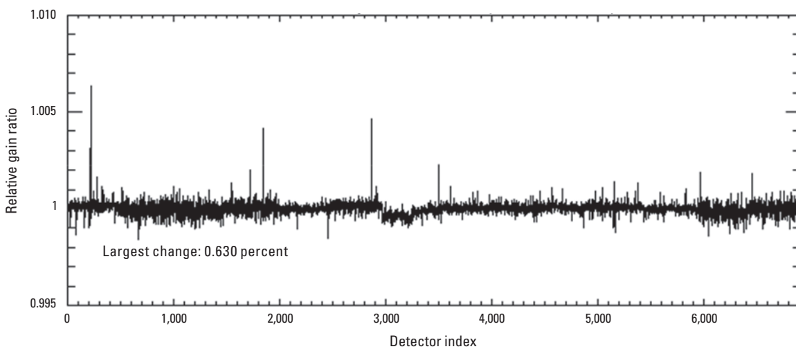
Figure 29. Landsat 8 Operational Land Imager shortwave infrared 1 band per-detector change in relative gains between quarter 4, 2022, and quarter 1, 2023.
