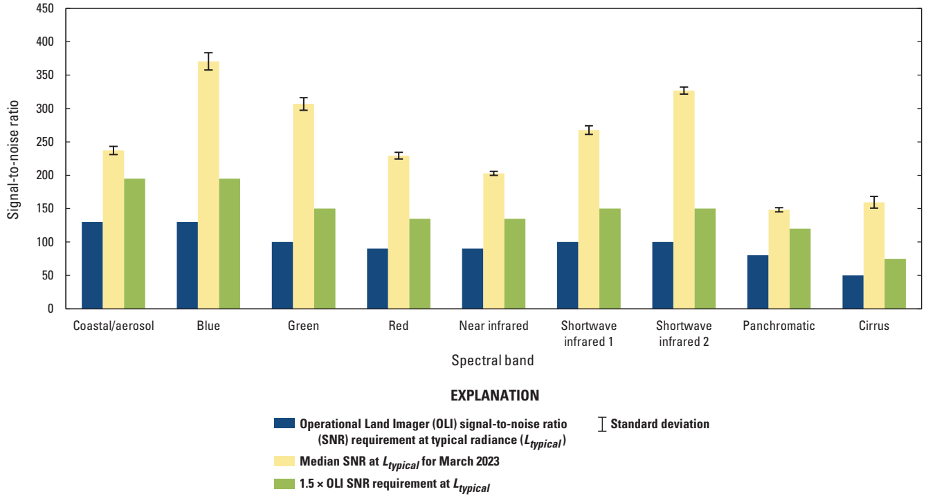
Figure 1. Landsat 8 Operational Land Imager signal-to-noise performance, March 2023.
