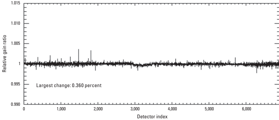
Figure 30. Landsat 8 Operational Land Imager shortwave infrared 2 band per-detector change in relative gains between quarter 4, 2022, and quarter 1, 2023.
