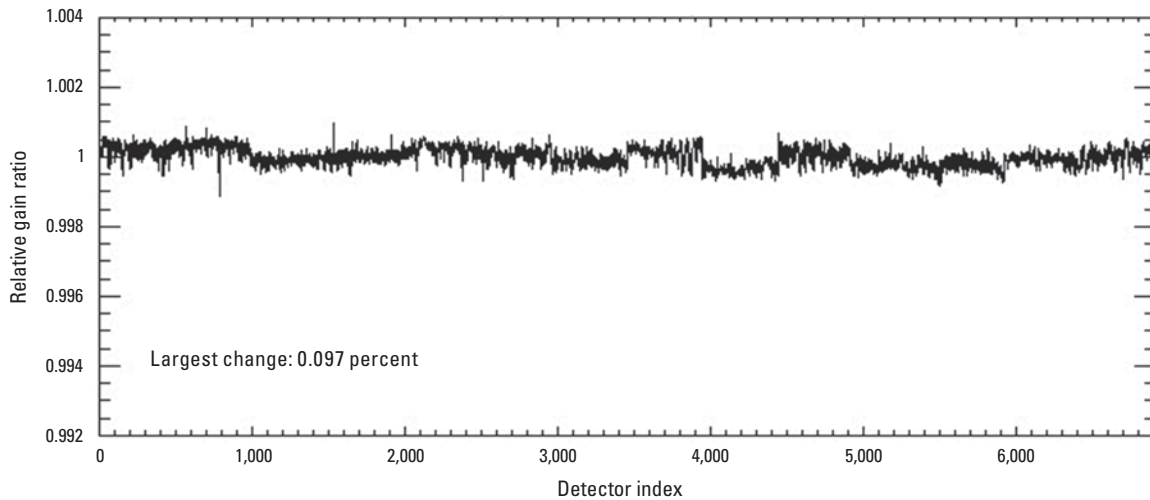
Figure 28. Landsat 8 Operational Land Imager coastal/aerosol band per-detector change in relative gains between quarter 4, 2022, and quarter 1, 2023.
