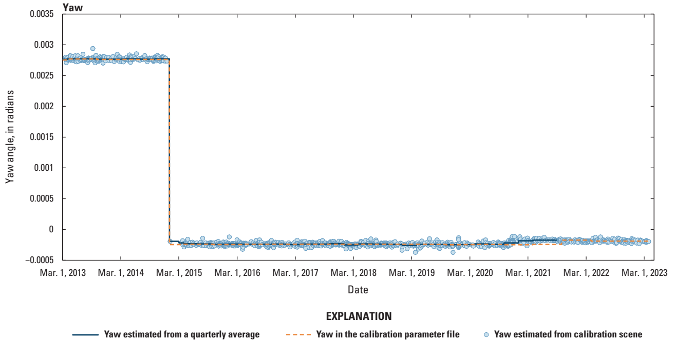
Figure 39. Landsat 8 Thermal Infrared Sensor to Operational Land Imager lifetime yaw alignment.
