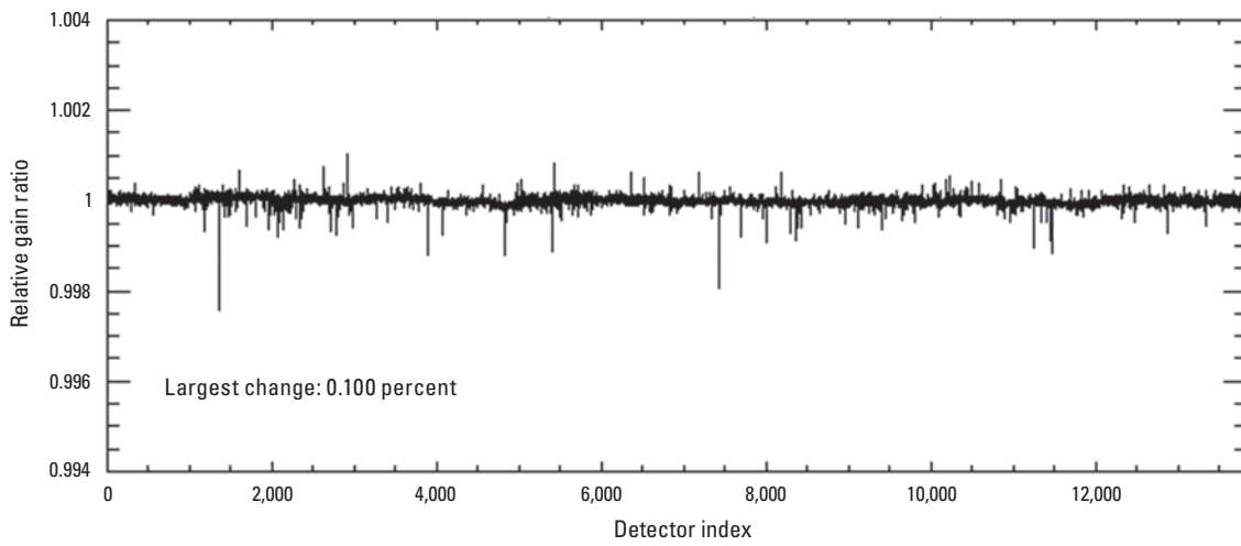
Figure 31. Landsat 8 Operational Land Imager panchromatic band per-detector change in relative gains between quarter 4, 2022, and quarter 1, 2023.
