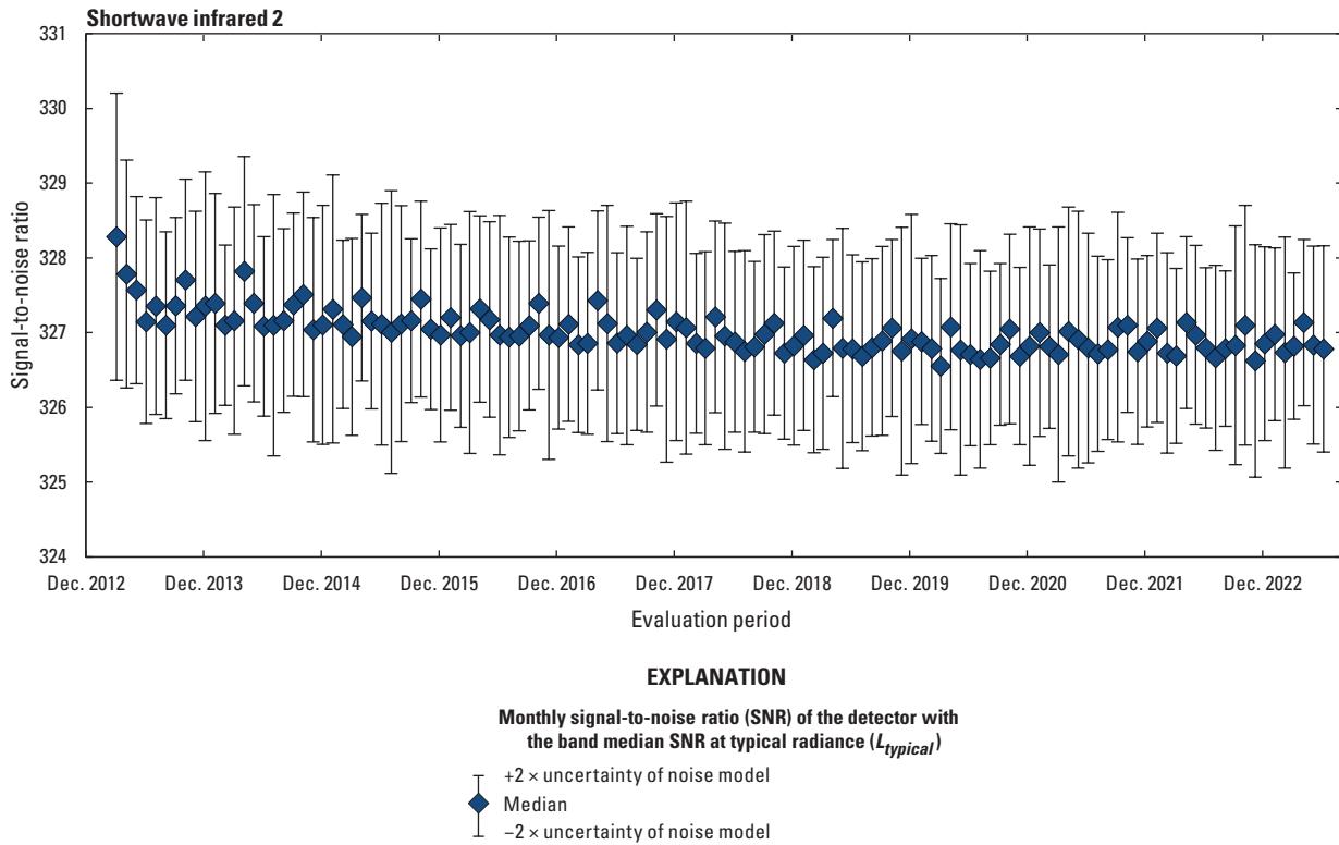
Figure 8. Landsat 8 Operational Land Imager shortwave infrared 2 band lifetime signal-to-noise ratio stability.
