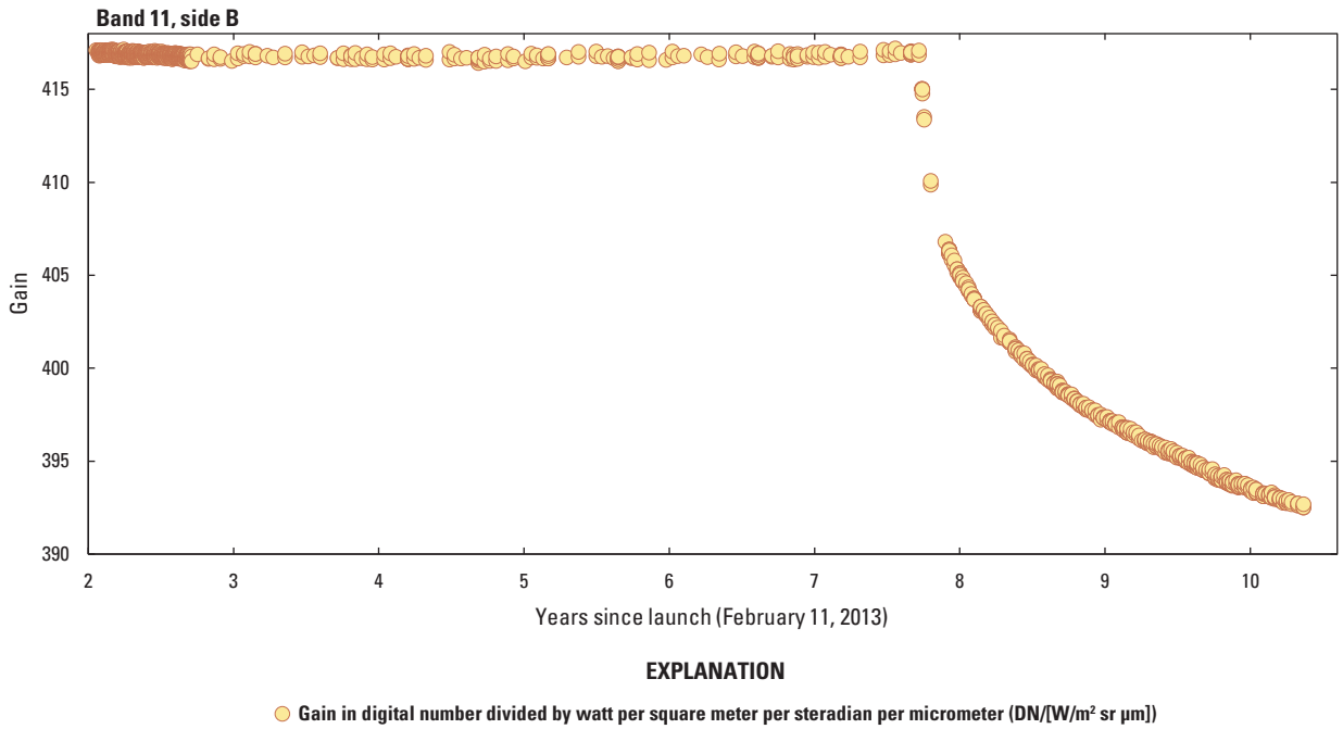
Figure 25. Landsat 8 Thermal Infrared Sensor band 11 radiometric stability (side B).
