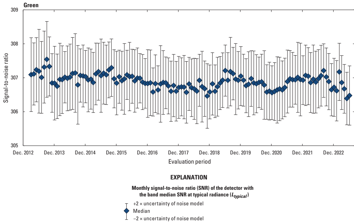
Figure 4. Landsat 8 Operational Land Imager green band lifetime signal-to-noise ratio stability.
