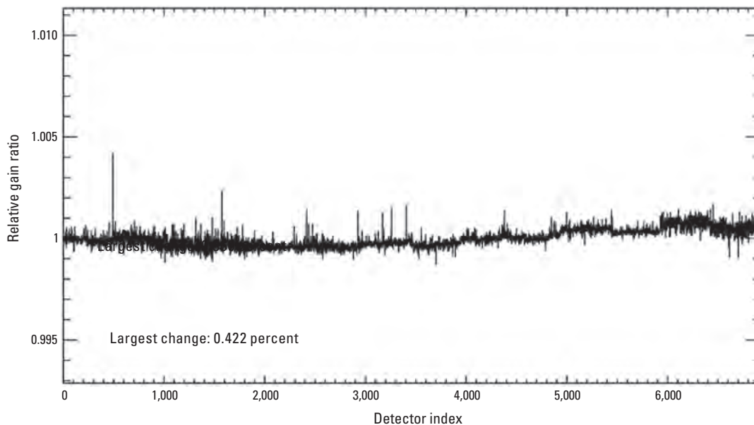
Figure 30. Landsat 8 Operational Land Imager shortwave infrared 2 band per-detector change in relative gains between quarter 1 and quarter 2, 2023.
