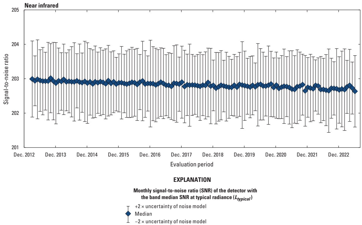
Figure 6. Landsat 8 Operational Land Imager near infrared band lifetime signal-to-noise ratio stability.
