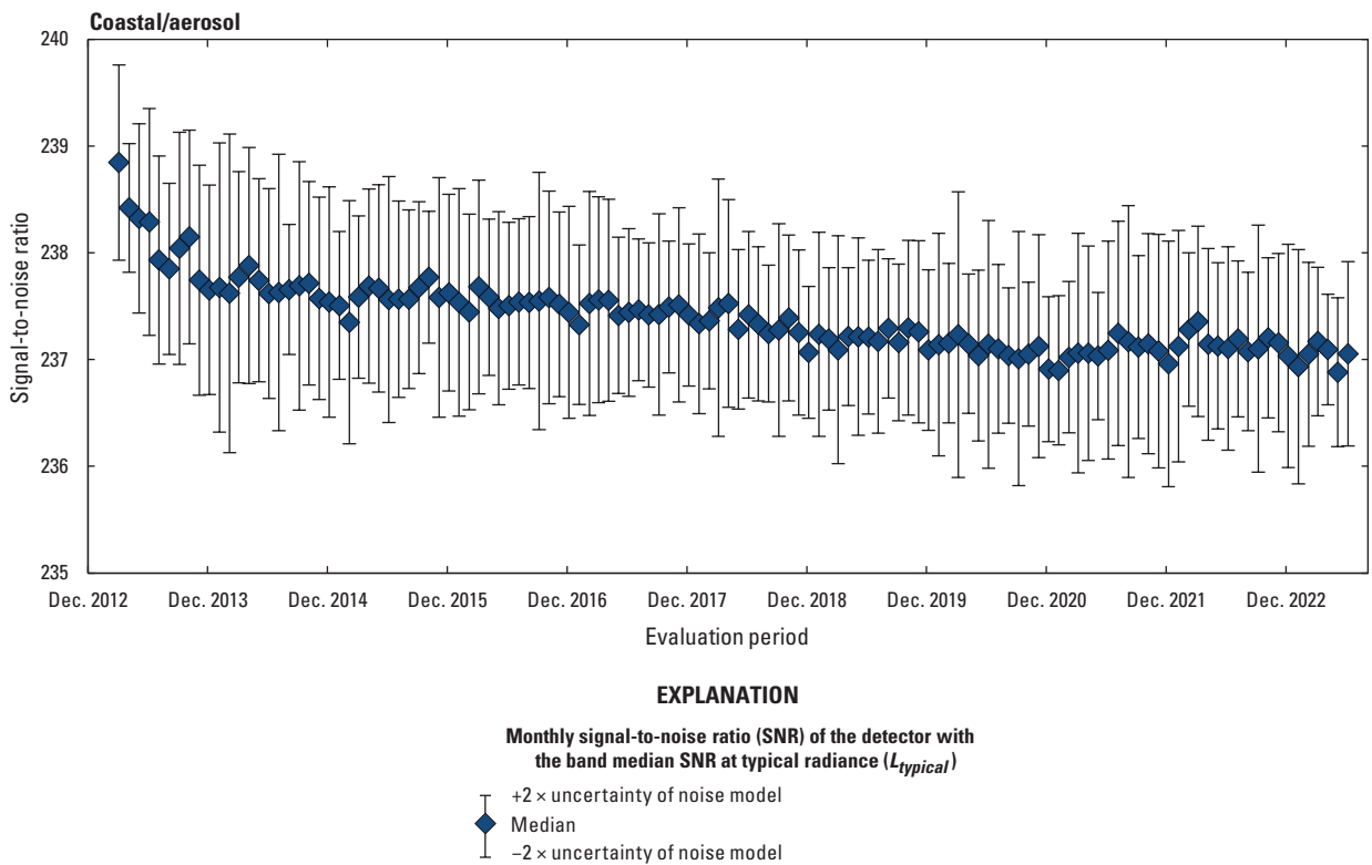
Figure 2. Landsat 8 Operational Land Imager coastal/aerosol band lifetime signal-to-noise ratio stability.
