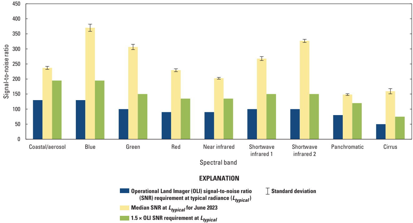
Figure 1. Landsat 8 Operational Land Imager signal-to-noise ratio performance, June 2023.
