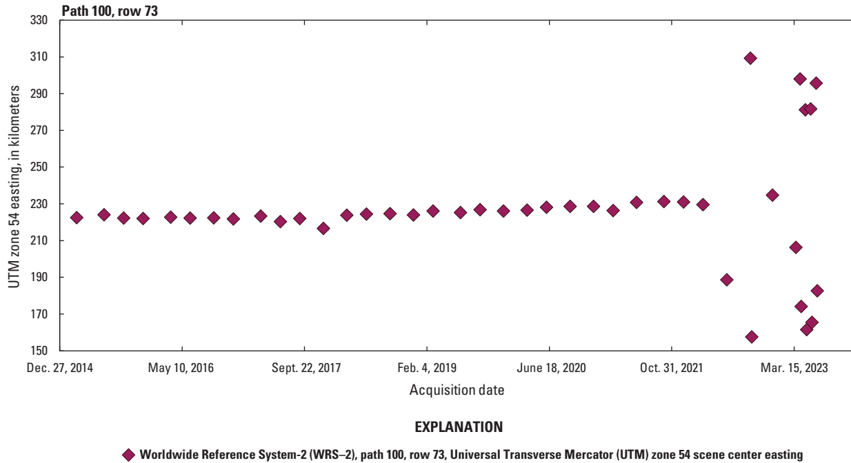
Figure 51. Landsat 7 lifetime orbital drift from World Reference System-2 (path 100, row 73).
