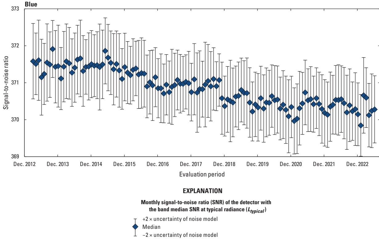
Figure 3. Landsat 8 Operational Land Imager blue band lifetime signal-to-noise ratio stability.
