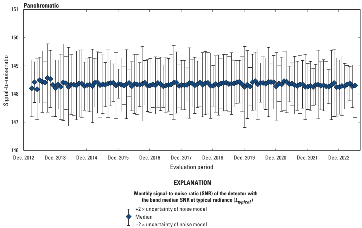
Figure 10. Landsat 8 Operational Land Imager panchromatic band lifetime signal-to-noise ratio stability.
