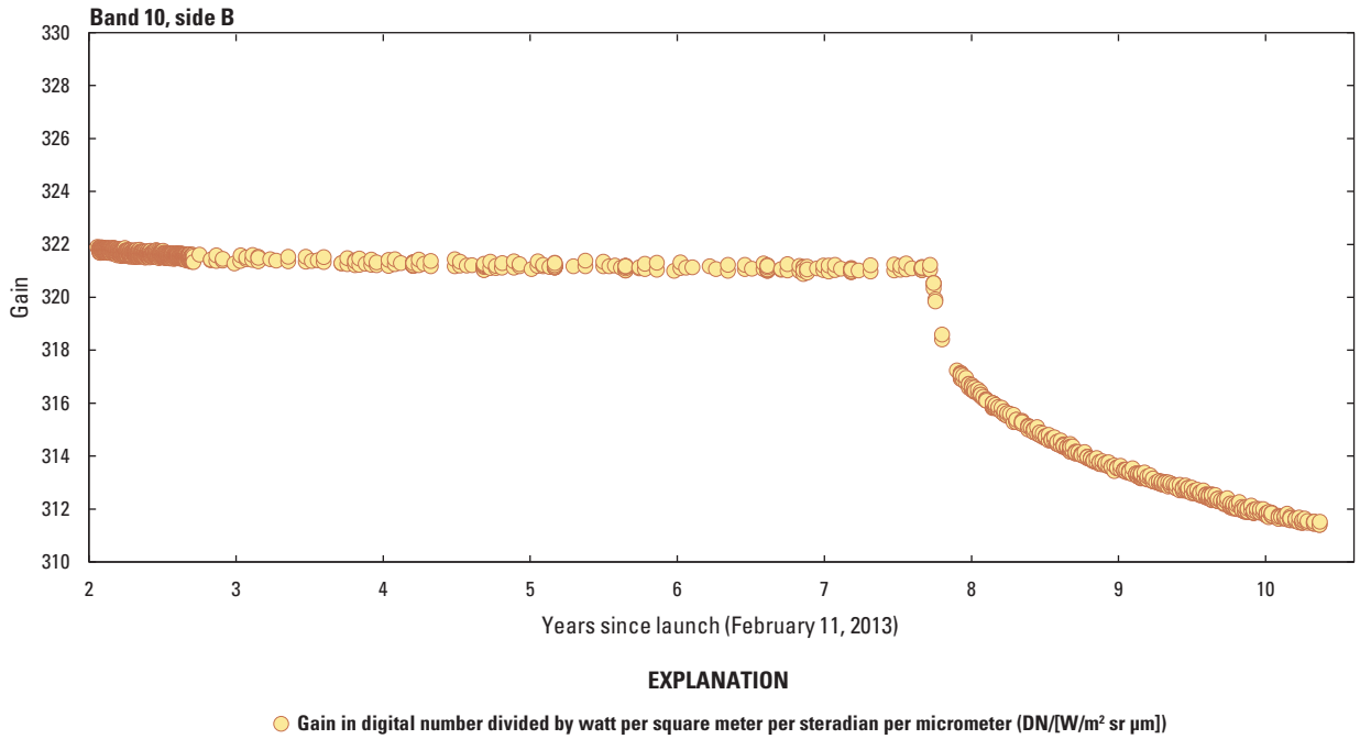
Figure 24. Landsat 8 Thermal Infrared Sensor band 10 radiometric stability (side B).
