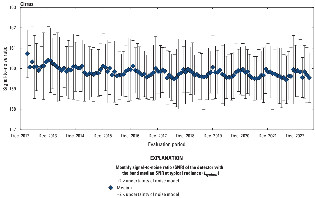
Figure 9. Landsat 8 Operational Land Imager cirrus band lifetime signal-to-noise ratio stability.
