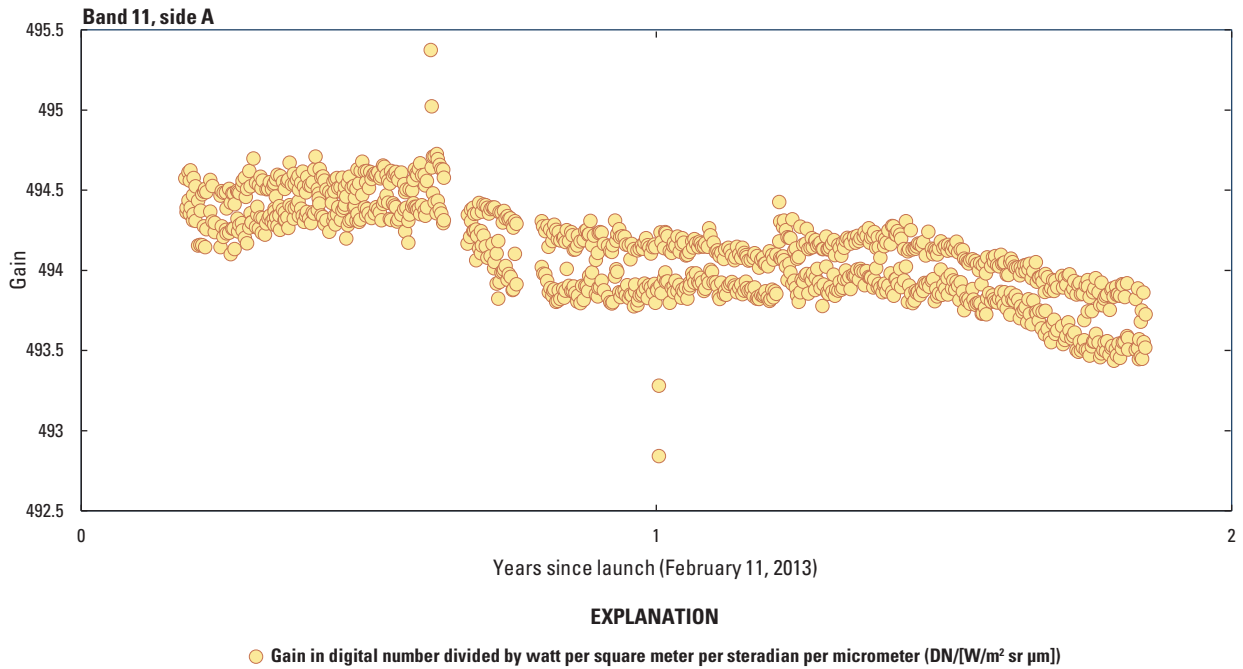
Figure 23. Landsat 8 Thermal Infrared Sensor band 11 radiometric stability (side A).
