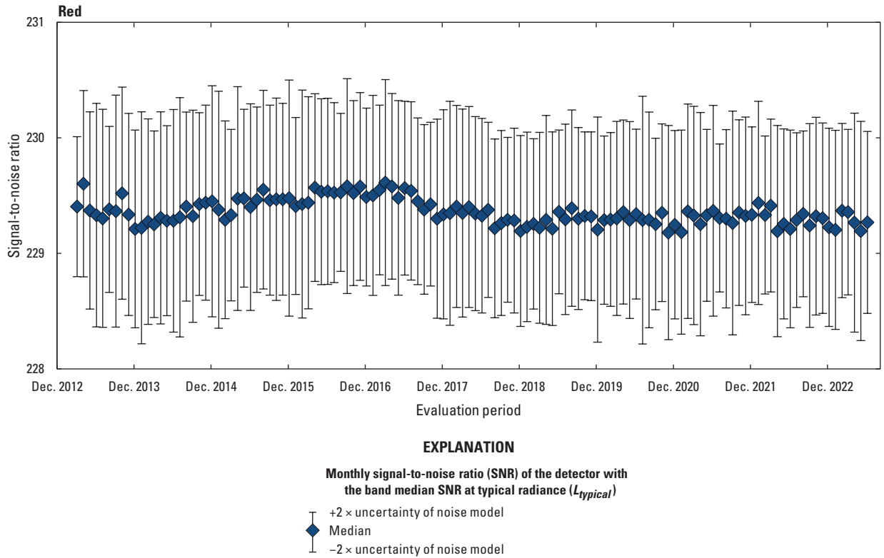
Figure 5. Landsat 8 Operational Land Imager red band lifetime signal-to-noise ratio stability.
