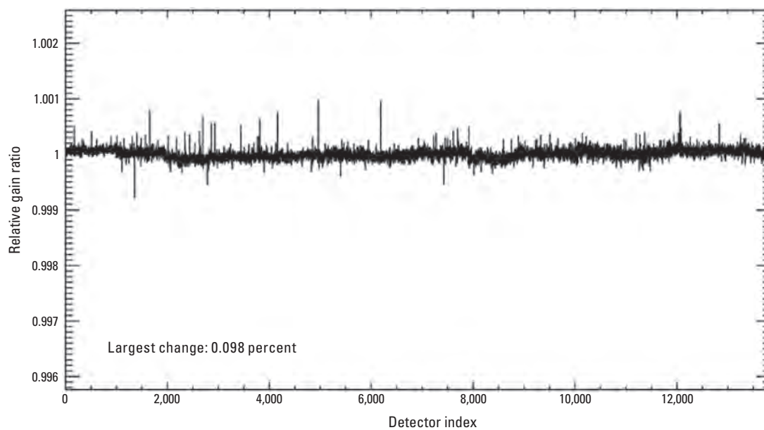
Figure 31. Landsat 8 Operational Land Imager panchromatic band per-detector change in relative gains between quarter 1 and quarter 2, 2023.
