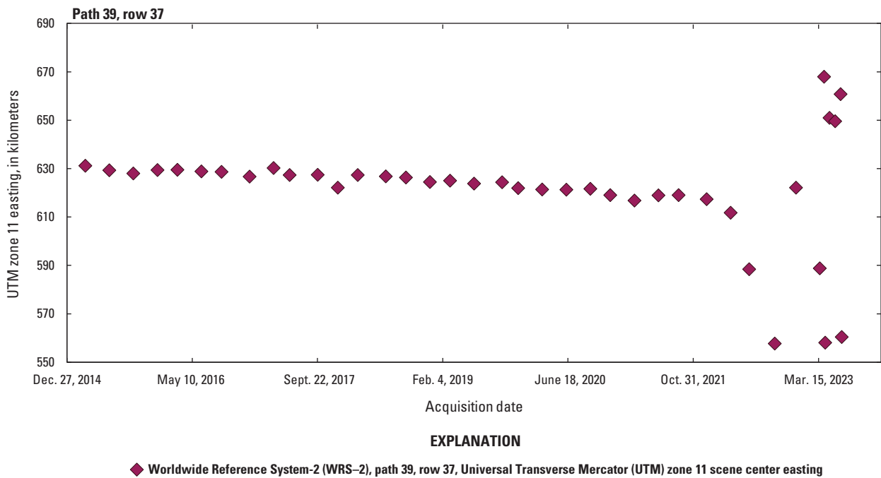
Figure 50. Landsat 7 lifetime orbital drift from World Reference System-2 (path 39, row 37).
