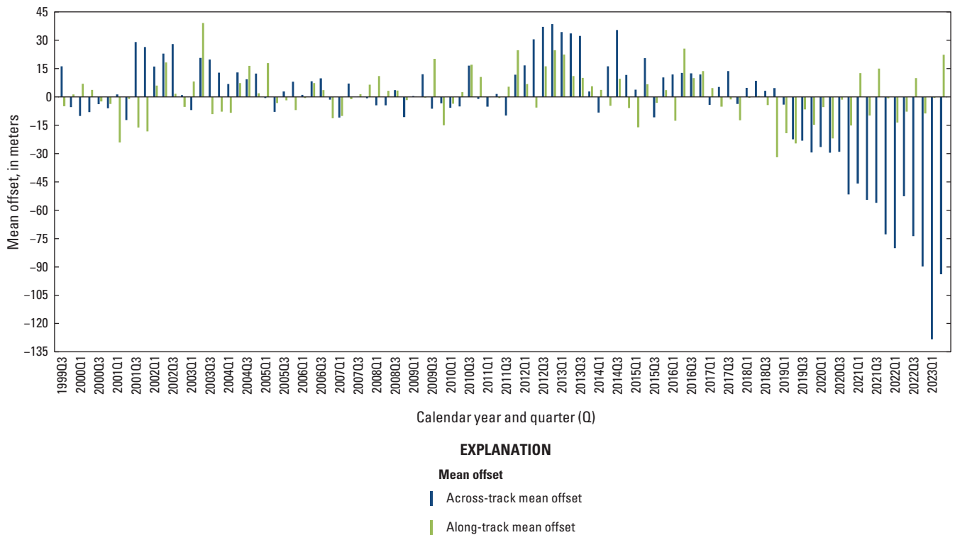
Figure 47. Landsat 7 lifetime mean offsets per quarter.
