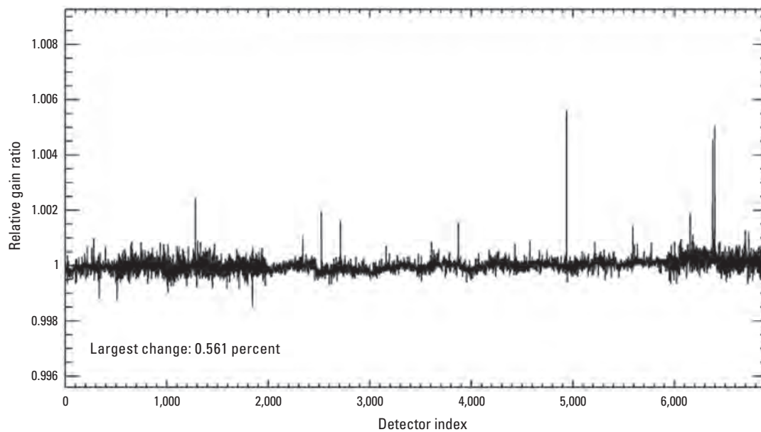
Figure 29. Landsat 8 Operational Land Imager shortwave infrared 1 band per-detector change in relative gains between quarter 1 and quarter 2, 2023.
