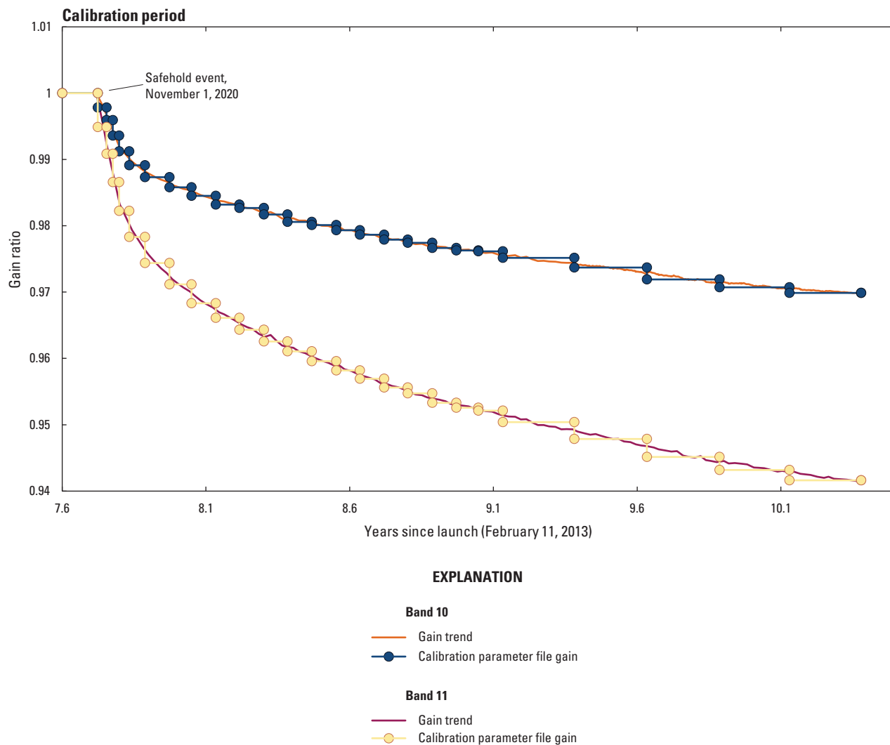
Figure 27. Landsat 8 Thermal Infrared Sensor gain degradation since the safehold event on November 1, 2020.
