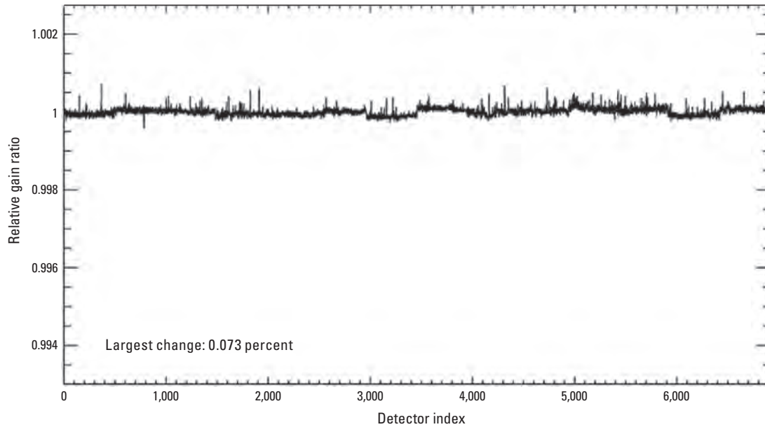
Figure 28. Landsat 8 Operational Land Imager coastal/aerosol band per-detector change in relative gains between quarter 1 and quarter 2, 2023.
