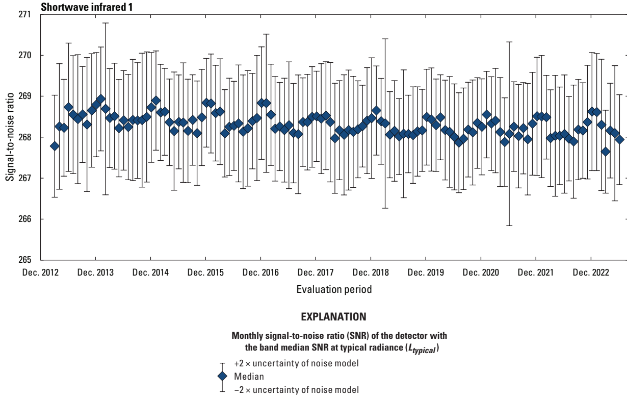
Figure 7. Landsat 8 Operational Land Imager shortwave infrared 1 band lifetime signal-to-noise ratio stability.
