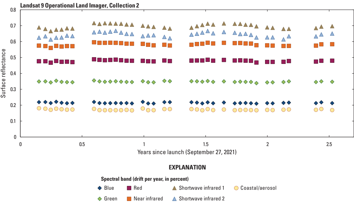
Figure 82. Graph showing Libya 4 pseudoinvariant calibration site surface reflectance trending, Landsat 9 Operational Land Imager, Collection 2.
