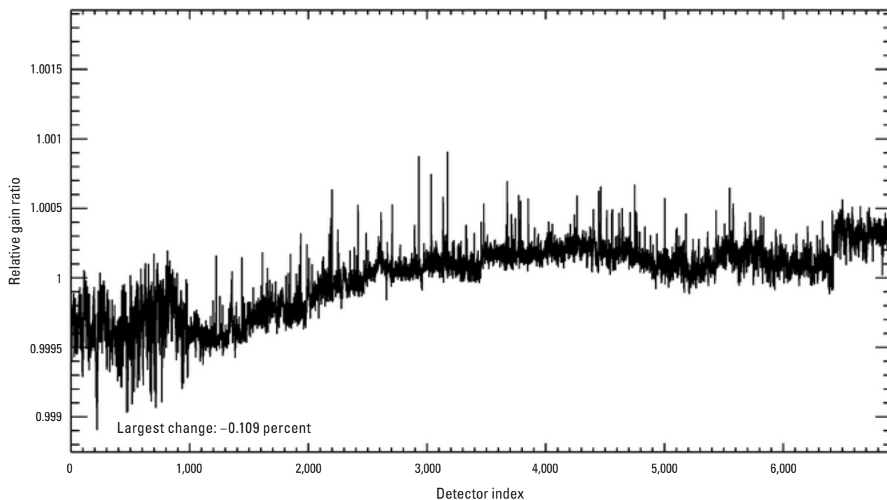
Figure 24. Graph showing Landsat 9 Operational Land Imager coastal/aerosol band per-detector change in relative gains between quarter 1 and quarter 2, 2024.
