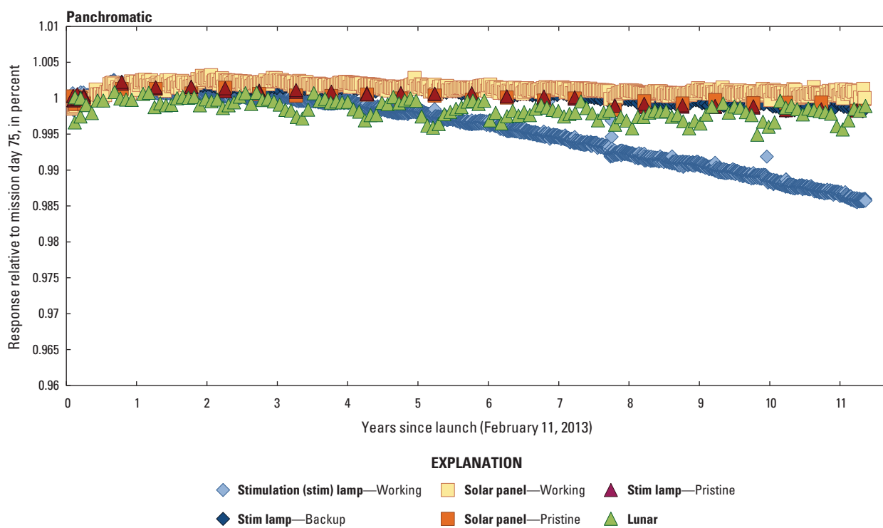
Figure 59. Graph showing Landsat 8 Operational Land Imager panchromatic band lifetime radiometric stability.
