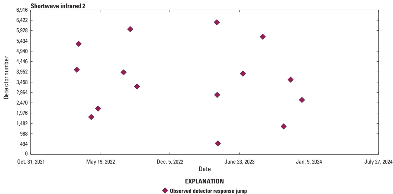
Figure 29. Graph showing Landsat 9 Operational Land Imager shortwave infrared 2 lifetime jumps in detector responsivity.
