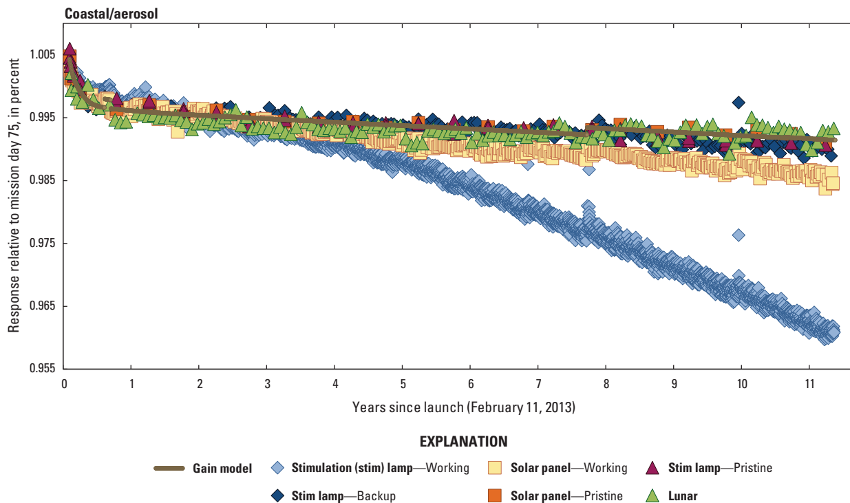
Figure 52. Graph showing Landsat 8 Operational Land Imager coastal/aerosol band lifetime radiometric stability.
