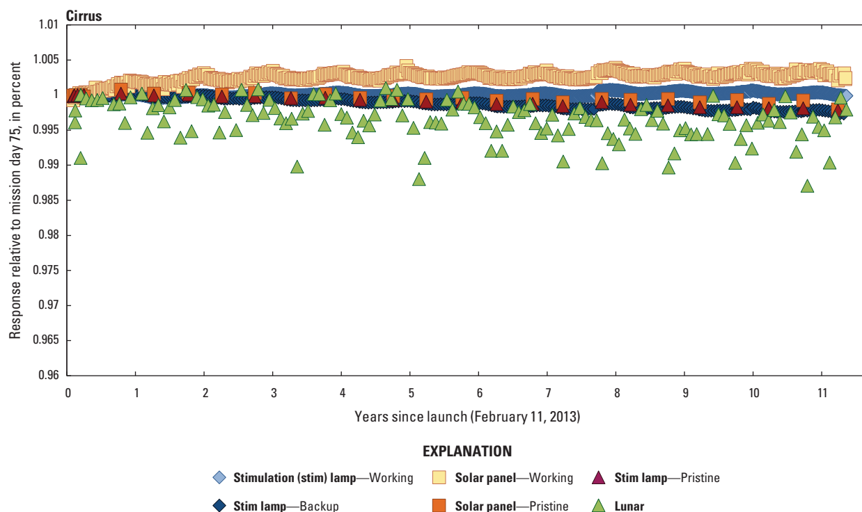
Figure 60. Graph showing Landsat 8 Operational Land Imager cirrus band lifetime radiometric stability.
