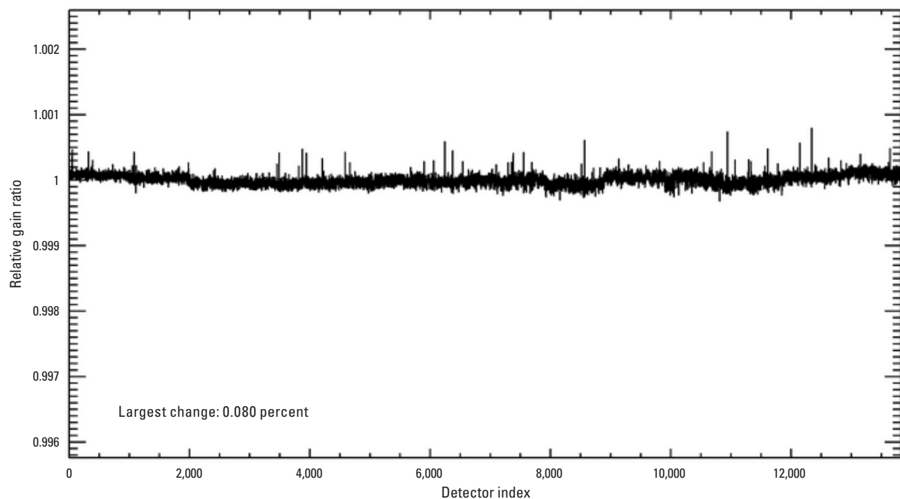
Figure 70. Graph showing Landsat 8 Operational Land Imager panchromatic band per-detector change in relative gains between quarter 1 and quarter 2, 2024.
