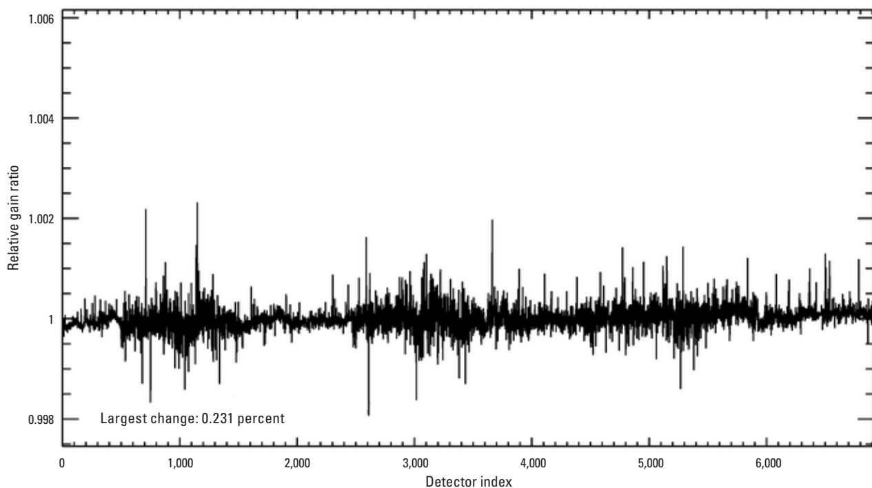
Figure 26. Graph showing Landsat 9 Operational Land Imager shortwave infrared 2 band per-detector change in relative gains between quarter 1 and quarter 2, 2024.
