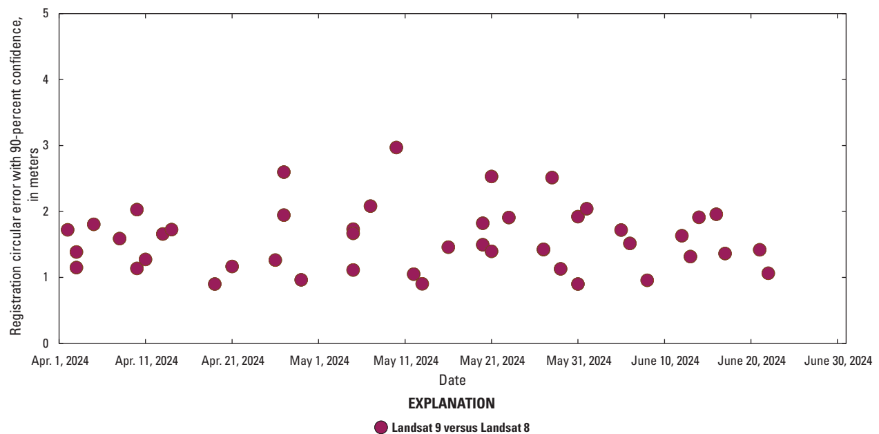
Figure 39. Graph showing coregistration error between Landsat 9 and Landsat 8 Level 1 terrain-corrected products, quarter 2, 2024.
