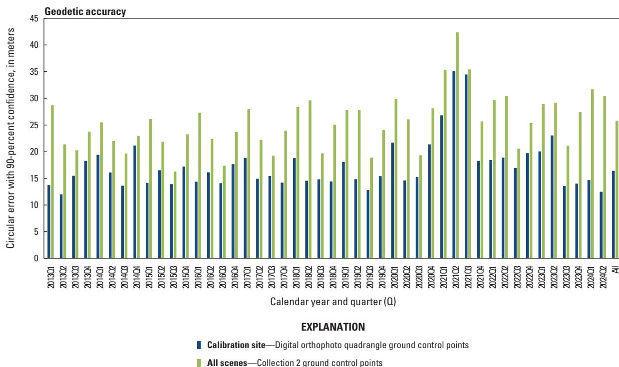
Figure 80. Graph showing Landsat 8 lifetime geodetic accuracy by quarter.
