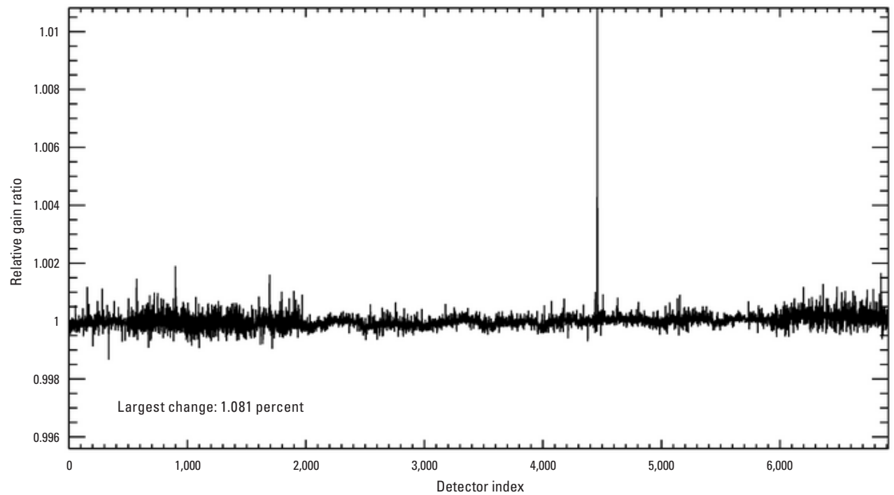
Figure 68. Graph showing Landsat 8 Operational Land Imager shortwave infrared 1 band per-detector change in relative gains between quarter 1 and quarter 2, 2024.
