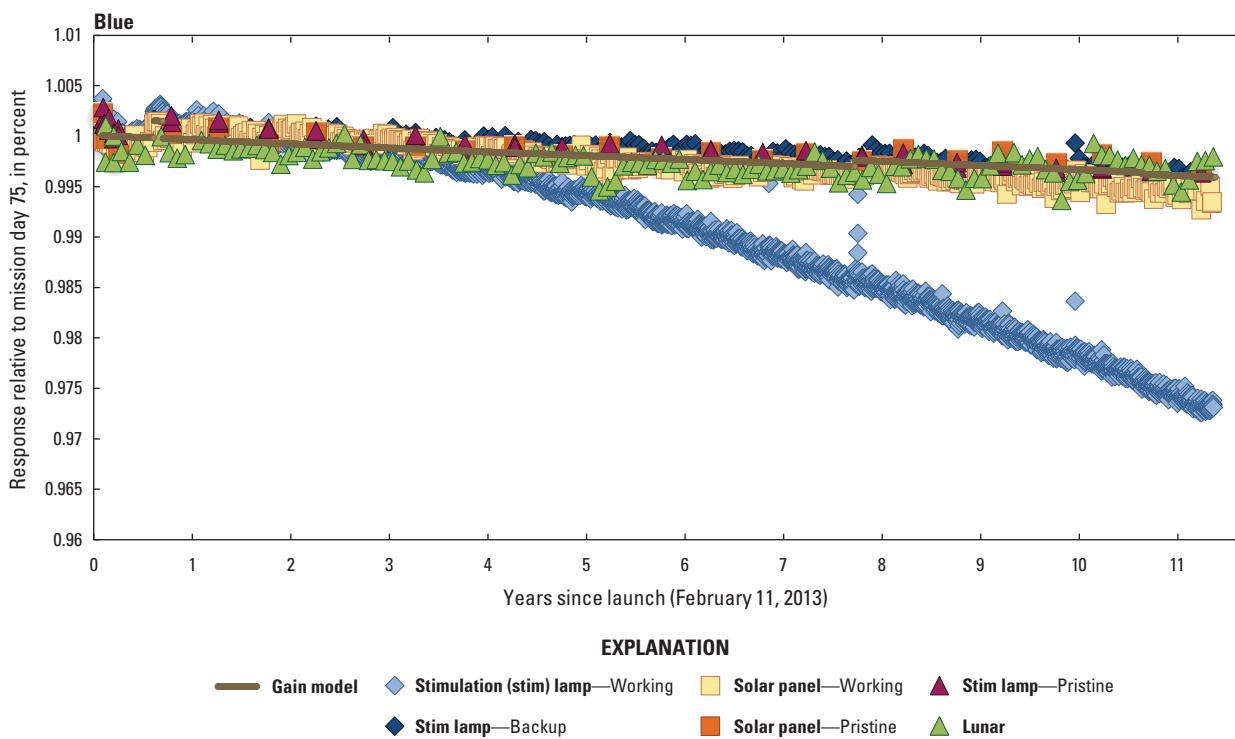
Figure 53. Graph showing Landsat 8 Operational Land Imager blue band lifetime radiometric stability.
