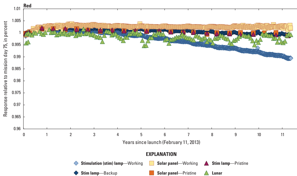
Figure 55. Graph showing Landsat 8 Operational Land Imager red band lifetime radiometric stability.
