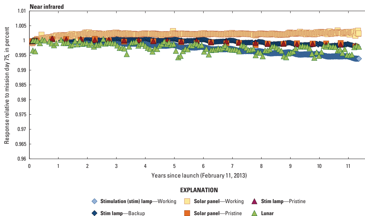
Figure 56. Graph showing Landsat 8 Operational Land Imager near infrared band lifetime radiometric stability.
