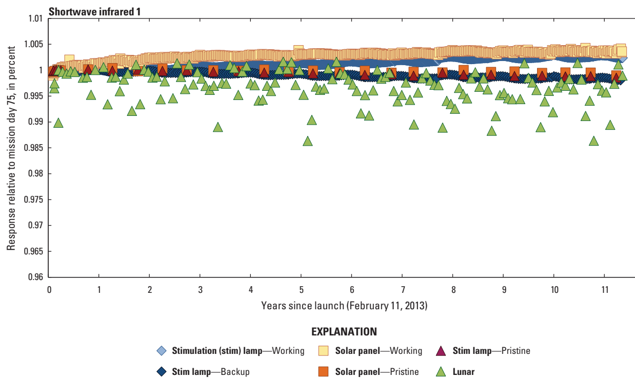
Figure 57. Graph showing Landsat 8 Operational Land Imager shortwave infrared 1 band lifetime radiometric stability.
