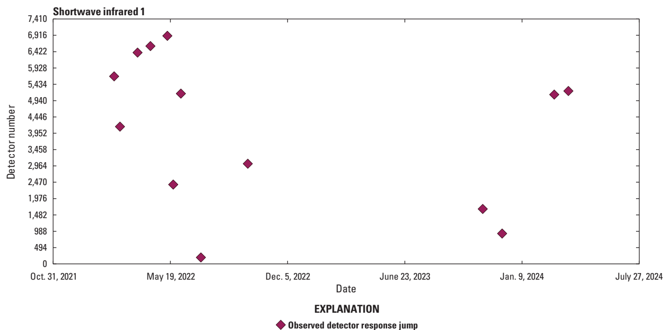
Figure 28. Graph showing Landsat 9 Operational Land Imager shortwave infrared 1 lifetime jumps in detector responsivity.
