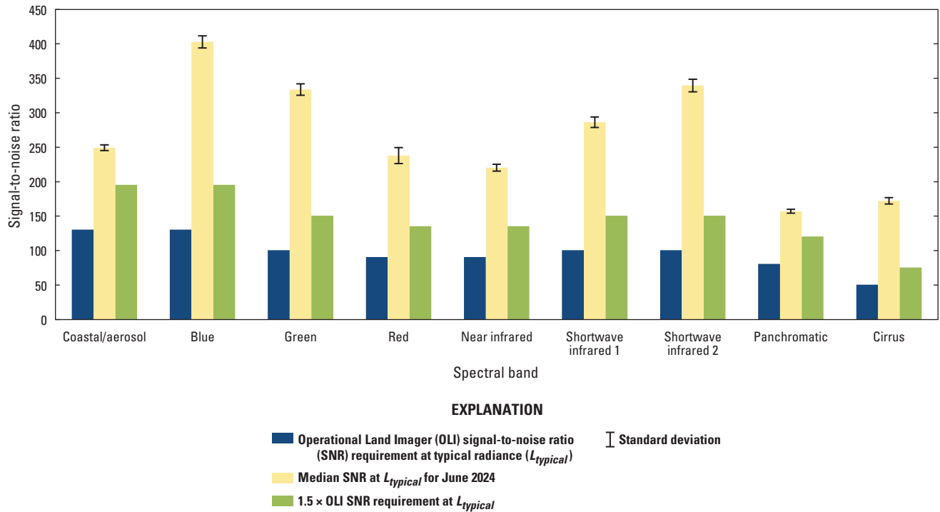
Figure 1. Graph showing Landsat 9 Operational Land Imager signal-to-noise ratio performance, June 2024.
