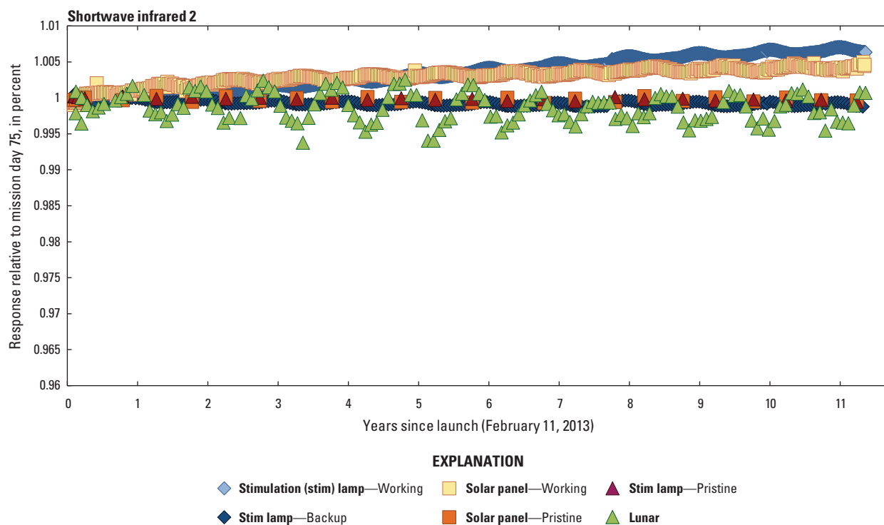
Figure 58. Graph showing Landsat 8 Operational Land Imager shortwave infrared 2 band lifetime radiometric stability.
