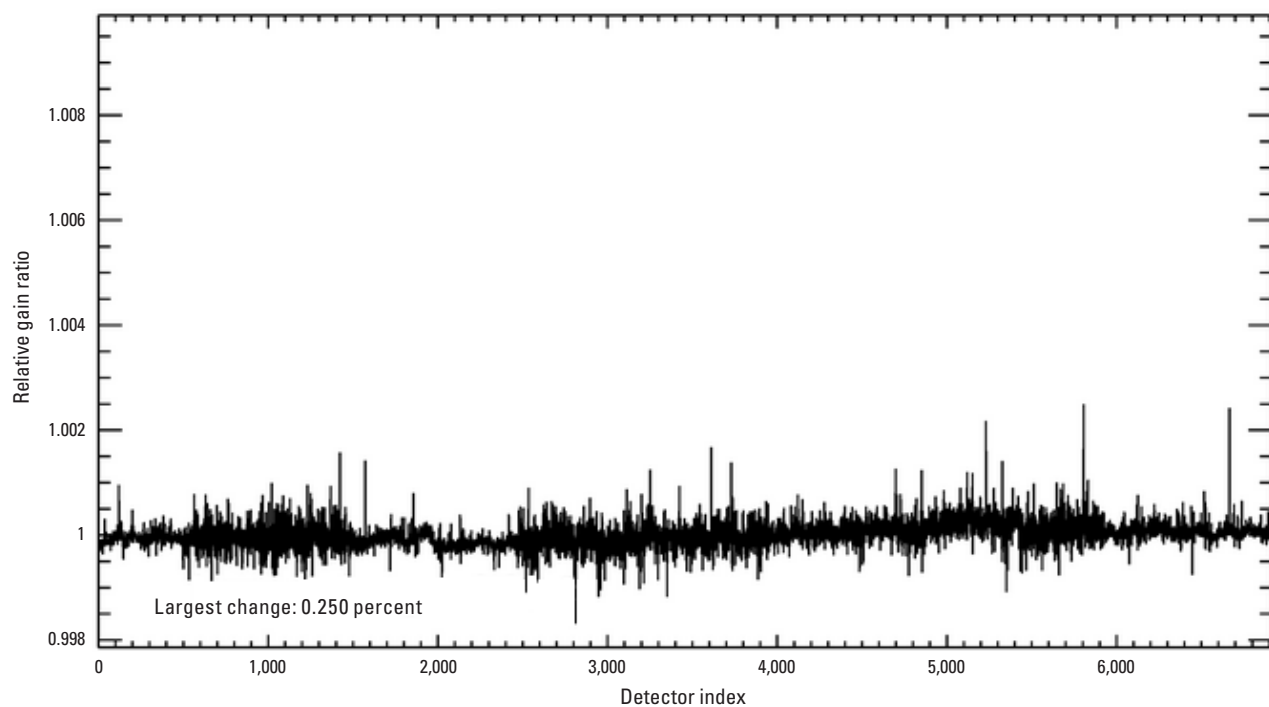
Figure 25. Graph showing Landsat 9 Operational Land Imager shortwave infrared 1 band per-detector change in relative gains between quarter 1 and quarter 2, 2024.
