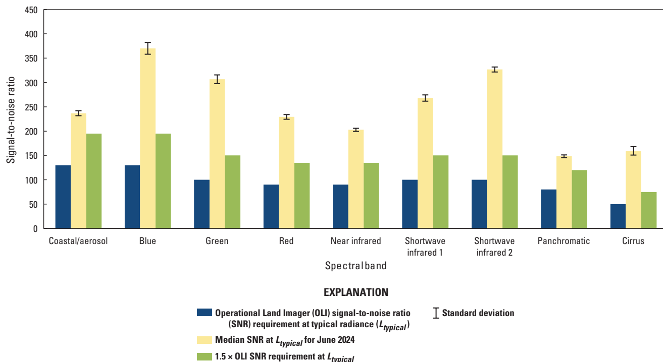
Figure 40. Graph showing Landsat 8 Operational Land Imager signal-to-noise ratio performance, June 2024.
