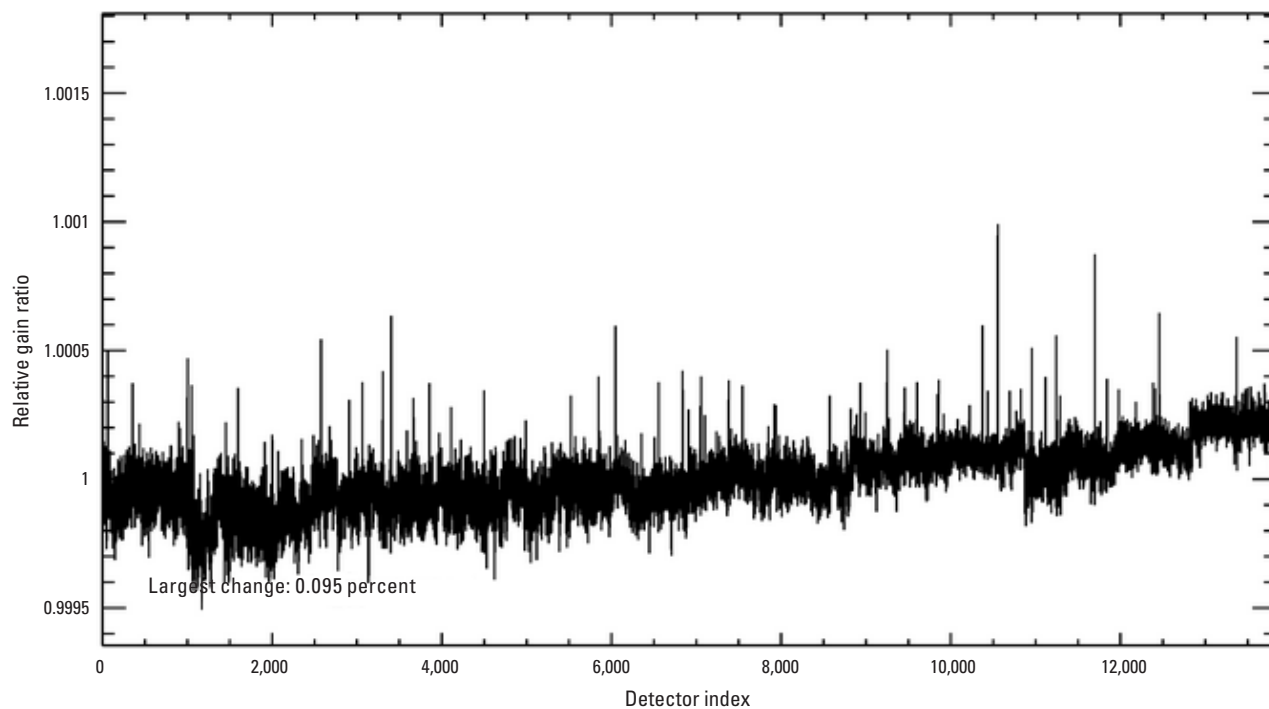
Figure 27. Graph showing Landsat 9 Operational Land Imager panchromatic band per-detector change in relative gains between quarter 1 and quarter 2, 2024.
