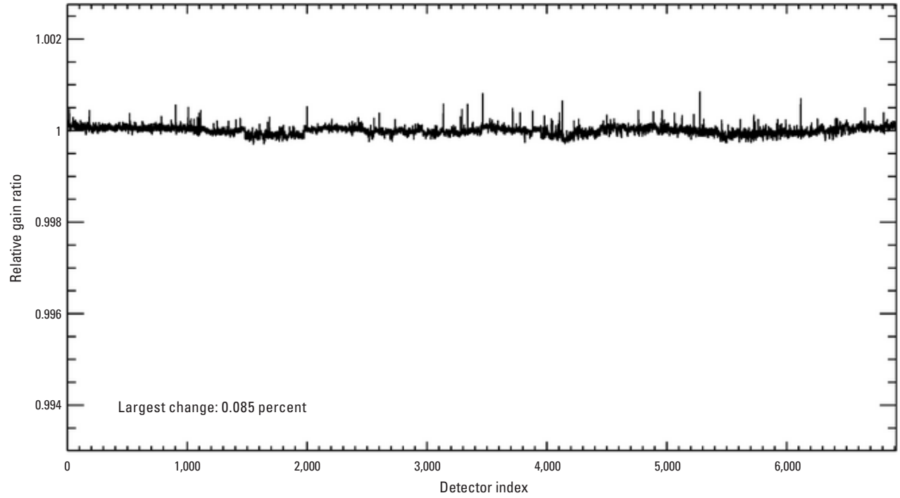
Figure 67. Graph showing Landsat 8 Operational Land Imager coastal/aerosol band per-detector change in relative gains between quarter 1 and quarter 2, 2024.
