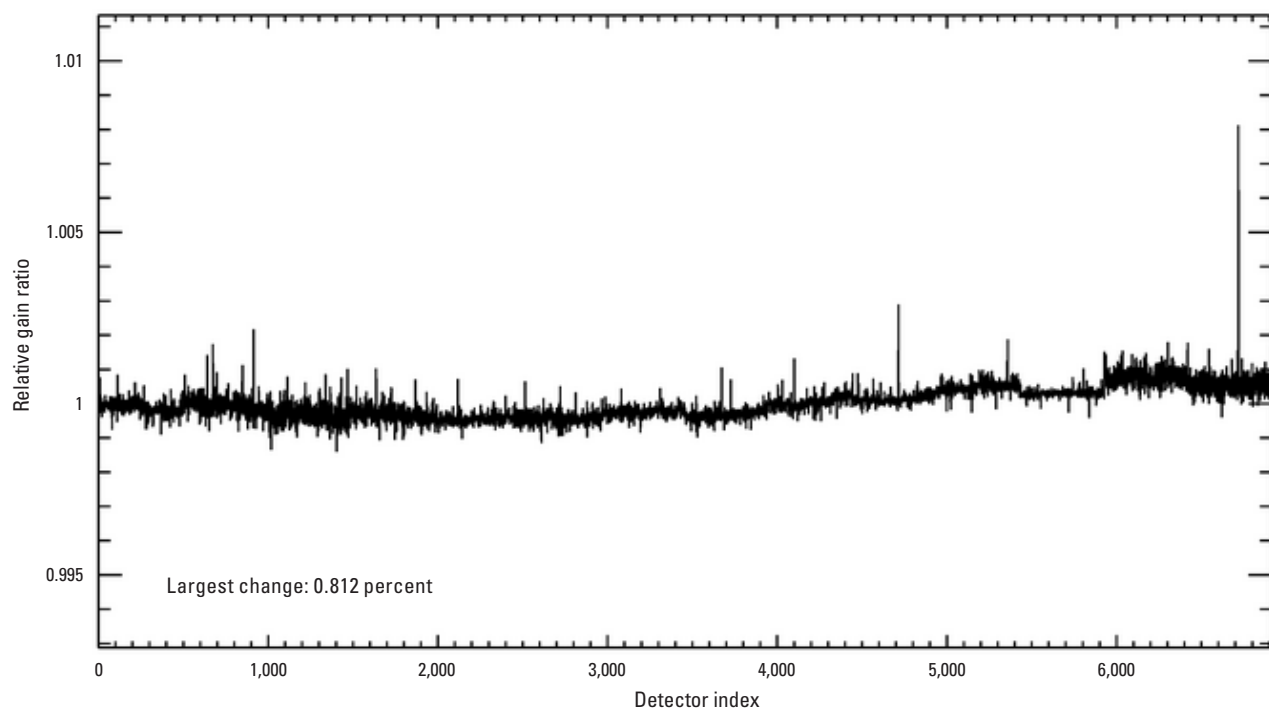
Figure 69. Graph showing Landsat 8 Operational Land Imager shortwave infrared 2 band per-detector change in relative gains between quarter 1 and quarter 2, 2024.
