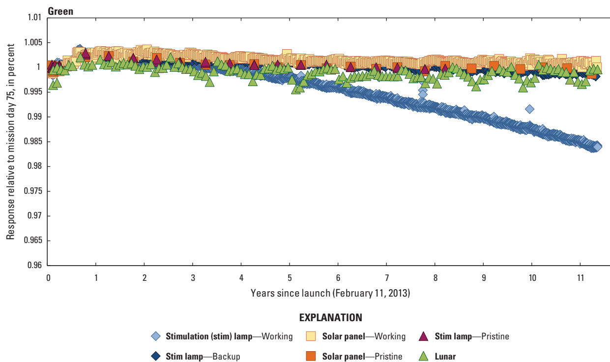
Figure 54. Graph showing Landsat 8 Operational Land Imager green band lifetime radiometric stability.
