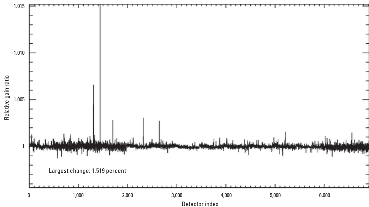
Figure 68. Graph showing Landsat 8 Operational Land Imager shortwave infrared 1 band per-detector change in relative gains between quarter 3 (July–September) and quarter 4 (October–December), 2024.
