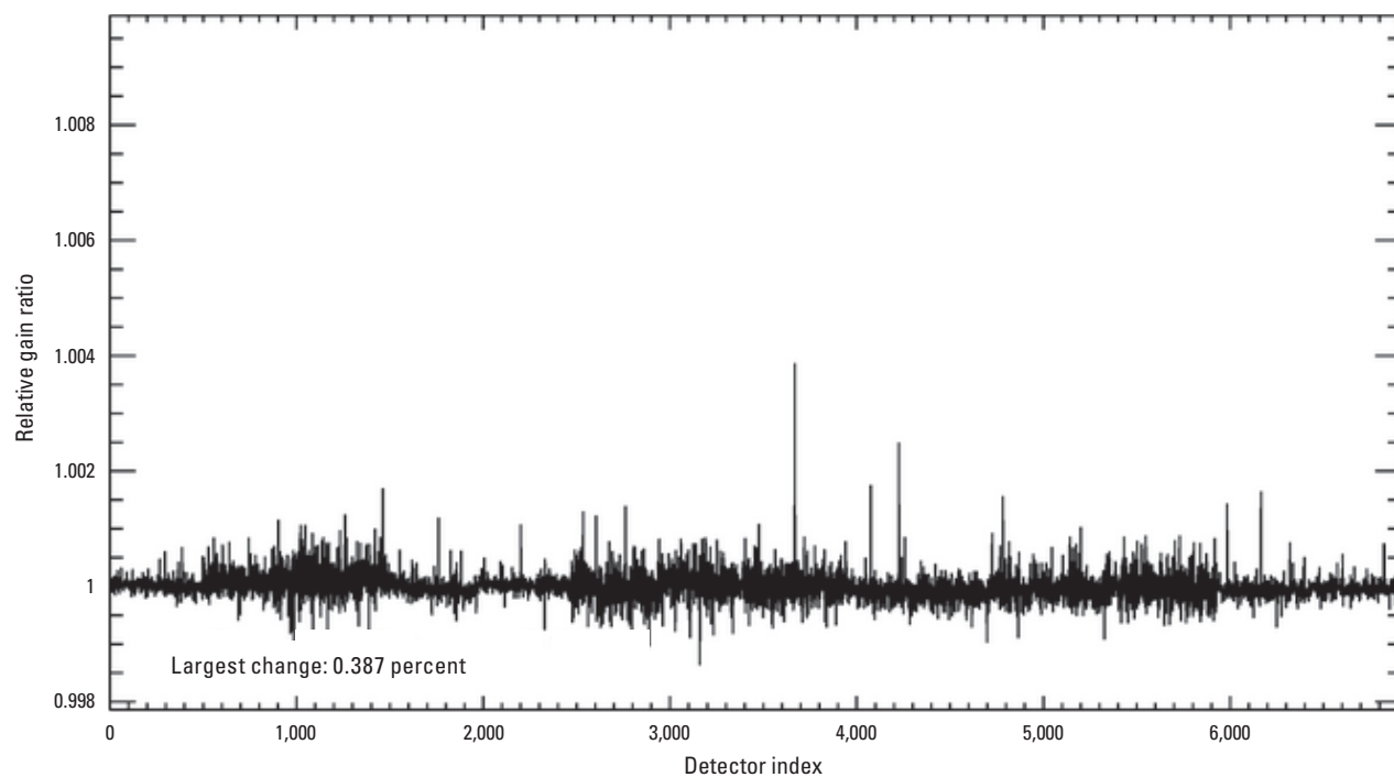
Figure 25. Graph showing Landsat 9 Operational Land Imager shortwave infrared 1 band per-detector change in relative gains between quarter 3 (July–September) and quarter 4 (October–December), 2024.
