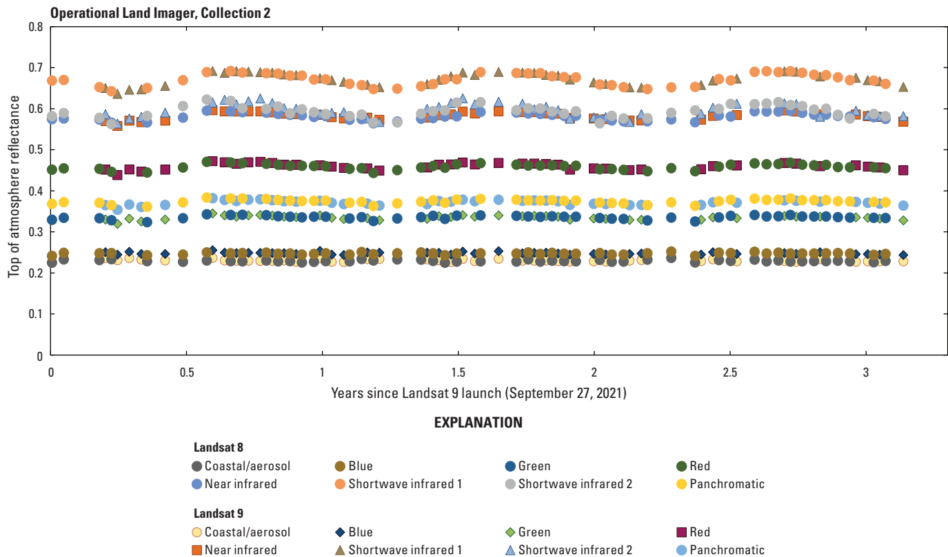
Figure 30. Graph showing Landsat 9 to Landsat 8 Operational Land Imager Libya 4 pseudoinvariant calibration site top of atmosphere reflectance cross-correlation.
