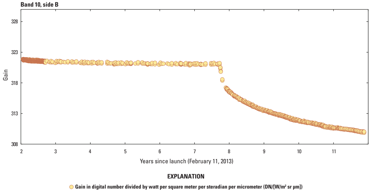
Figure 63. Graph showing Landsat 8 Thermal Infrared Sensor band 10 radiometric stability (side B).
