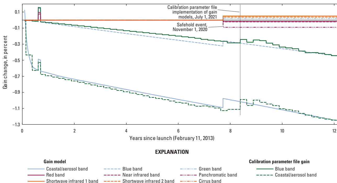
Figure 65. Graph showing Landsat 8 Operational Land Imager lifetime gain trends and calibration gain updates.
