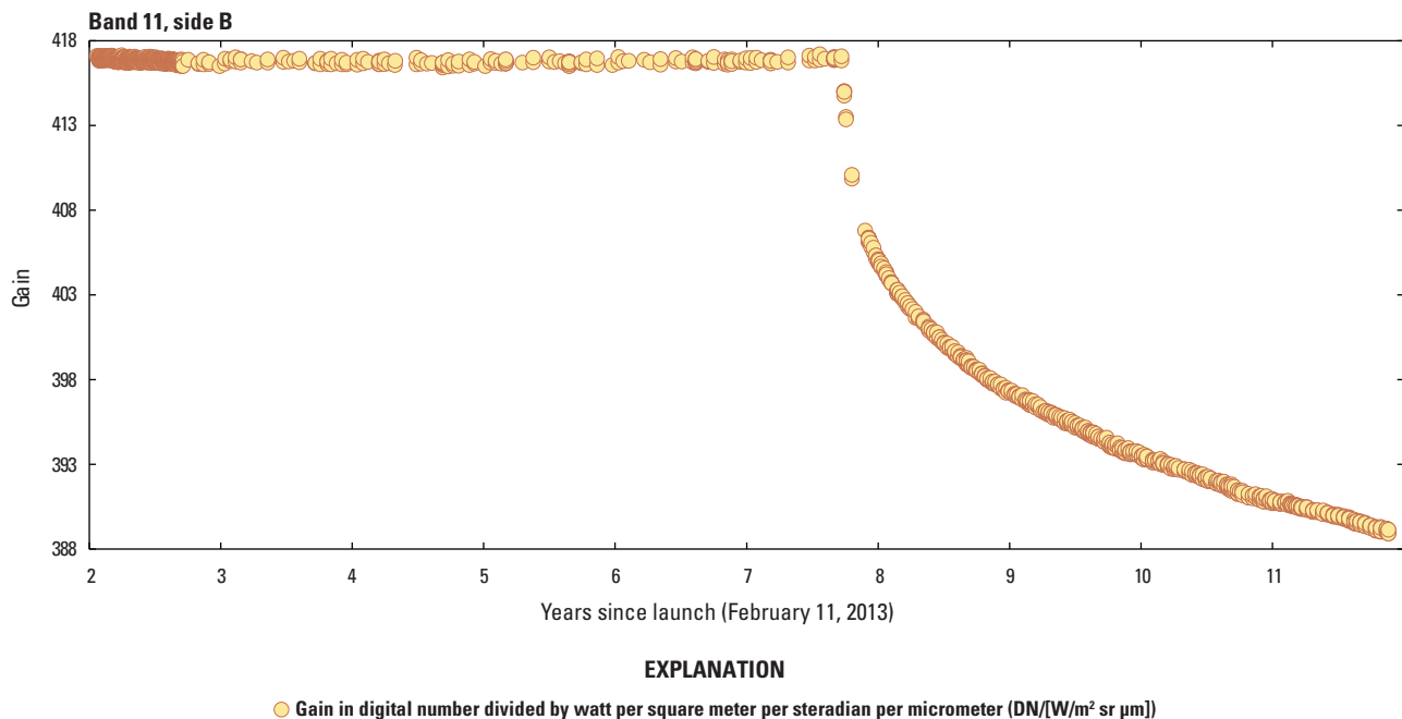
Figure 64. Graph showing Landsat 8 Thermal Infrared Sensor band 11 radiometric stability (side B).
