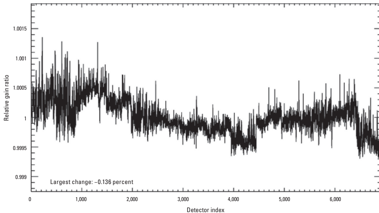
Figure 24. Graph showing Landsat 9 Operational Land Imager coastal/aerosol band per-detector change in relative gains between quarter 3 (July–September) and quarter 4 (October–December), 2024.
