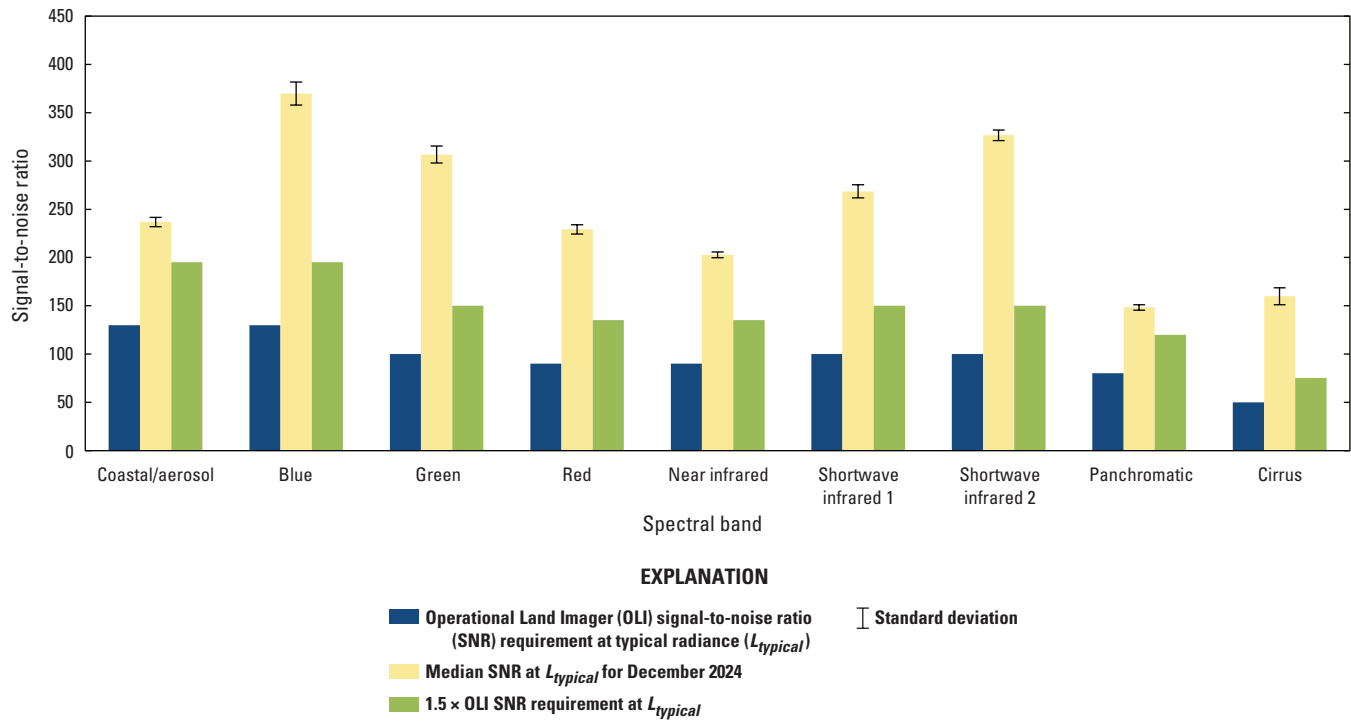
Figure 40. Graph showing Landsat 8 Operational Land Imager signal-to-noise ratio performance, December 2024.
