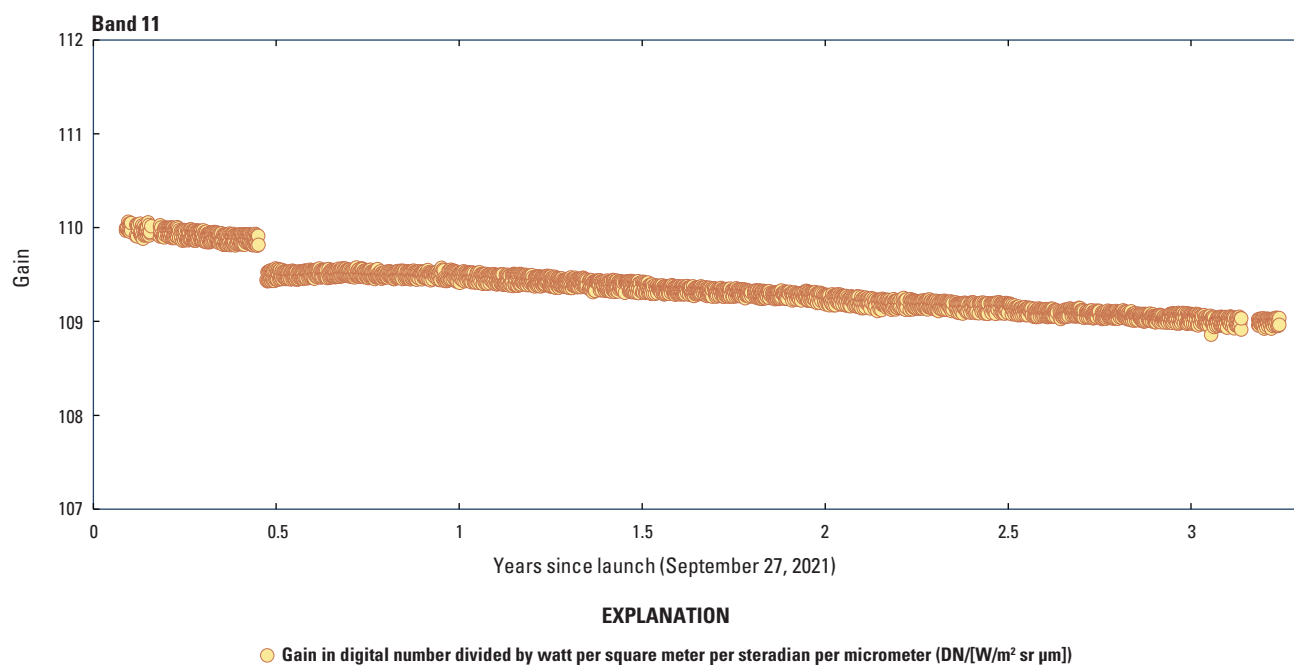
Figure 23. Graph showing Landsat 9 Thermal Infrared Sensor band 11 radiometric stability.
