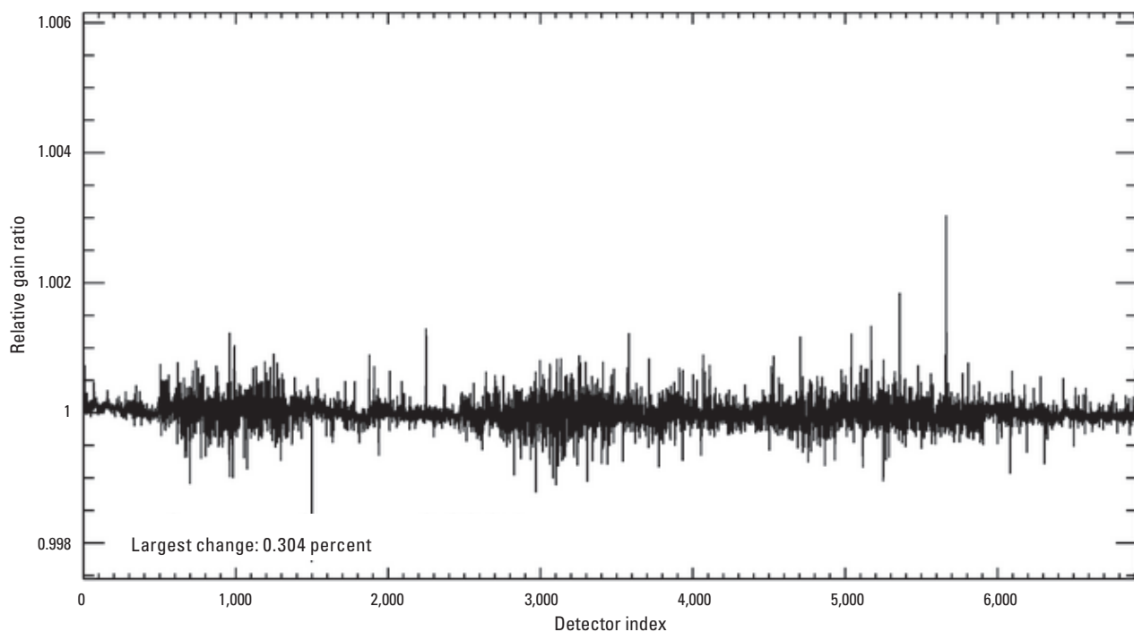
Figure 26. Graph showing Landsat 9 Operational Land Imager shortwave infrared 2 band per-detector change in relative gains between quarter 3 (July–September) and quarter 4 (October–December), 2024.
