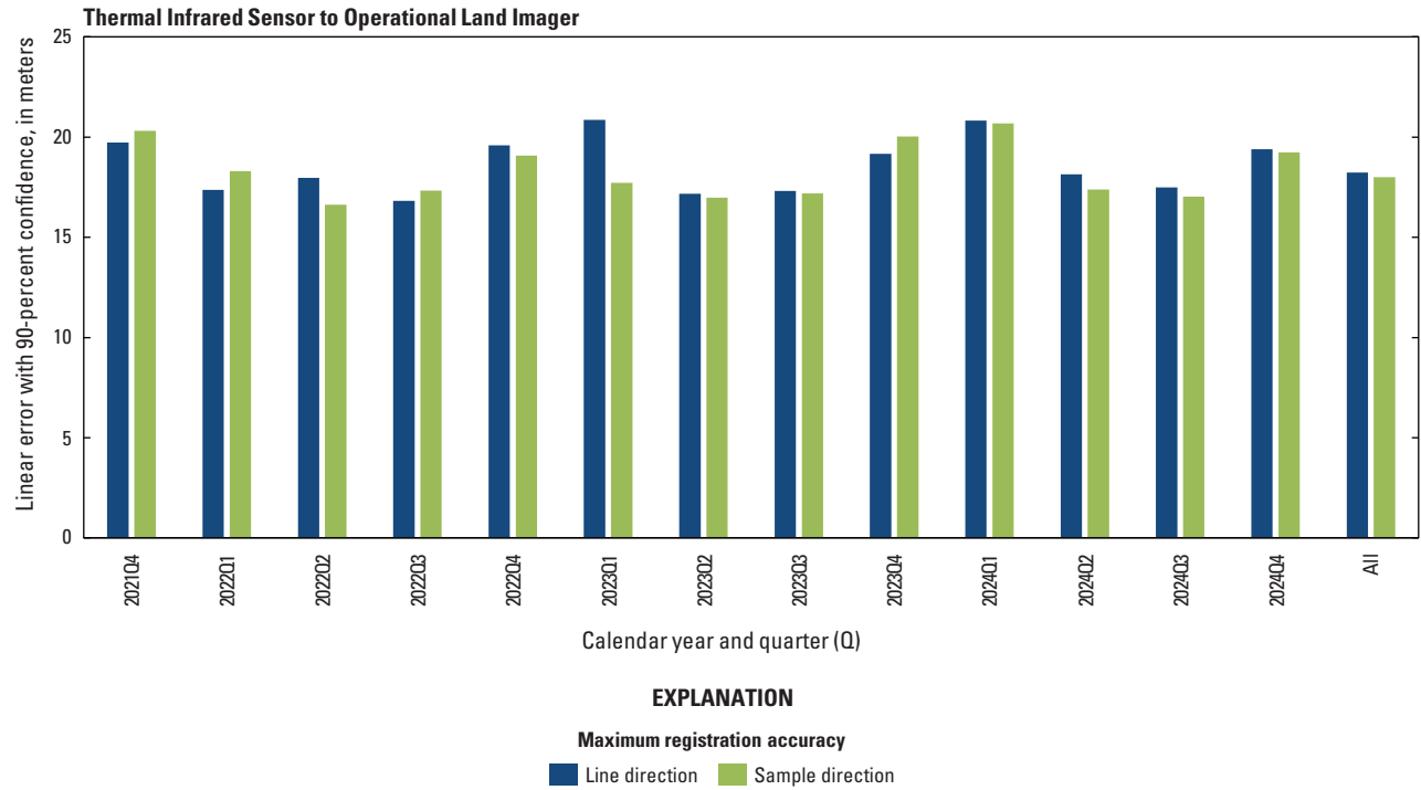
Figure 33. Graph showing Landsat 9 Thermal Infrared Sensor to Operational Land Imager lifetime band (excluding cirrus) registration accuracy by quarter.
