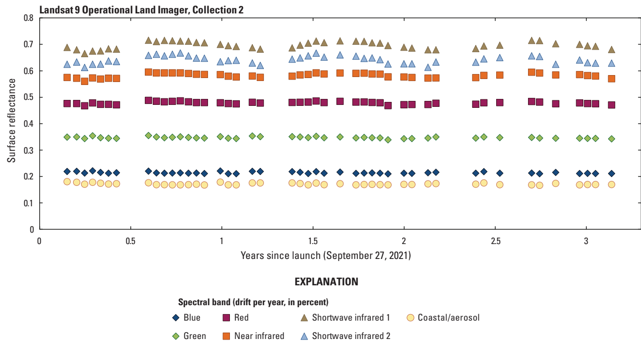
Figure 82. Graph showing Libya 4 pseudoinvariant calibration site surface reflectance trending, Landsat 9 Operational Land Imager, Collection 2.
