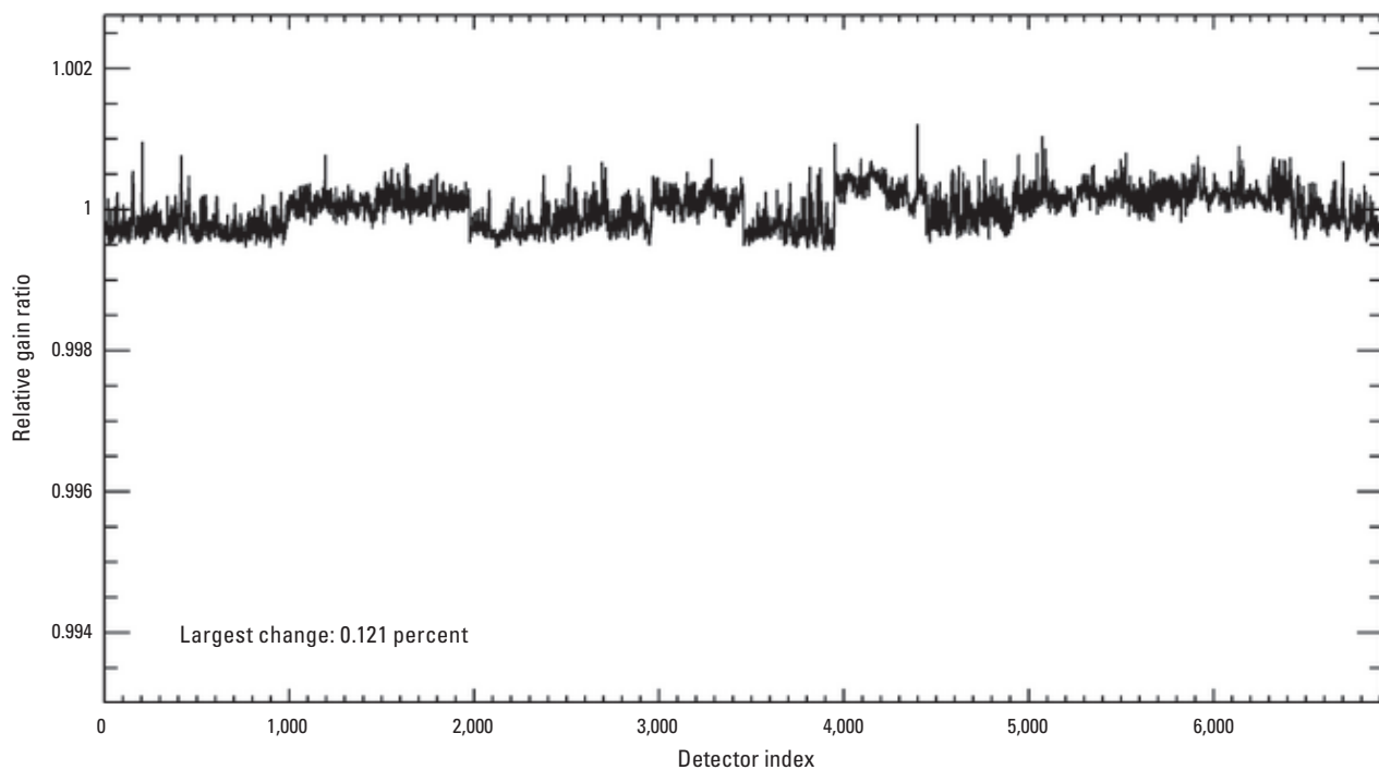
Figure 67. Graph showing Landsat 8 Operational Land Imager coastal/aerosol band per-detector change in relative gains between quarter 3 (July–September) and quarter 4 (October–December), 2024.
