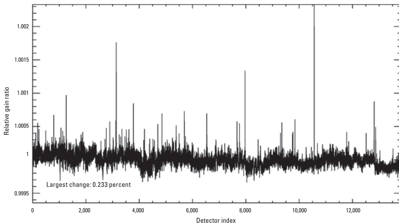
Figure 27. Graph showing Landsat 9 Operational Land Imager panchromatic band per-detector change in relative gains between quarter 3 (July–September) and quarter 4 (October–December), 2024.
