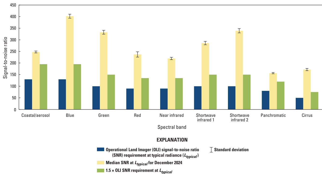
Figure 1. Graph showing Landsat 9 Operational Land Imager signal-to-noise ratio performance, December 2024.
