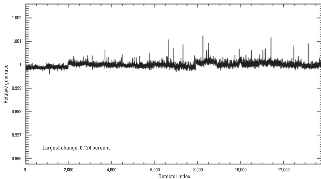
Figure 70. Graph showing Landsat 8 Operational Land Imager panchromatic band per-detector change in relative gains between quarter 3 (July–September) and quarter 4 (October–December), 2024.
