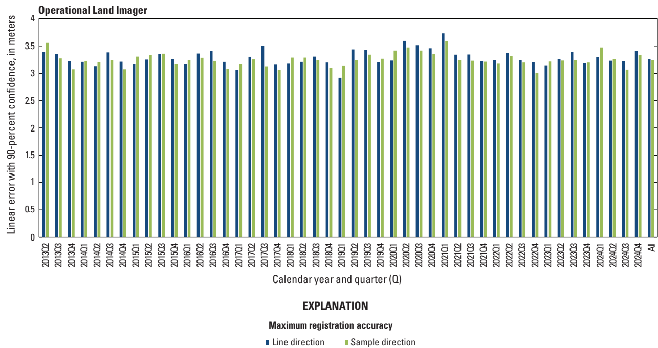
Figure 73. Graph showing Landsat 8 Operational Land Imager lifetime band (excluding cirrus) registration accuracy by quarter.
