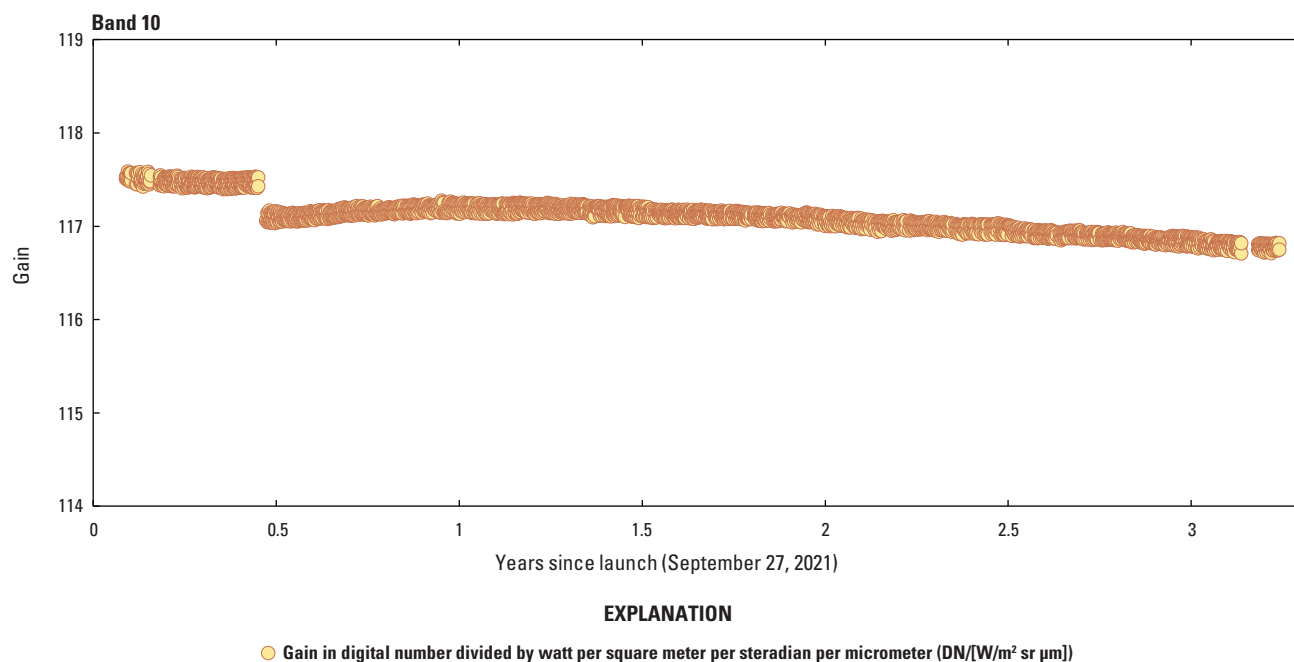
Figure 22. Graph showing Landsat 9 Thermal Infrared Sensor band 10 radiometric stability.
