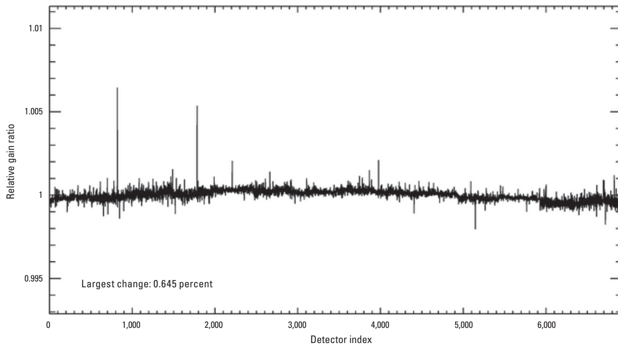
Figure 69. Graph showing Landsat 8 Operational Land Imager shortwave infrared 2 band per-detector change in relative gains between quarter 3 (July–September) and quarter 4 (October–December), 2024.
