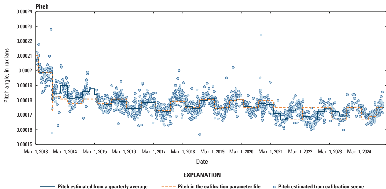
Figure 76. Graph showing Landsat 8 Thermal Infrared Sensor to Operational Land Imager lifetime pitch alignment.
