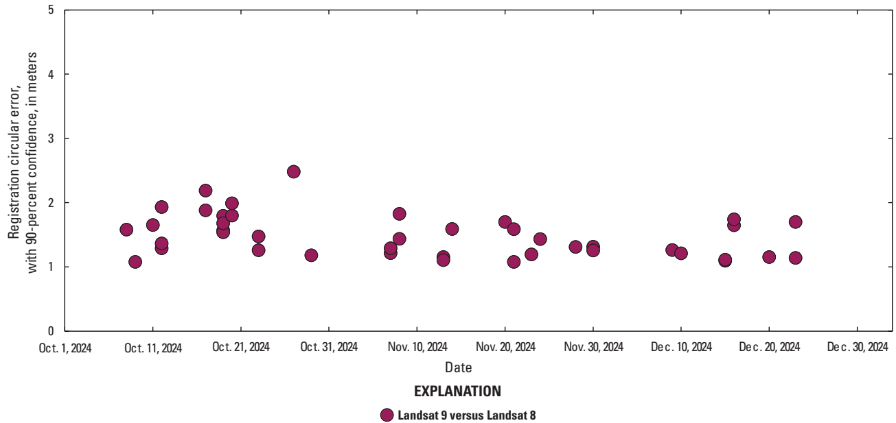
Figure 39. Graph showing coregistration error between Landsat 9 and Landsat 8 Level 1 terrain-corrected products, quarter 4 (October–December), 2024.
