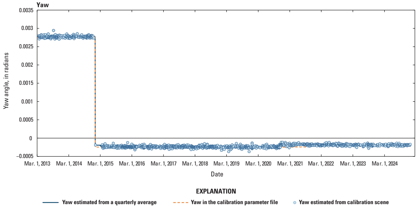
Figure 78. Graph showing Landsat 8 Thermal Infrared Sensor to Operational Land Imager lifetime yaw alignment.
