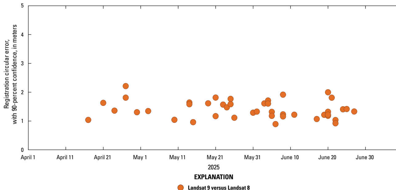
Figure 39. Graph showing coregistration error between Landsat 9 and Landsat 8 Level 1 terrain-corrected products, quarter 2, 2025.
