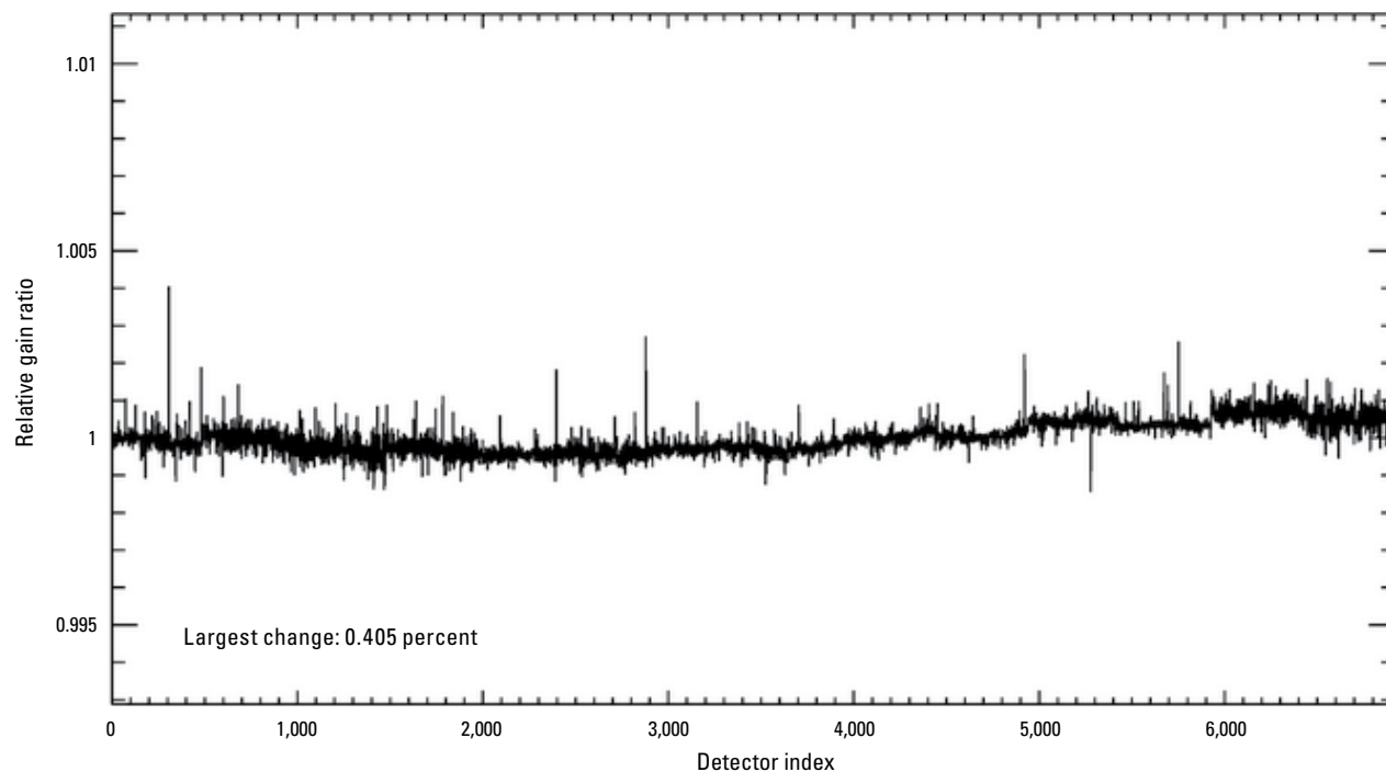
Figure 69. Graph showing Landsat 8 Operational Land Imager shortwave infrared 2 band per-detector change in relative gains between quarter 1 (January–March) and quarter 2 (April–June), 2025.
