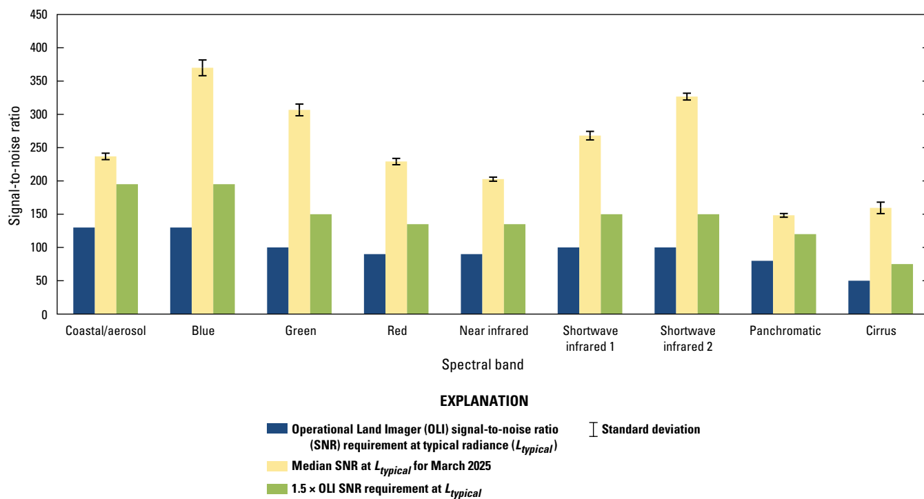
Figure 40. Graph showing Landsat 8 Operational Land Imager signal-to-noise ratio performance, June 2025.
