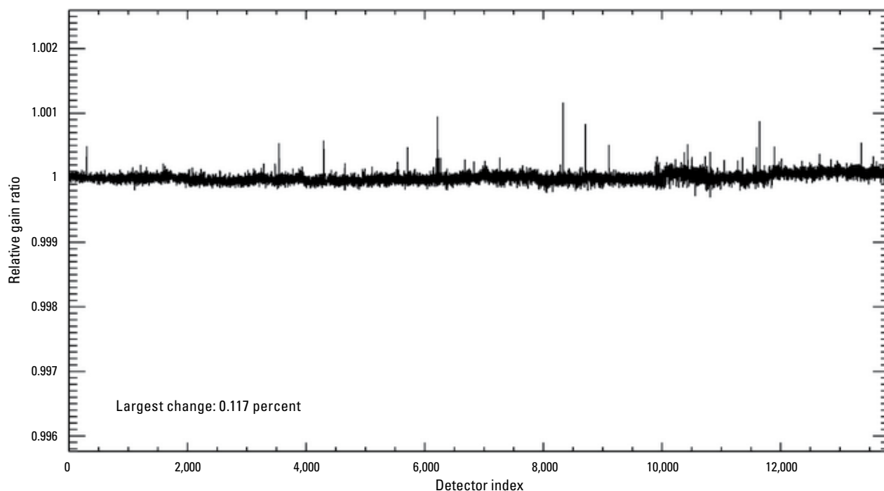
Figure 70. Graph showing Landsat 8 Operational Land Imager panchromatic band per-detector change in relative gains between quarter 1 (January–March) and quarter 2 (April–June), 2025.
