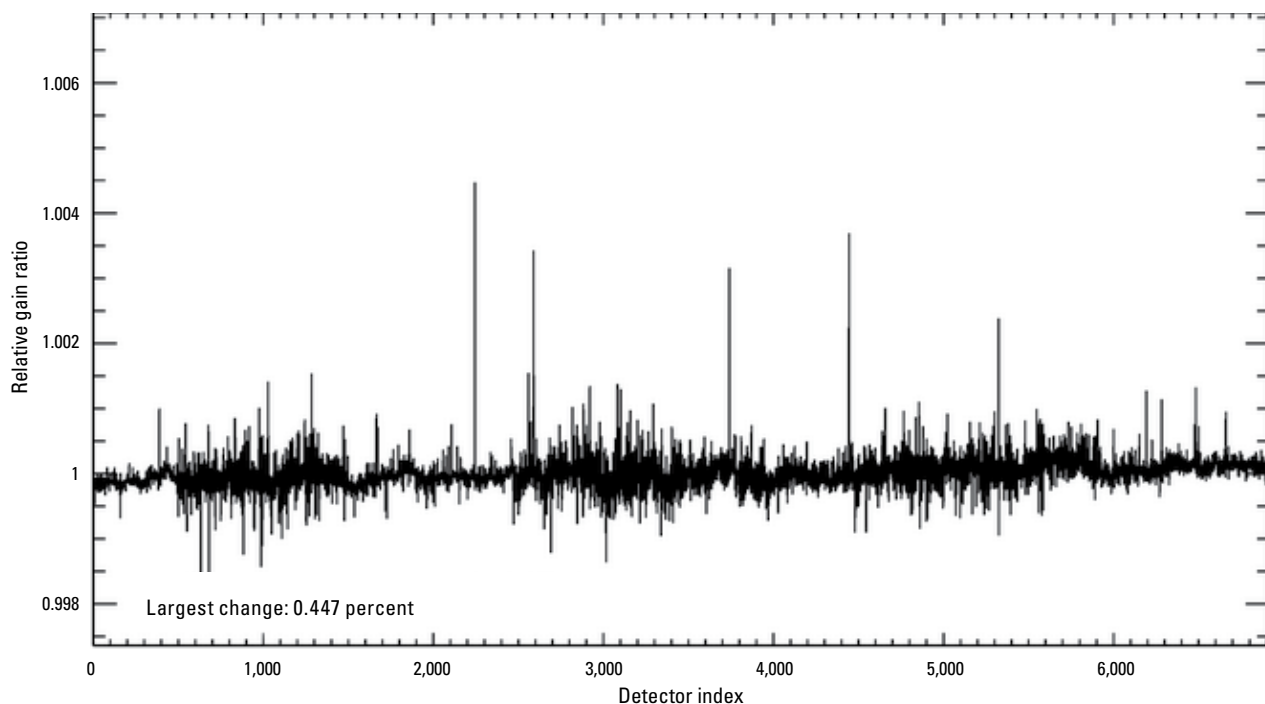
Figure 26. Graph showing Landsat 9 Operational Land Imager shortwave infrared 2 band per-detector change in relative gains between quarter 1 (January–March) and quarter 2 (April–June), 2025.
