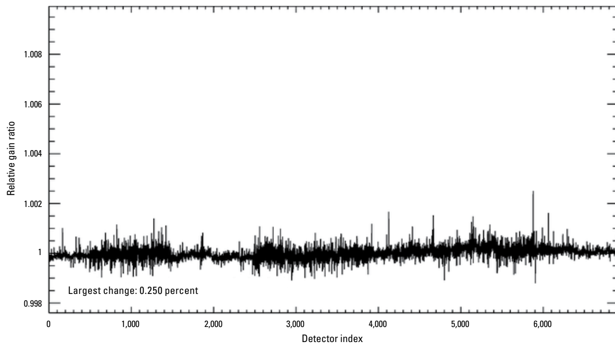
Figure 25. Graph showing Landsat 9 Operational Land Imager shortwave infrared 1 band per-detector change in relative gains between quarter 1 (January–March) and quarter 2 (April–June), 2025.
