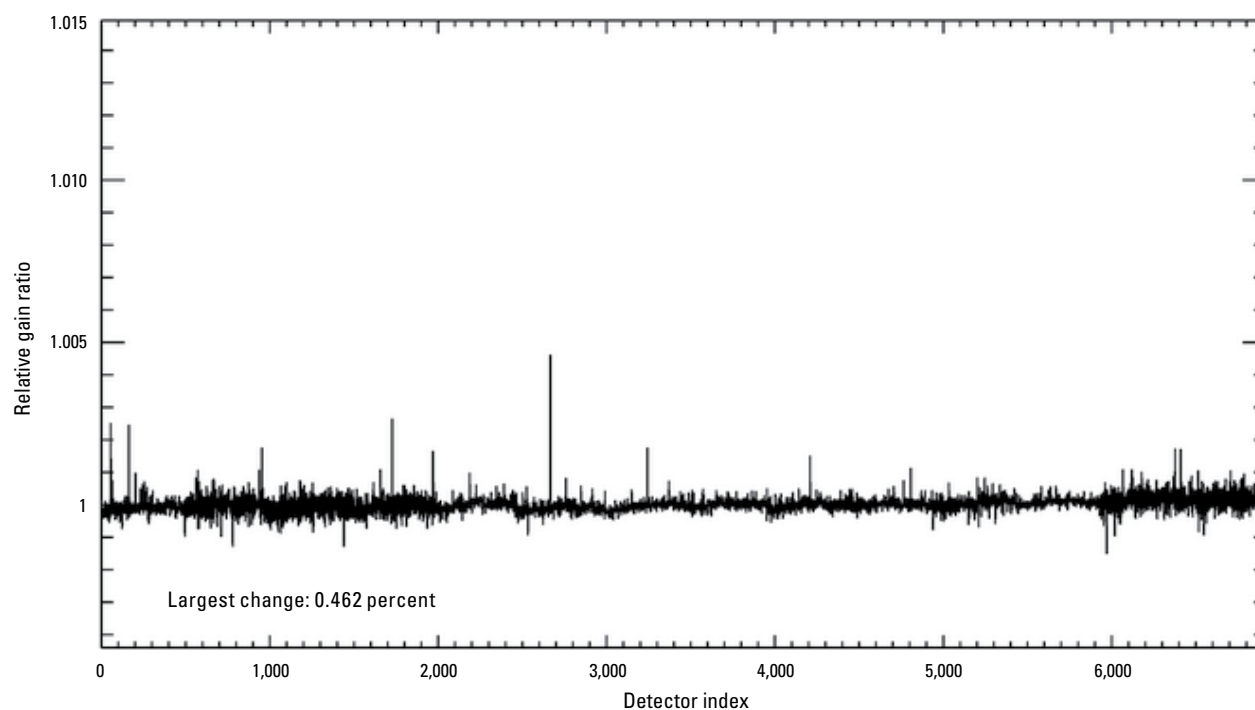
Figure 68. Graph showing Landsat 8 Operational Land Imager shortwave infrared 1 band per-detector change in relative gains between quarter 1 (January–March) and quarter 2 (April–June), 2025.
