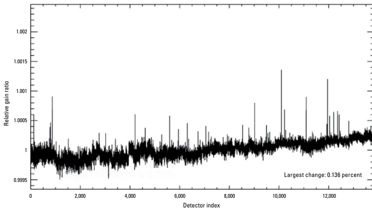
Figure 27. Graph showing Landsat 9 Operational Land Imager panchromatic band per-detector change in relative gains between quarter 1 (January–March) and quarter 2 (April–June), 2025.
