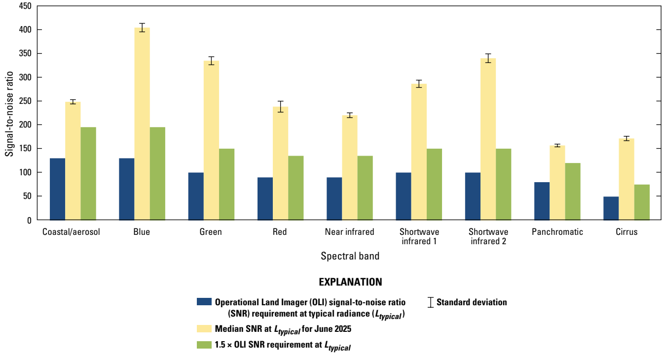
Figure 1. Graph showing Landsat 9 Operational Land Imager signal-to-noise ratio performance, June 2025.
