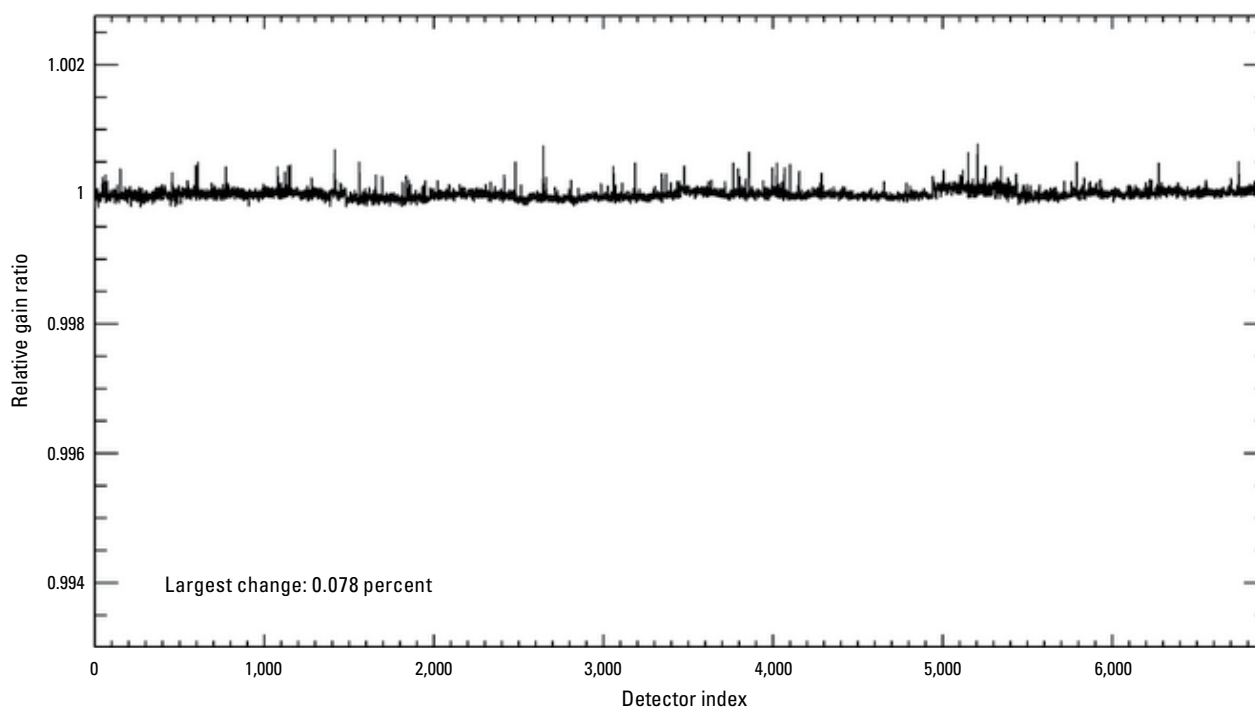
Figure 67. Graph showing Landsat 8 Operational Land Imager coastal/aerosol band per-detector change in relative gains between quarter 1 (January–March) and quarter 2 (April–June), 2025.
