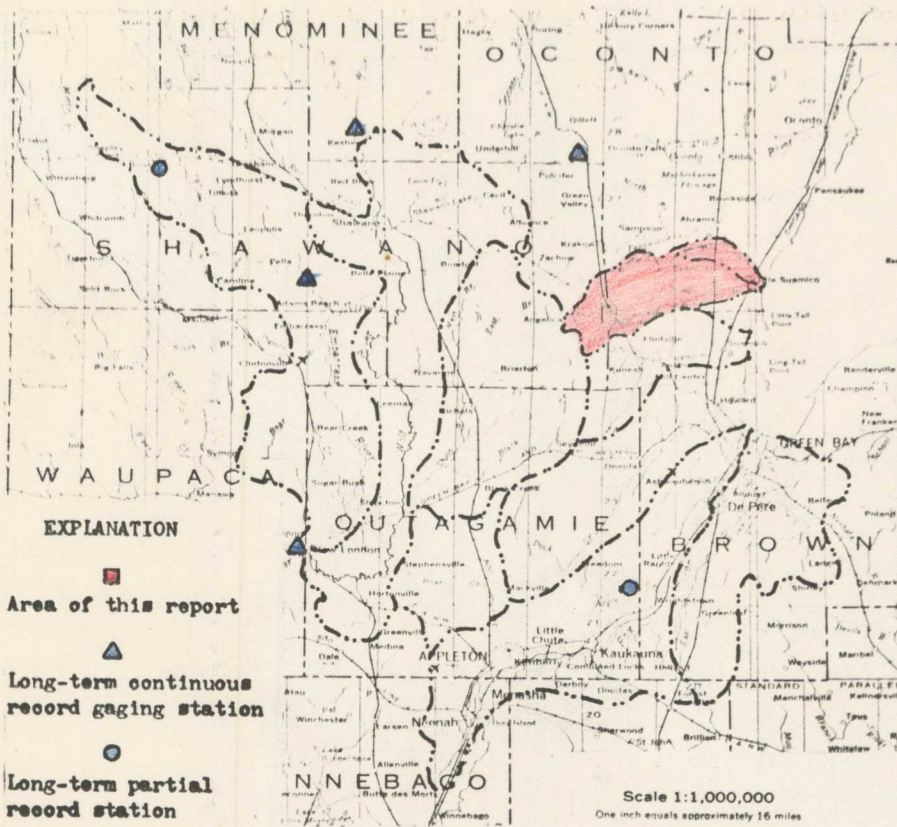
Figure 1.--Index map of basins studied in the Green Bay area, Wisconsin.
