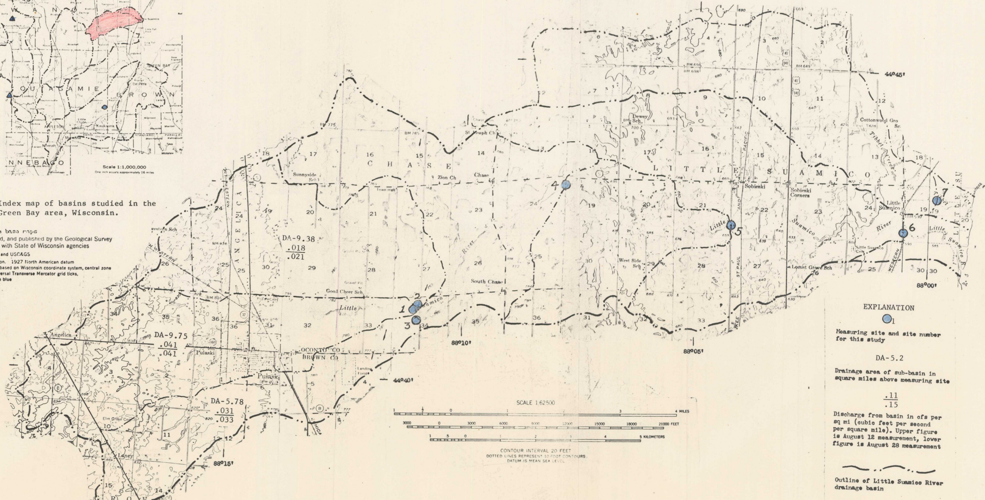
Figure 2.--Map of the Little Suamico River basin, Oconto, Brown, and Shawano Counties, Wisconsin, showing locations of stream gaging sites.
