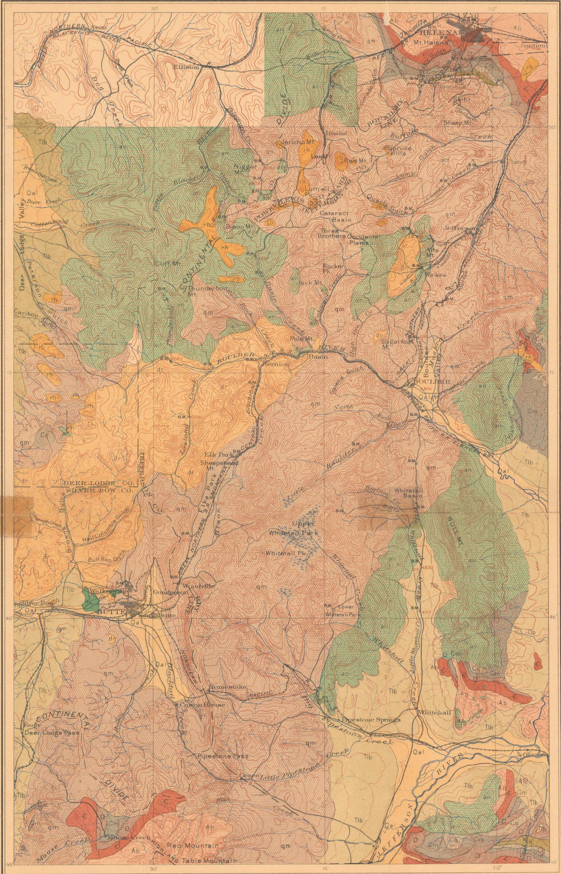
GEOLOGIC MAP OF REGION SURROUNDING THE BUTTE DISTRICT
