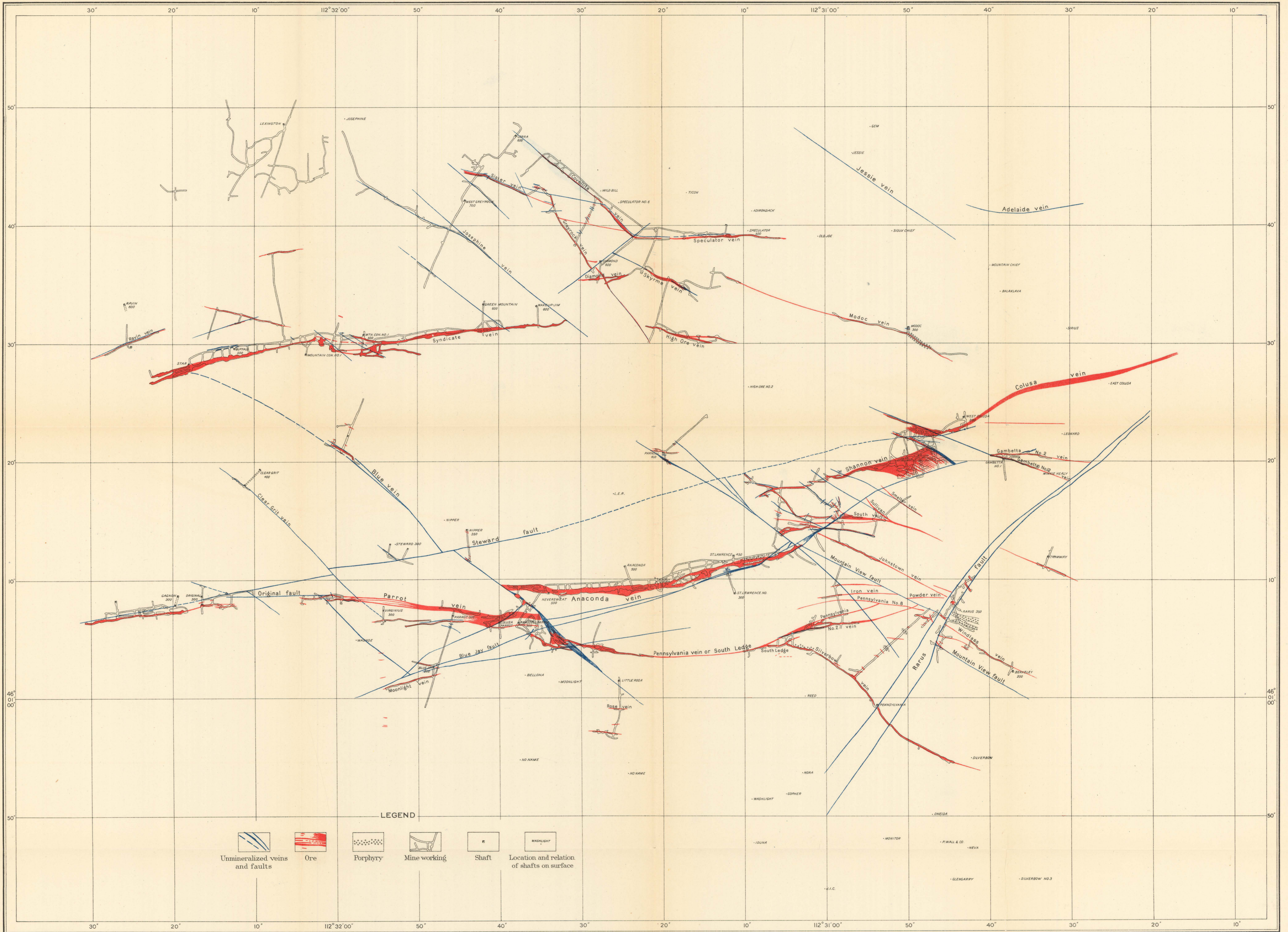
MAP SHOWING KNOWN VEIN STRUCTURE ON 5600-FOOT PLANE ABOVE SEA LEVEL
