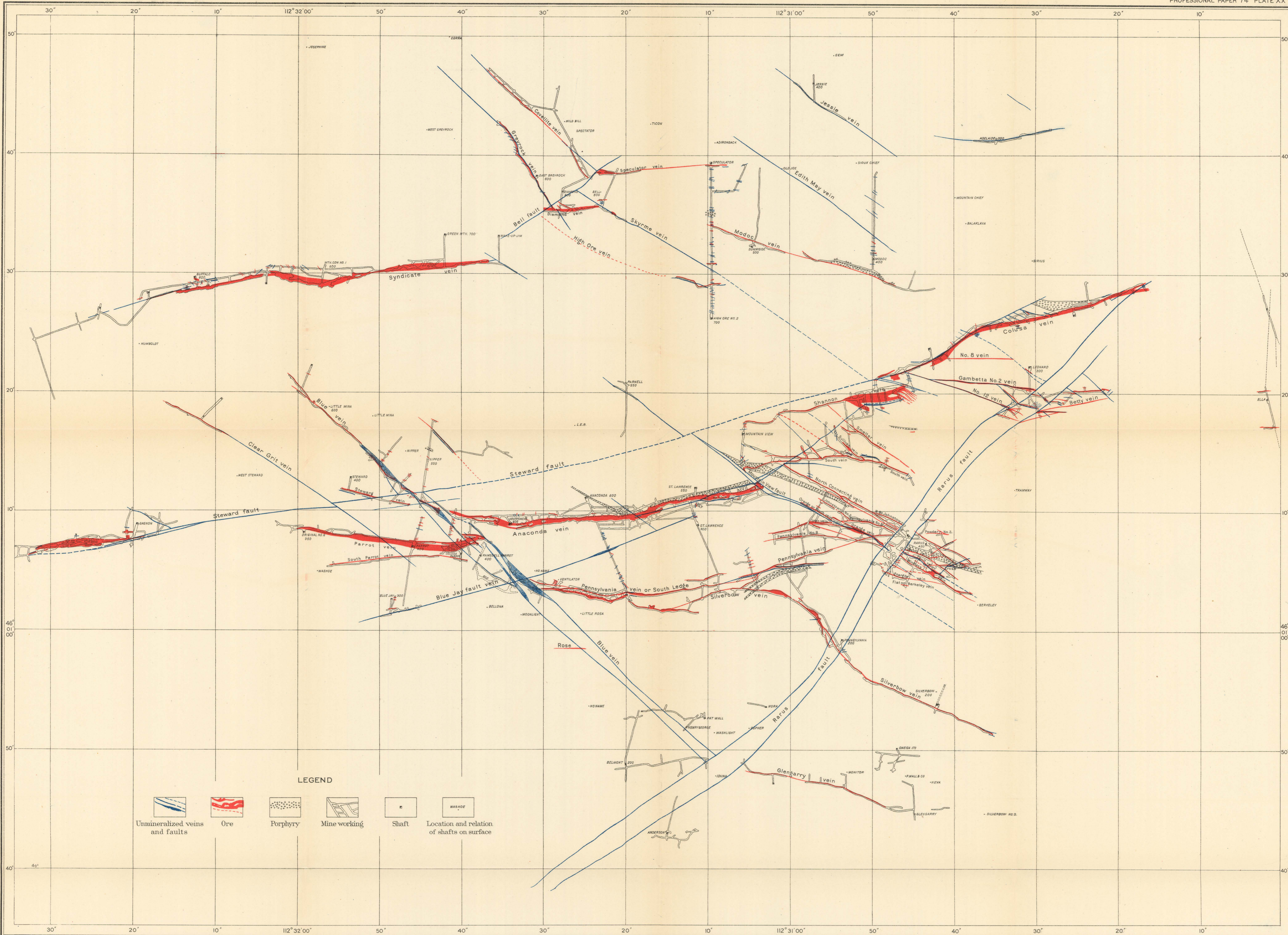
MAP SHOWING KNOWN VEIN STRUCTURE ON 5500-FOOT PLANE ABOVE SEA LEVEL
