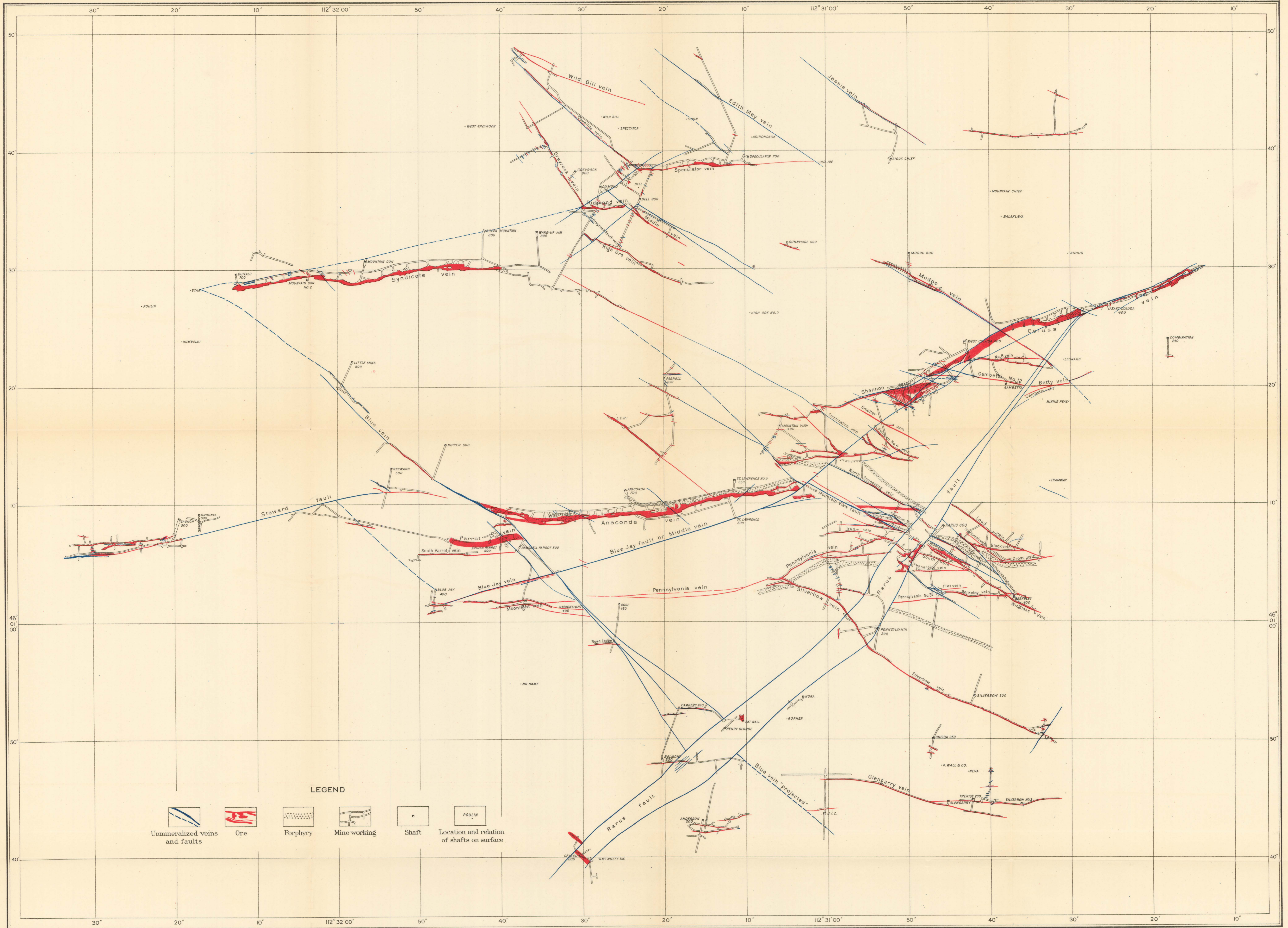
MAP SHOWING KNOWN VEIN STRUCTURE ON 5400-FOOT PLANE ABOVE SEA LEVEL
