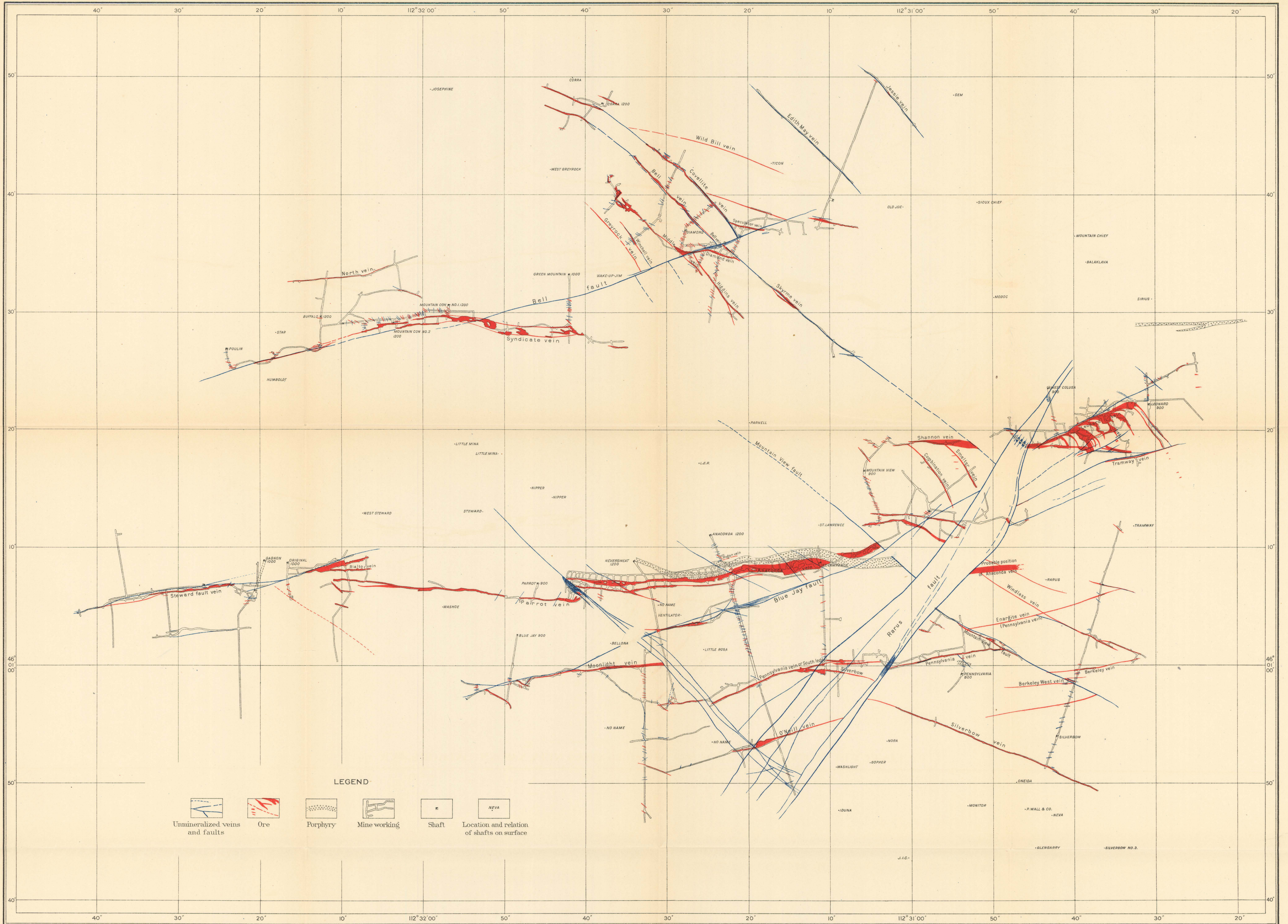
MAP SHOWING KNOWN VEIN STRUCTURE ON 4900-FOOT PLANE ABOVE SEA LEVEL
