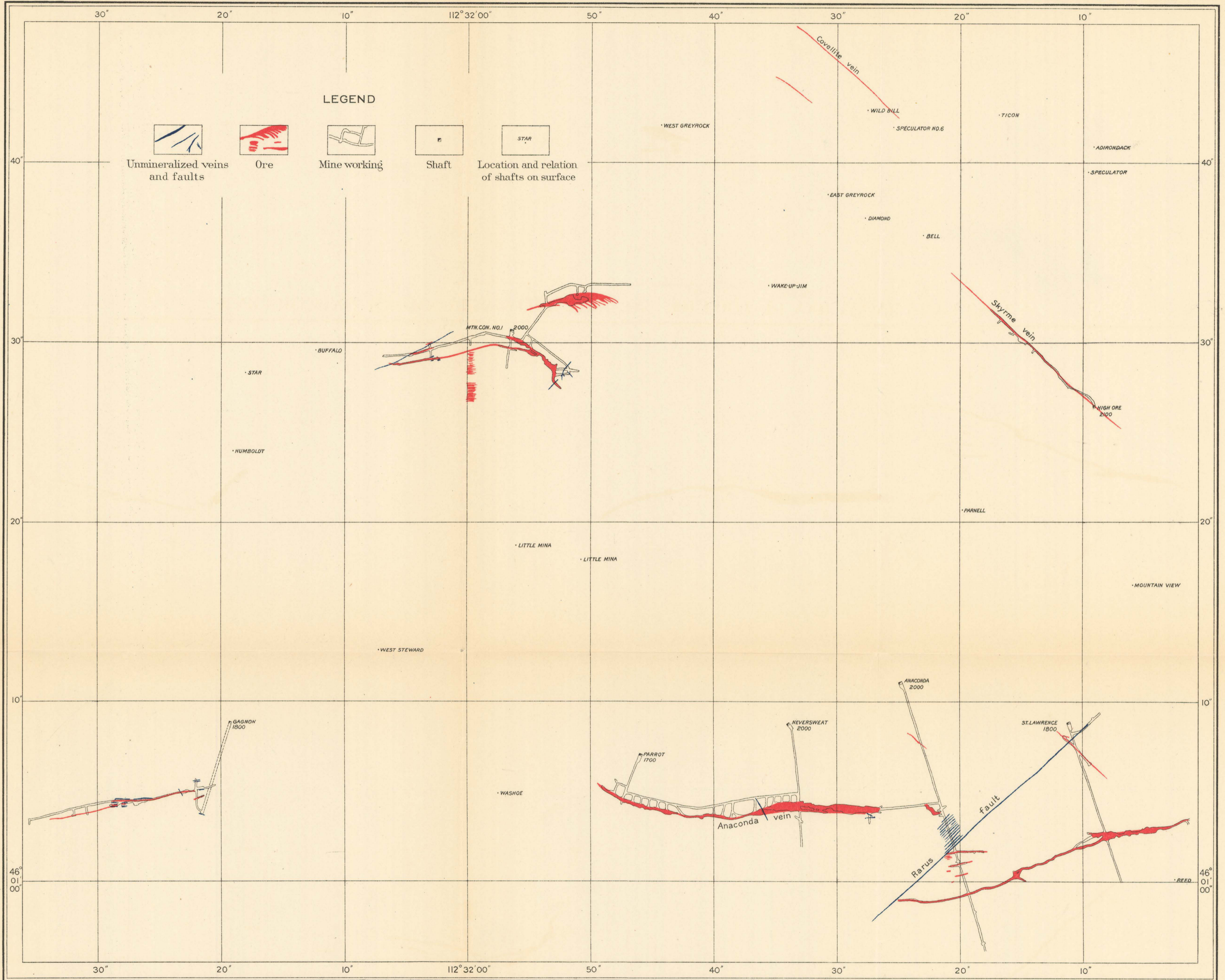
MAP SHOWING KNOWN VEIN STRUCTURE ON 4100-FOOT PLANE ABOVE SEA LEVEL
