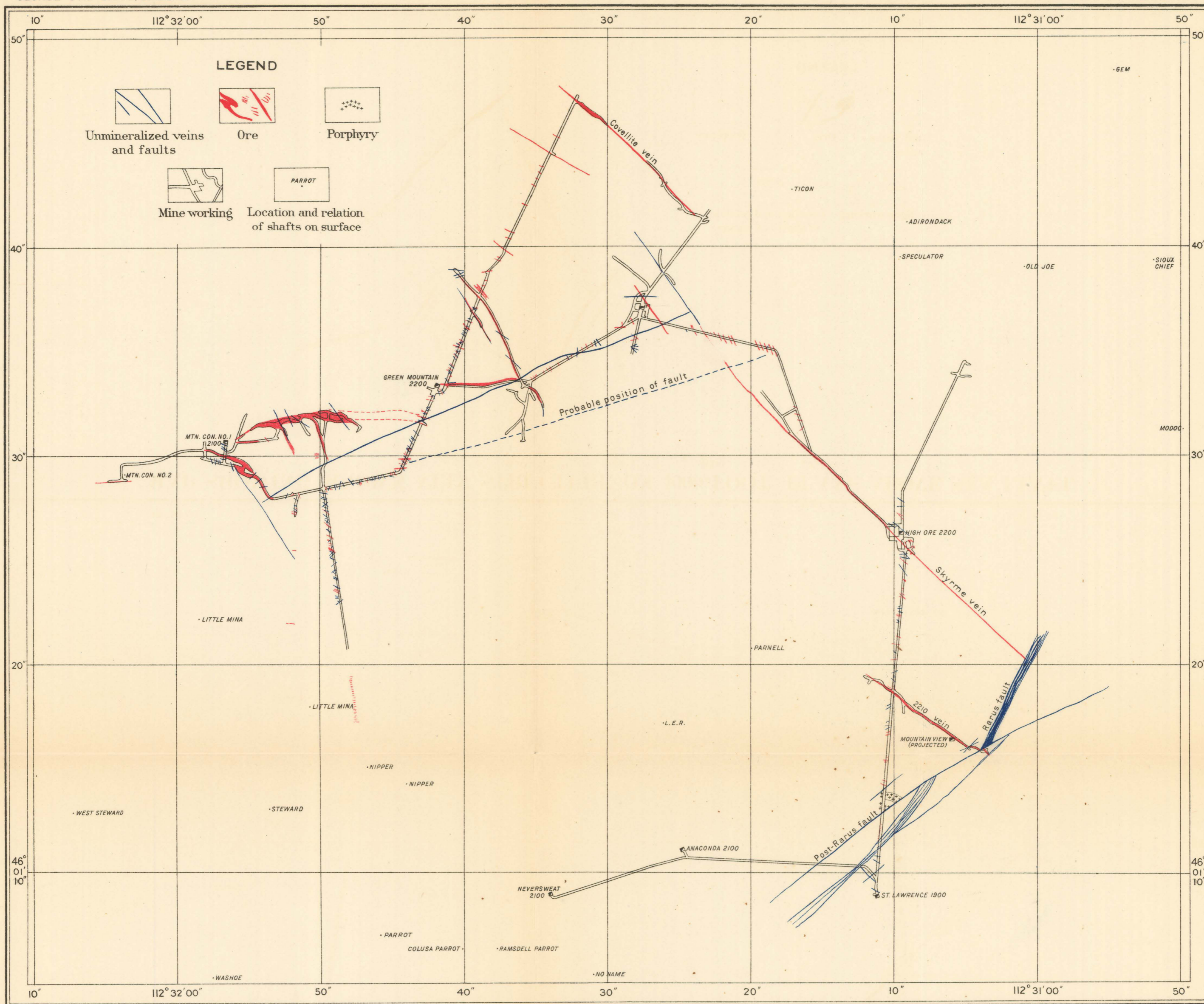
MAP SHOWING KNOWN VEIN STRUCTURE ON 4000-FOOT PLANE ABOVE SEA LEVEL
