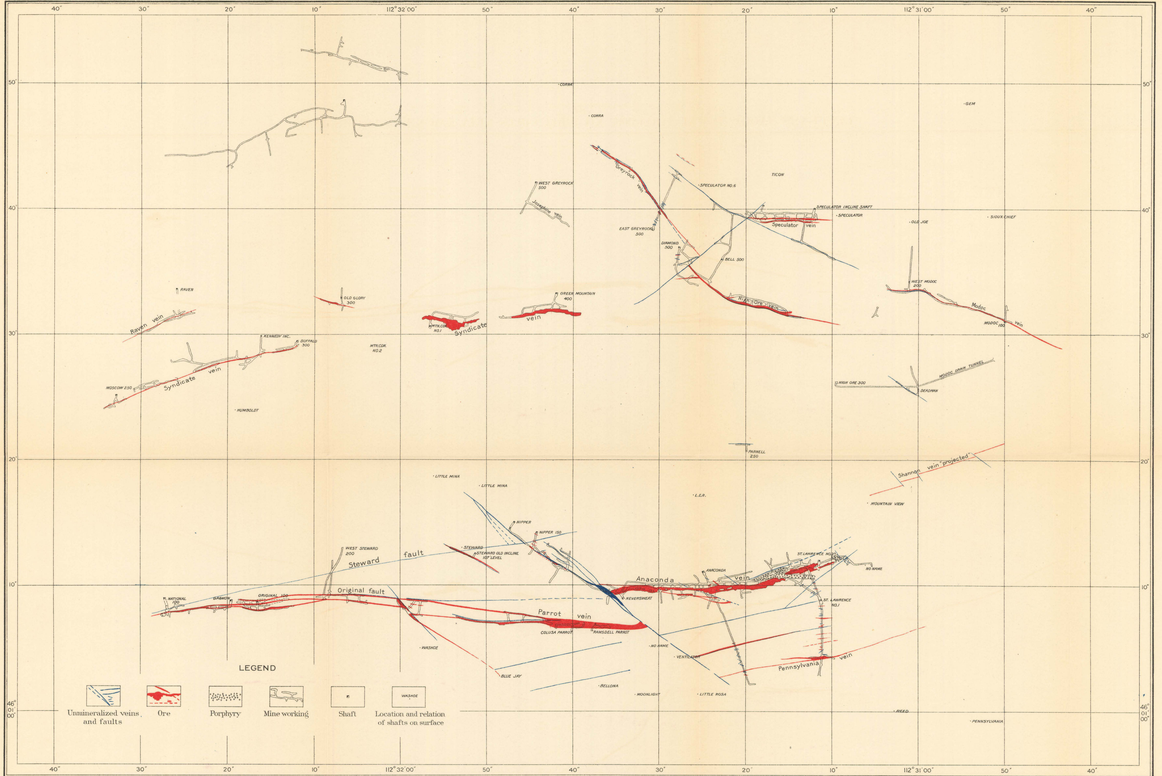
MAP SHOWING KNOWN VEIN STRUCTURE ON 5800-FOOT PLANE ABOVE SEA LEVEL
